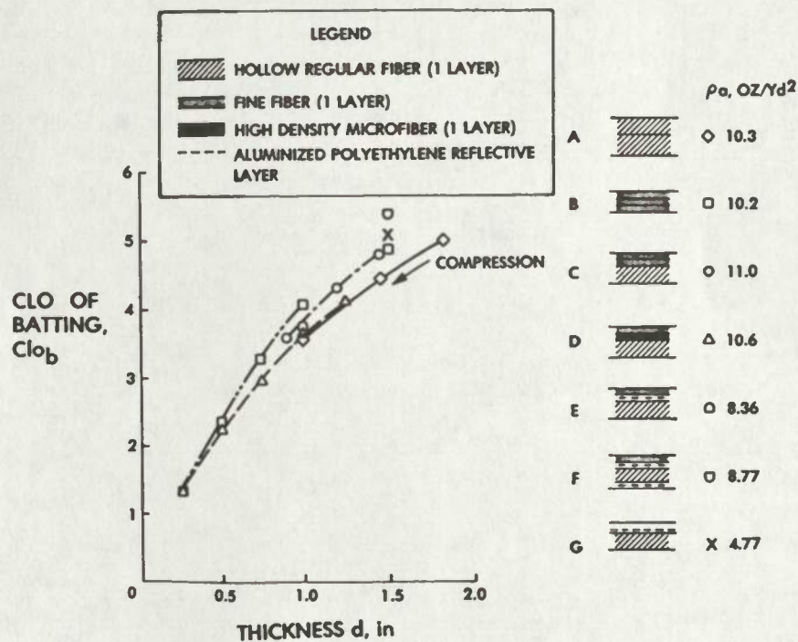
Figure 16. Performance of 10 oz/yd 2 composite and reflective battings.
