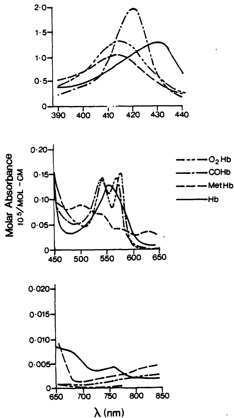
FIGURE 1 Spectra for the Major Haemoglobin Species
