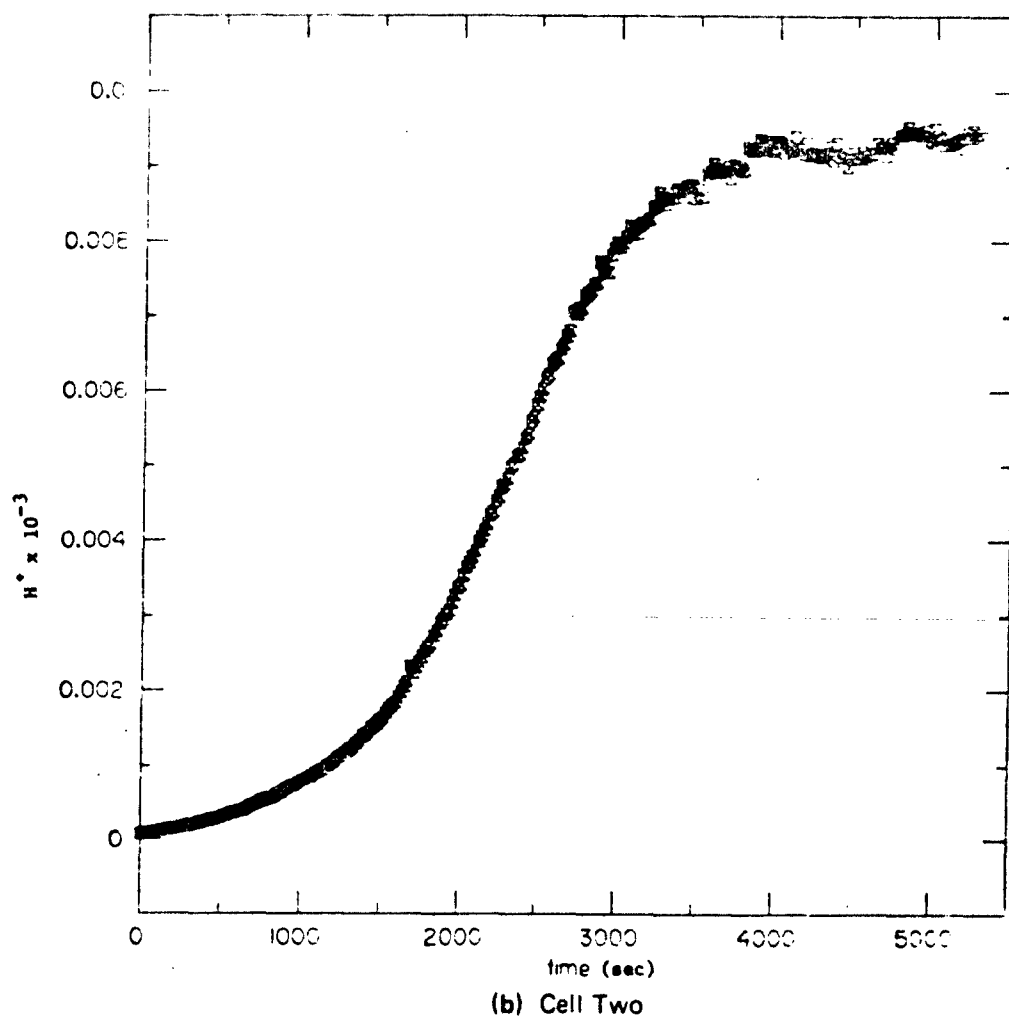
Figure A-3. Plot of Hydrolysis Data for Mustard at 20°C. (Concluded)
