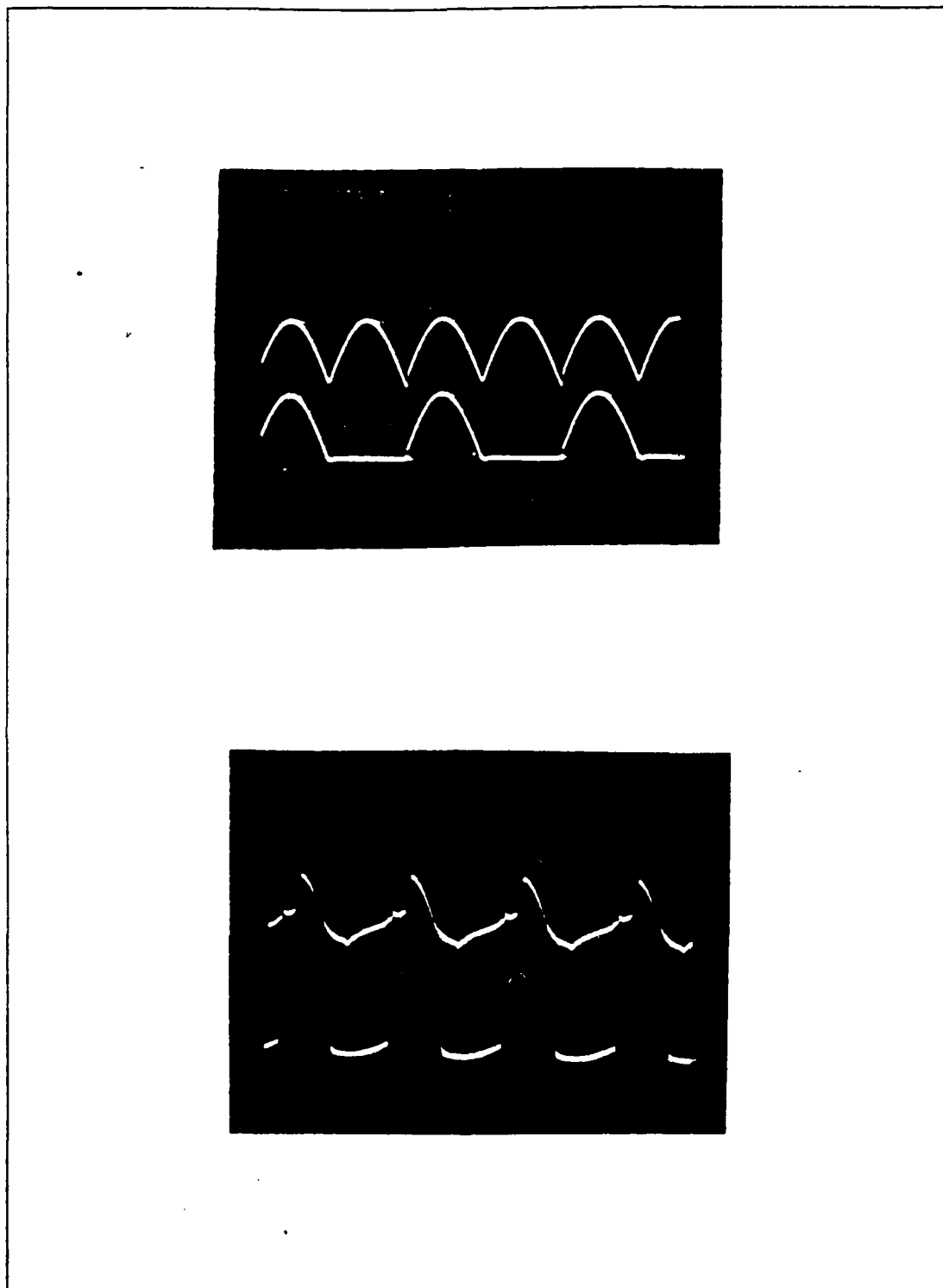
Figure 4.8 (a) Output of Figure 4.6 c for 5 KHz Input (b) Output for Figure 4.6 c for 15 KHz Input
