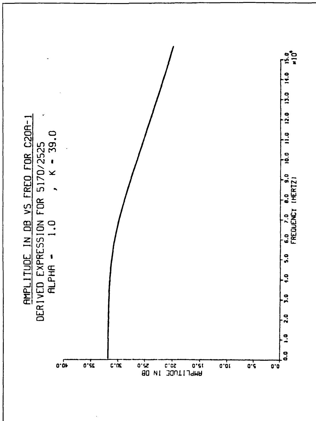
Figure 2.14 Computer Generated Frequency Response of C20A-1 Utilizing a Two Pole Model
