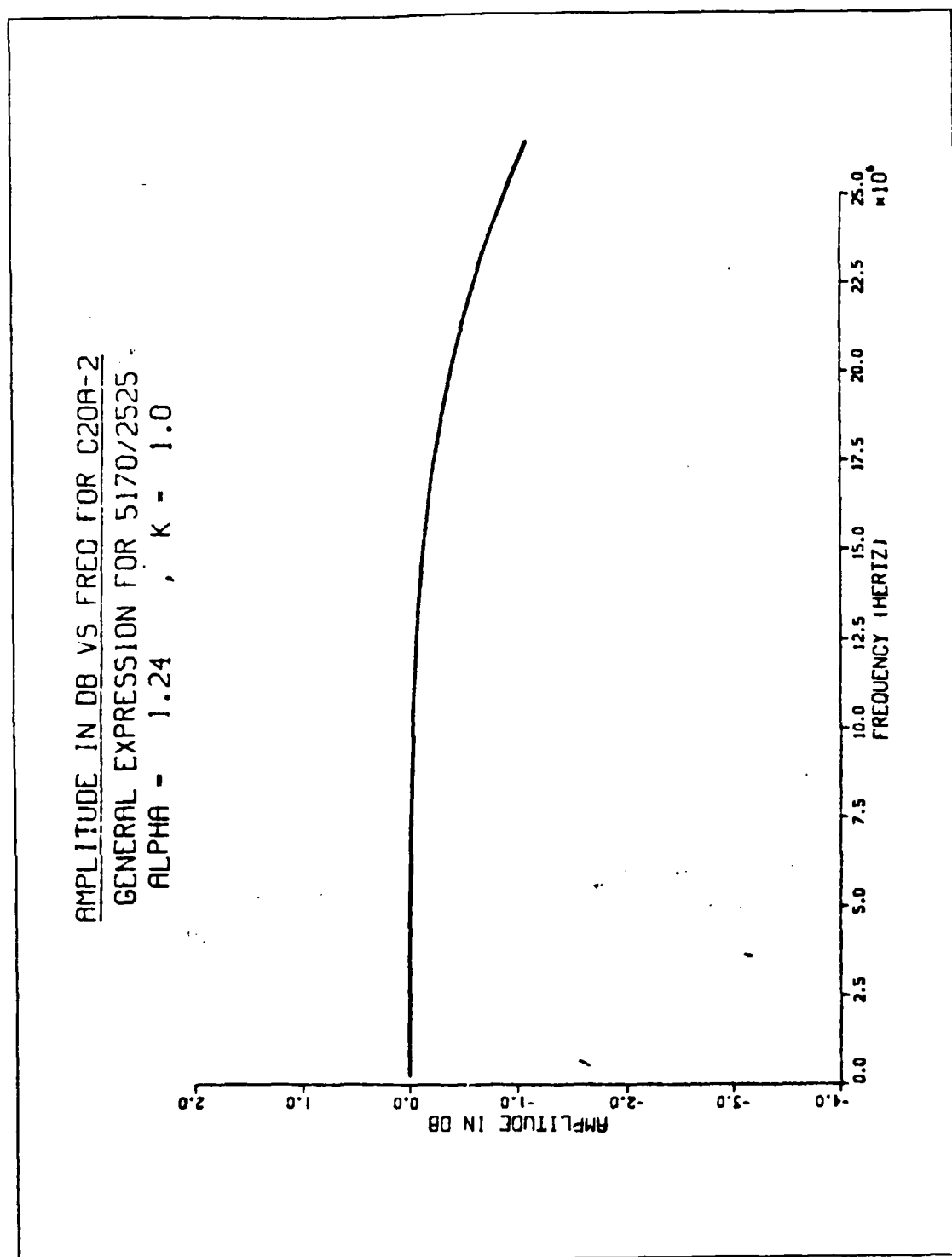
Figure 2.17 Computer Generated Frequency Response of C20A-2 Utilizing a Single Pole Model
