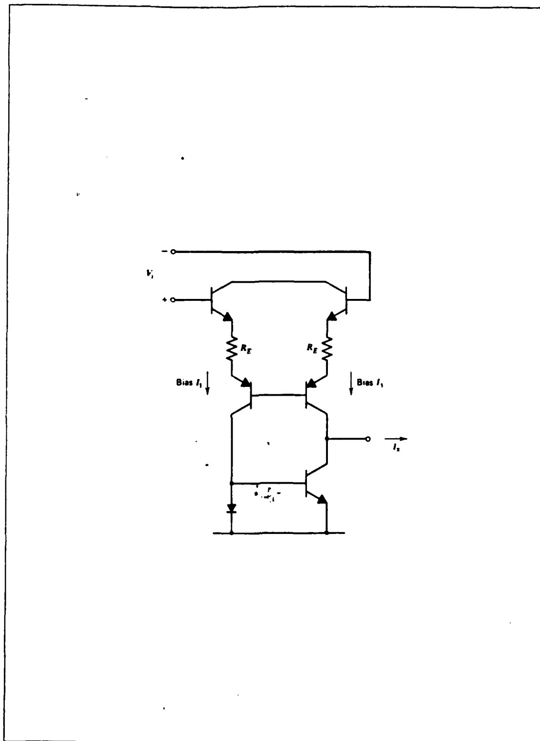
Figure 1.10 Inclusion of Emitter Resistors in First Stage of Op-amp
