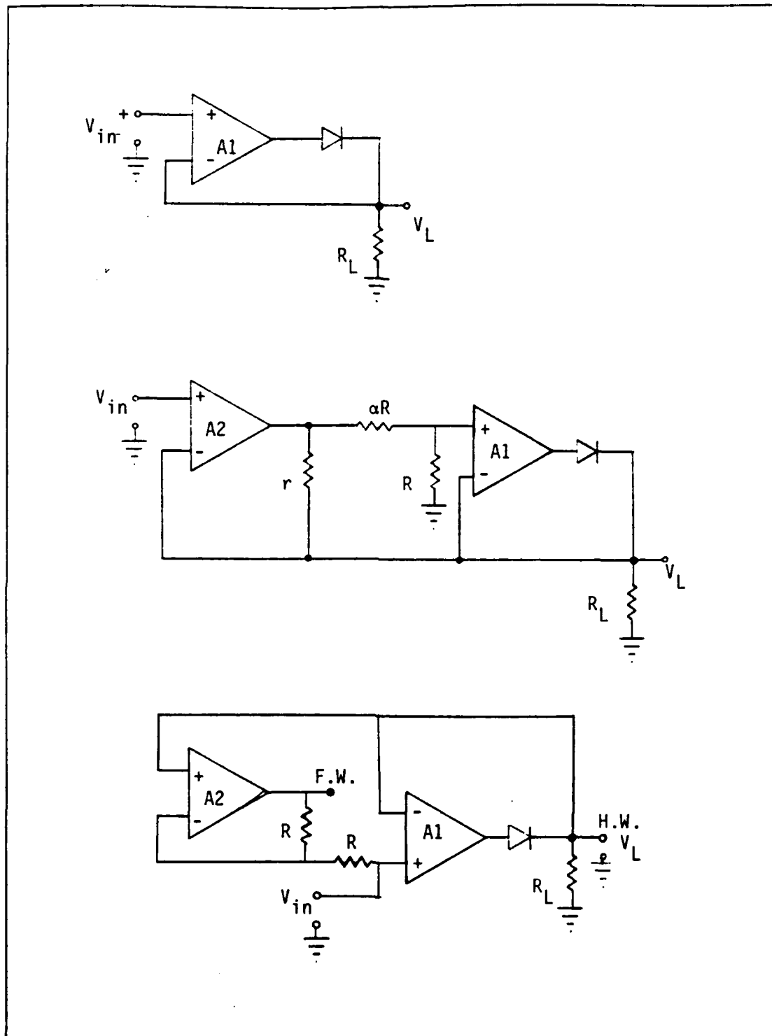
Figure 4.6 (a) Superdiode Circuit (b) Composite Superdiode Circuit (c) Improved Composite Superdiode Circuit
