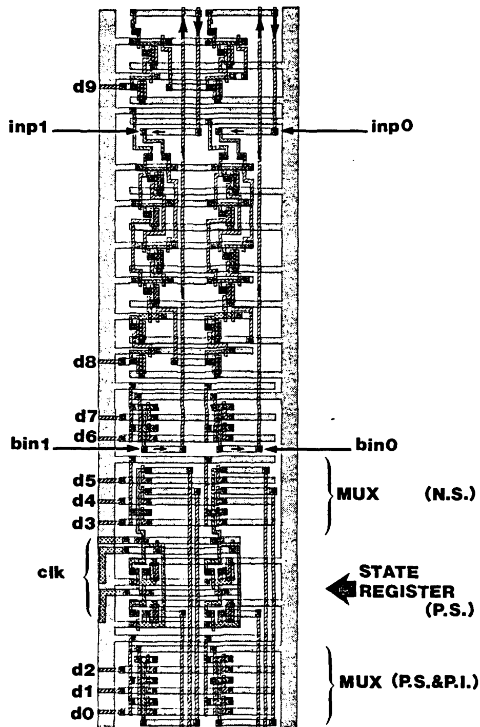
Figure 4.5 Data Path Arithmetic Block From GC.cif
