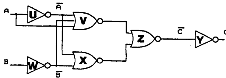
Figure 2.28 Gate Equivalent of Casand Weinberger Array
