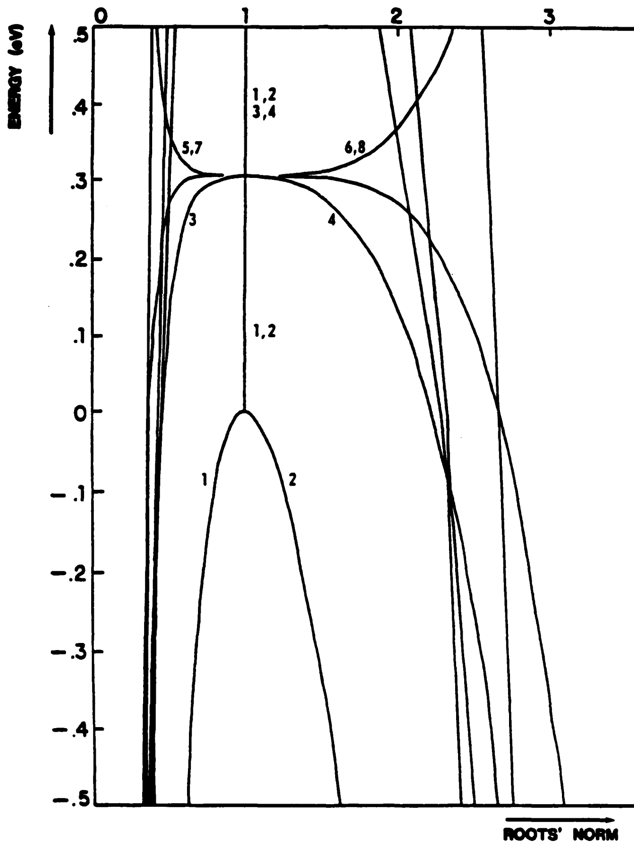
FIGURE 3 Locus of the roots of GaAs bandstructure of Figure 1 as a function of the energy.
