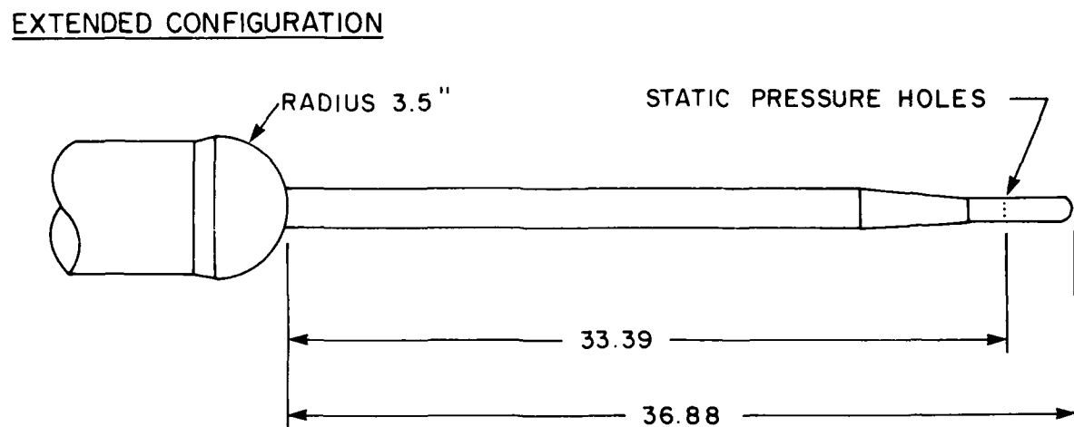
FIG. 3: SCHEMATIC AND DIMENSIONS OF THE PROBE IN THE SHORT AND EXTENDED CONFIGURATIONS
