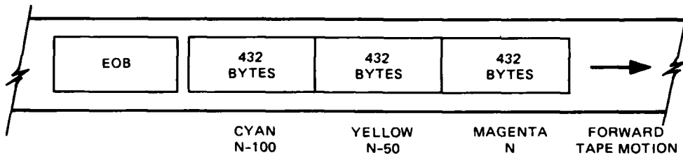
a. DATA FORMAT OF BLOCK NUMBER N ON A COMPUTER COMPATIBLE-MAGNETIC TAPE FOR THE TRI-COLOR IMAGE DATA CONVERTOR
