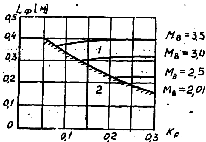
Fig. 6. Dependence of flame jet length on K_F and M . The mixture H_2 + \text{air} , T_g^* = 2500^\circ K , P_g = 4905 \text{ N/m}^2 , \alpha_g = 1 , \epsilon_r = 0.01 , 1 - region of stall-free flow; 2 - region of choking.
