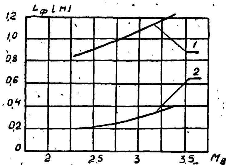
Fig. 7. Dependence of flame jet length on M for different fuel mixtures. 1 - kerosene + air, 2 - H_2 + \text{air} , P = 4905 \text{ N/m}^2 , T = 2500^\circ K , \alpha_g = 1 , K_F = 0.2 , \epsilon_r = 0.01 .
