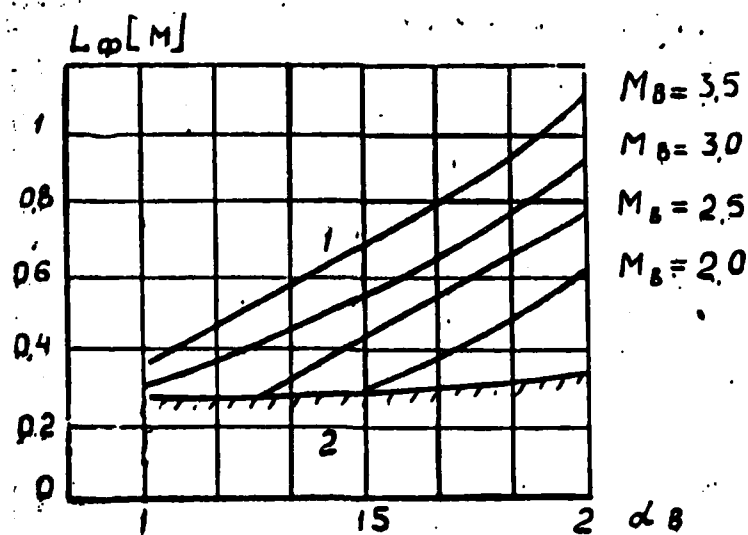
Fig. 5. Dependence of flame jet length on \alpha_g and M_b . Mixture H_2 + \text{air} , T_{g^*}=2000^\circ\text{K} , P_g=2943 \text{ N/m}^2 , \alpha_g=0.01 , K_r=0.2 , 1 - region of stall-free flow; 2 - region of choking.
