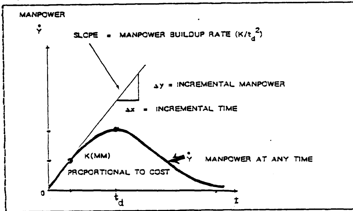
Figure 4.1 Rayleigh Function as Software Management Tool.
