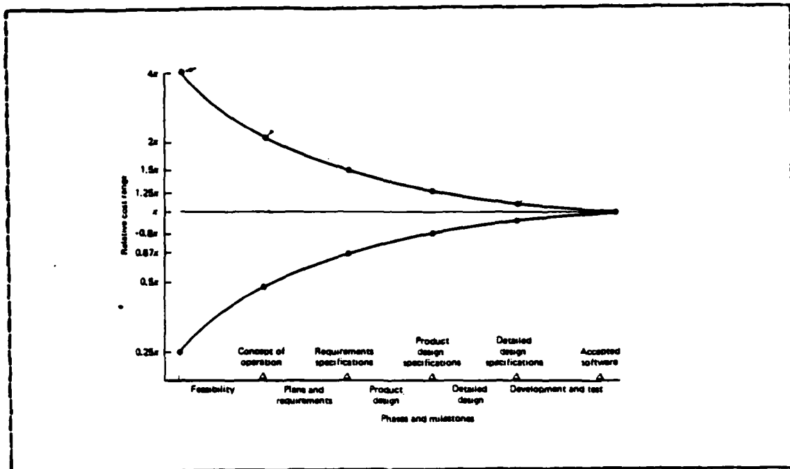
Figure 2.2 Software Cost Estimation Accuracy vs. Phase.
