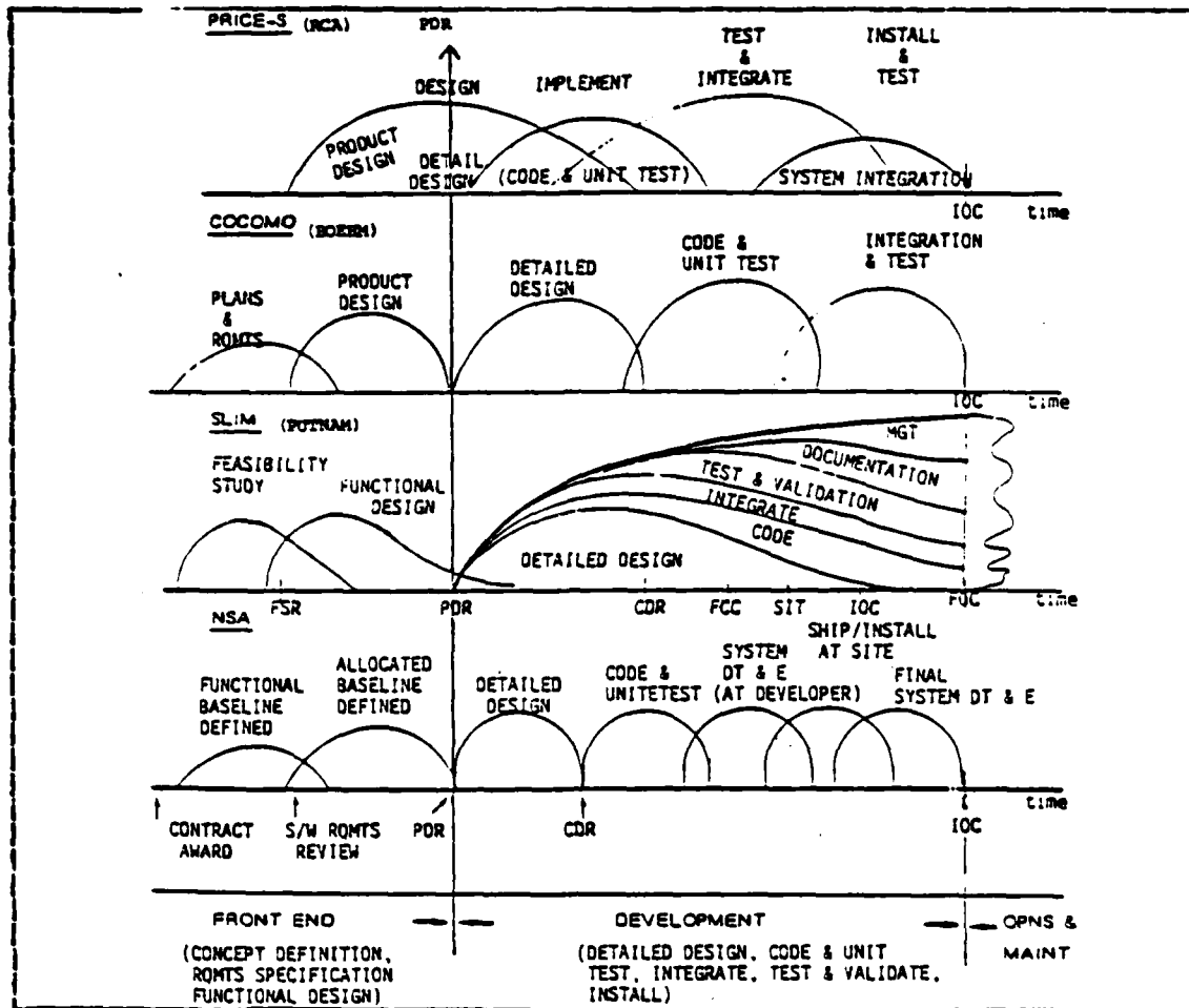
Figure 2.1 Software Life-Cycle.
