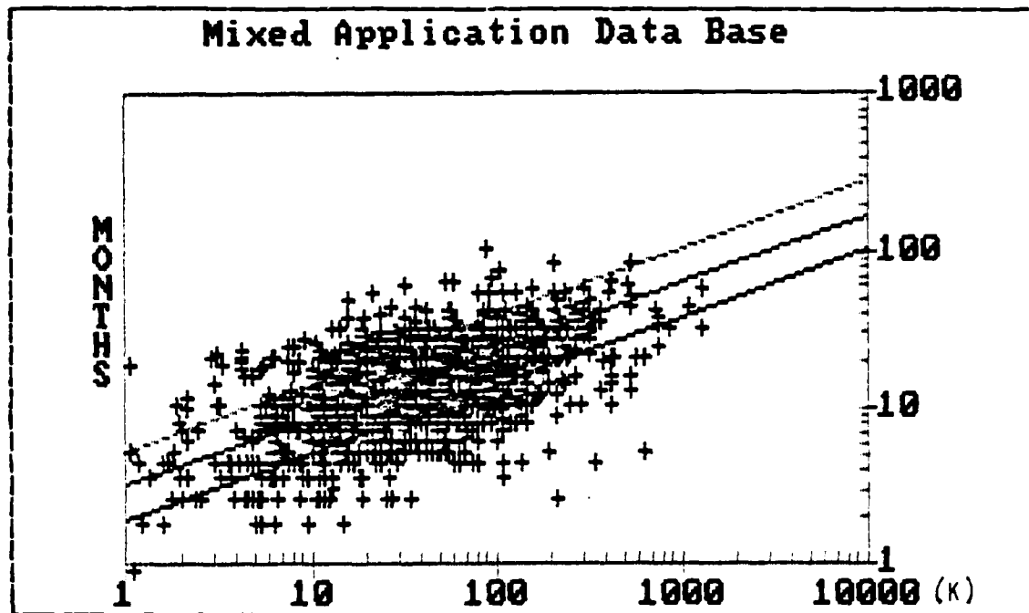
Figure 3.1 QSM Database Software Size vs. Development Time.
