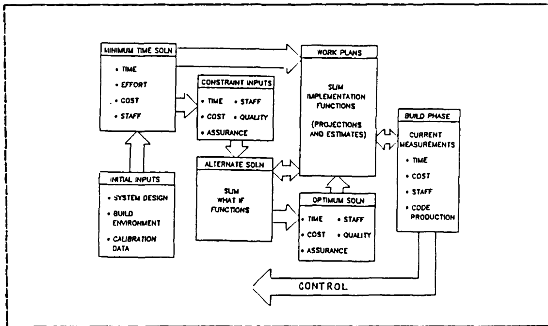
Figure 4.4 SLIM Diagram [Ref. 4]
