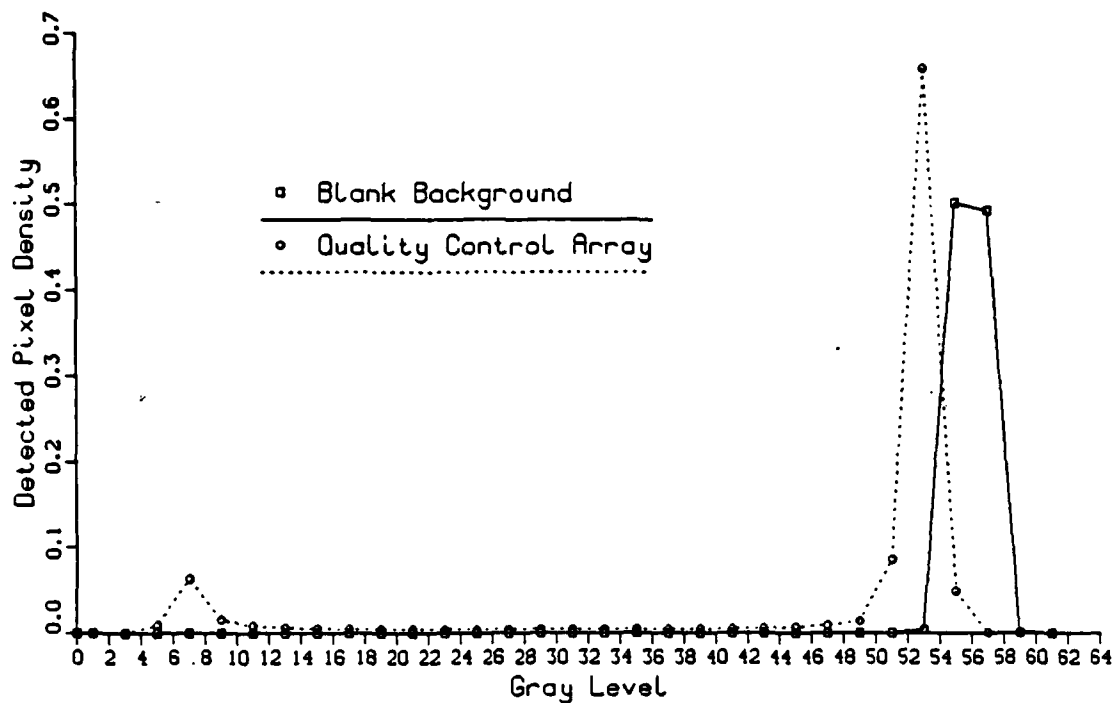
Figure 6.7 Gray Level Distribution of Reticle
