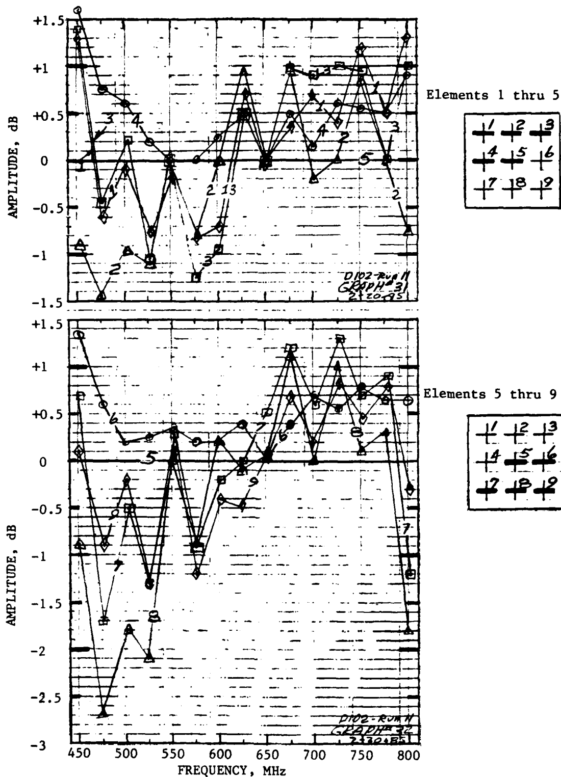
Fig. 10 - 3 \times 3 array individual dipole amplitude response wrt center element using Nurad horn source, horizontal polarization.
