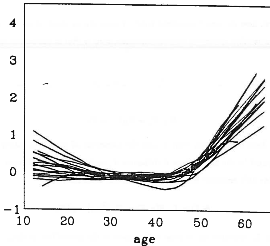
Figure 7. 20 Bootstraps of the local likelihood estimate, for the Stanford heart transplant data
