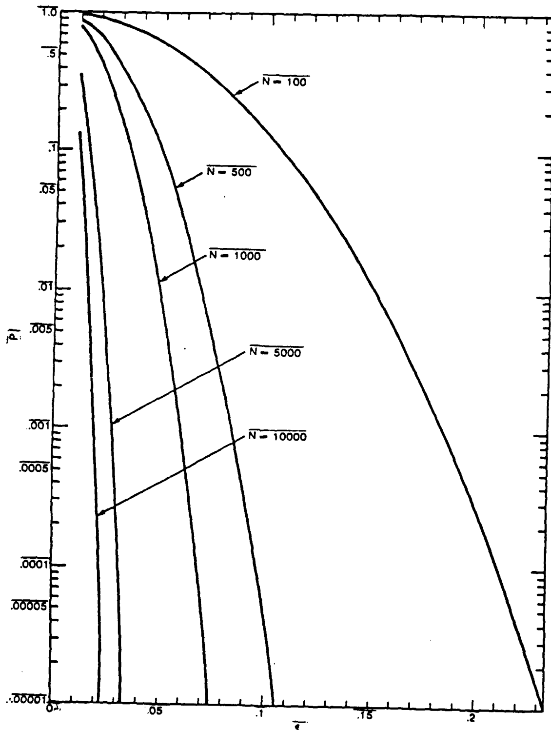
Figure 5.2a Chernoff Bound
