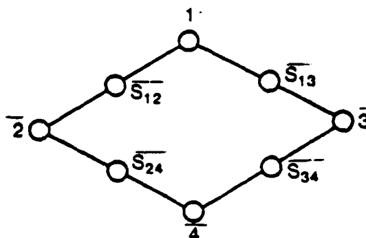
Figure 6.1b Process-communication Graph
