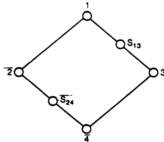
Figure 6.2 Process-communication Graph
