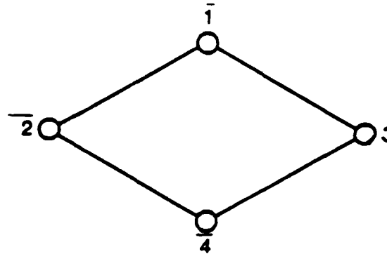
Figure 6.1a Process Graph
