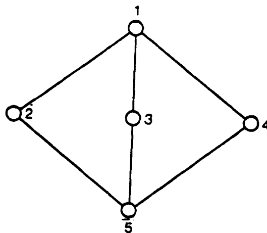
Figure 6.4 Process Graph
