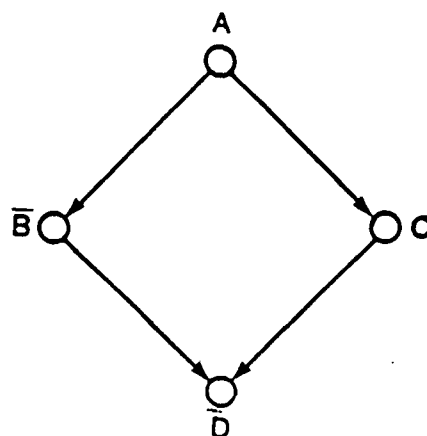
Figure 4.5 Process Graph
