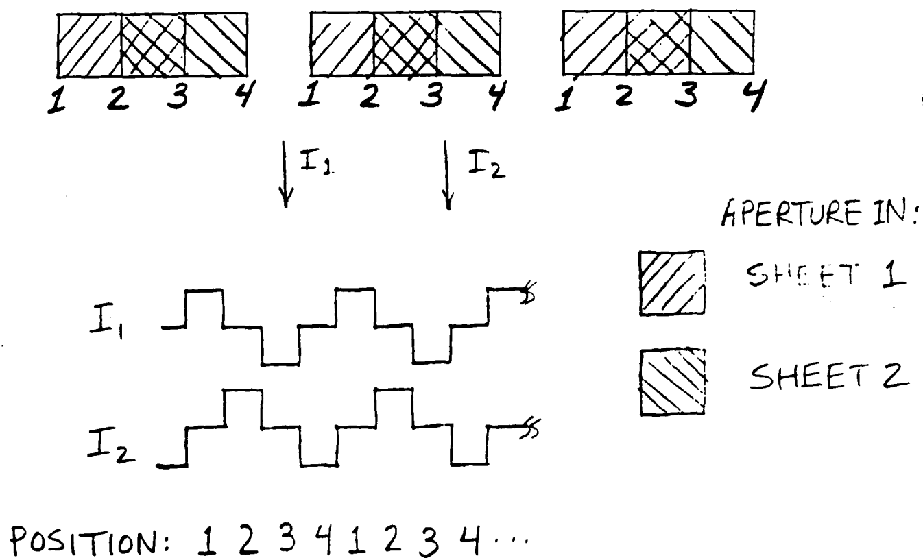
Figure 2: Overlapping Apertures in Two Conductive Sheets
