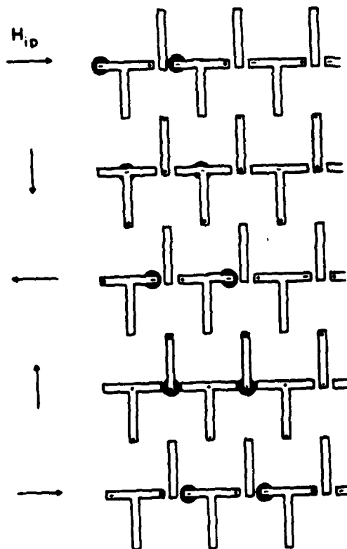
Fig. 1-4: Permalloy Propagation Patterns
