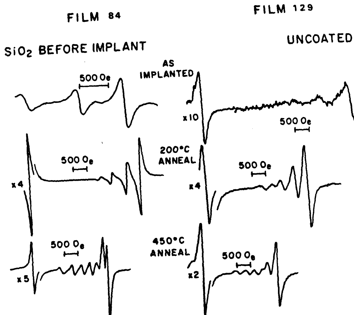
Fig. 3-52: Resonance Spectra for Films 84 and 129 - As Implanted, 250 °C Anneal, 450°C Anneal f = 4.5 GHz
