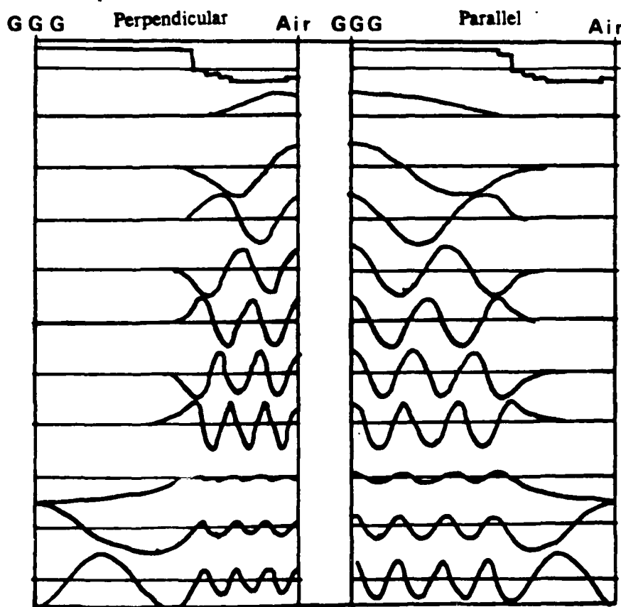
Fig. D-1: Depth Dependence of Spin Wave Solutions for 700°C Fit Perpendicular and Parallel Modes
