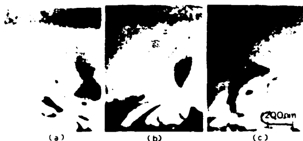
FIG 9 Bright-field images perpendicular to the implanted surface following implantation with deuterium at 60 keV and a dose of 1.5 \times 10^{16} \text{ D}_2^+/\text{cm}^2 and then with oxygen at 110 keV and a dose of 2.9 \times 10^{14} \text{ O}^+/\text{cm}^2 and subsequent annealing for 5 min at (a) 250, (b) 300, (c) 350 °C.
