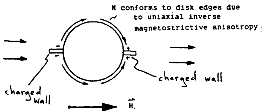
Fig. 1. Charged walls form in ion-implanted bubble devices due to stress relief.
