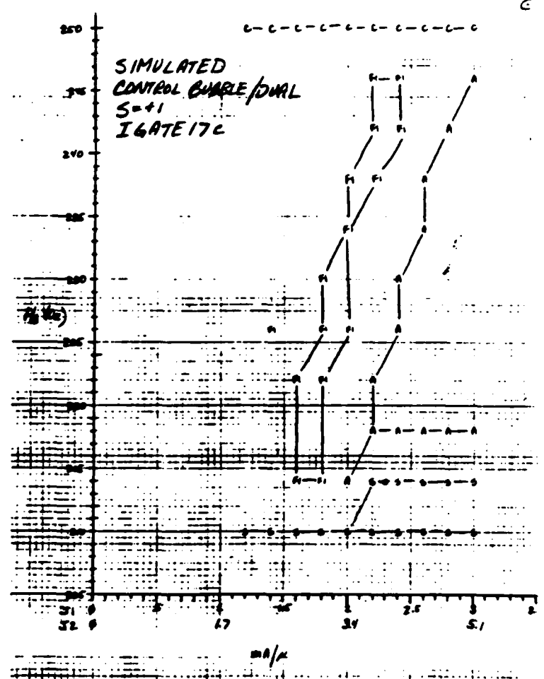
Figure 9: Empirical and Simulated Margins: Gate #17 Control Bubble/Dual Input, Positive Bias Field
