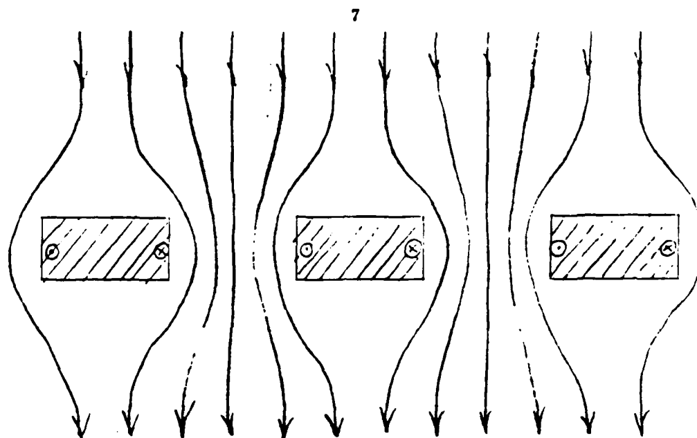
Figure 1: Fields Produced by Planar Current Flow Around Aperture
