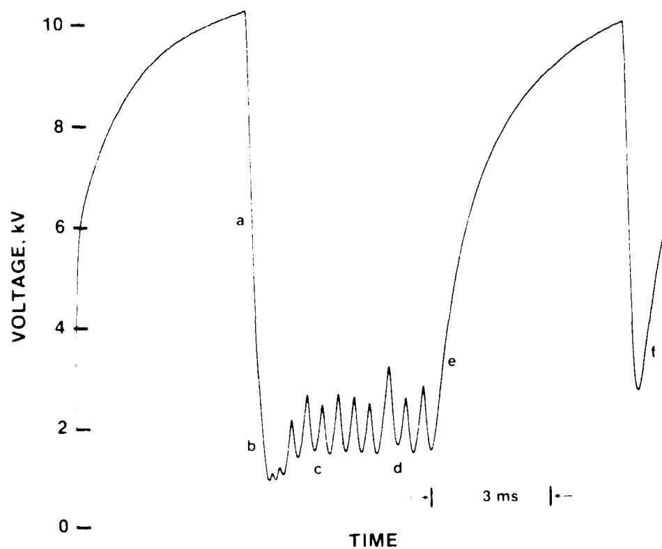
Figure 2.9 Example of a Multiple Low Voltage Prefire, U = 4.1 \text{ m/s} , \tau = 10^3
