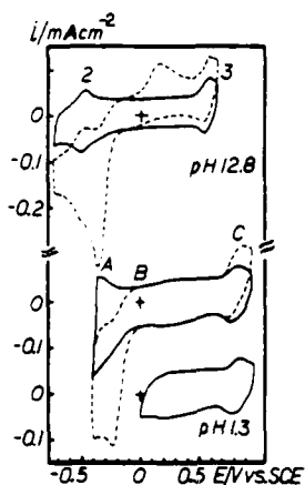
Fig. 10. Cyclic voltammograms on OPG in 0.05 M Na 2 SO 4 , pH 12.8 and pH 1.3 containing 10 -5 M Co(II)-TsPc under N 2 (—) and O 2 (●●●); scan rate 500 mV/s; no rotation. (Note: at pH 1.3 when the lower limit is 0.0 V, there is no difference between N 2 and O 2 voltammograms.)
