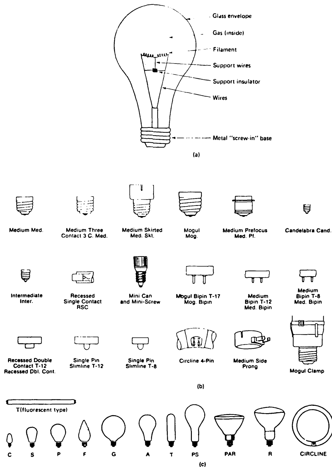
Figure 5.2 (a) Incandescent lamp; (b) common lamp bases; (c) common bulb designations (3:95).
