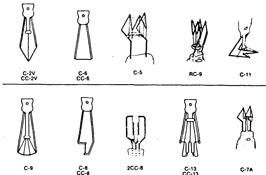
Figure 5.1 Incandescent lamp filament designs (3:96).
