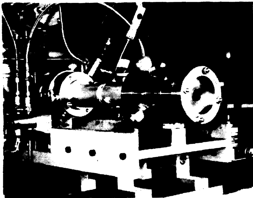
Figure 5. Experimental Thrust Stand and SFRJ
