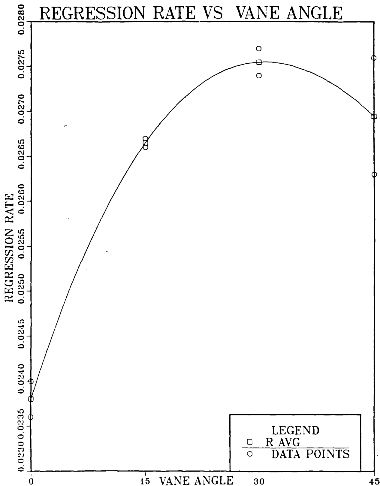
Figure 9. Regression Rate vs. Swirl Vane Angle
