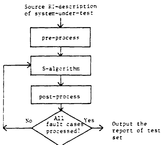
Figure 5 Simplified test generation flow
