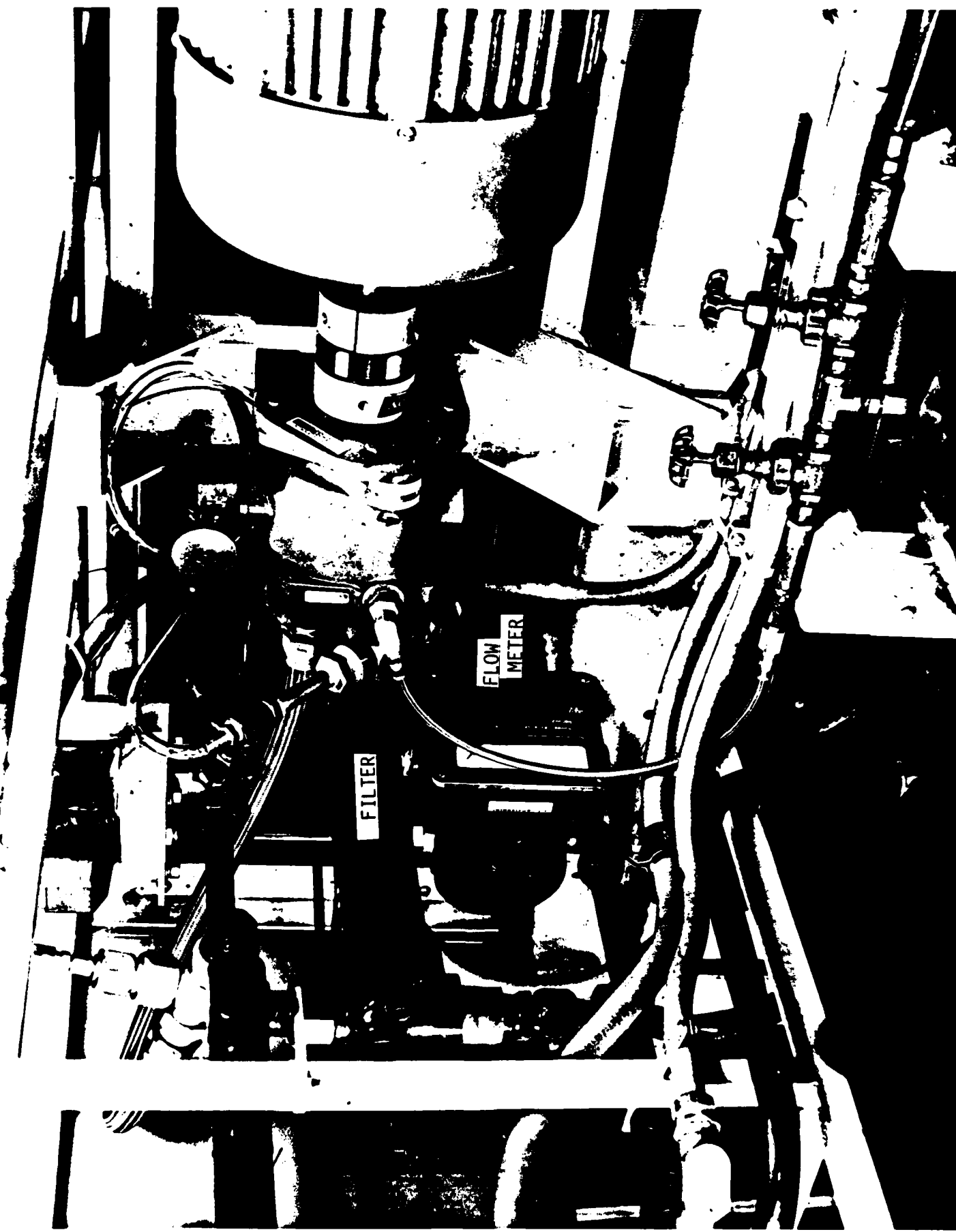
FIGURE 16. FILTER AND FLOWMETER
