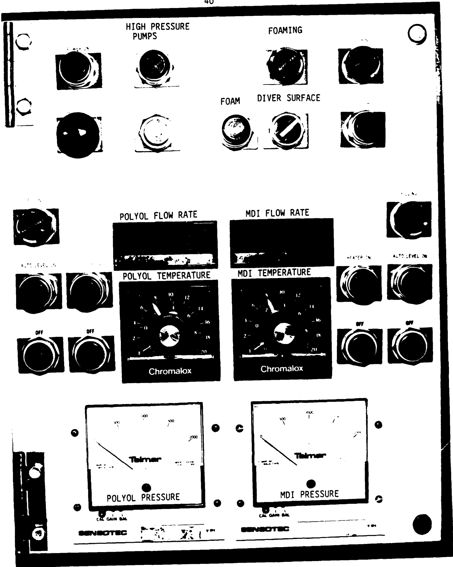
FIGURE 21. MAIN CONTROL PANEL
