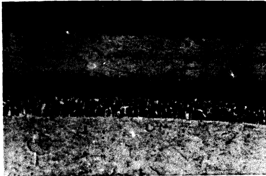
Figure 7. Coating No. 3 - Medium Pt Diffusion, Inward Al, Etched (425x)
