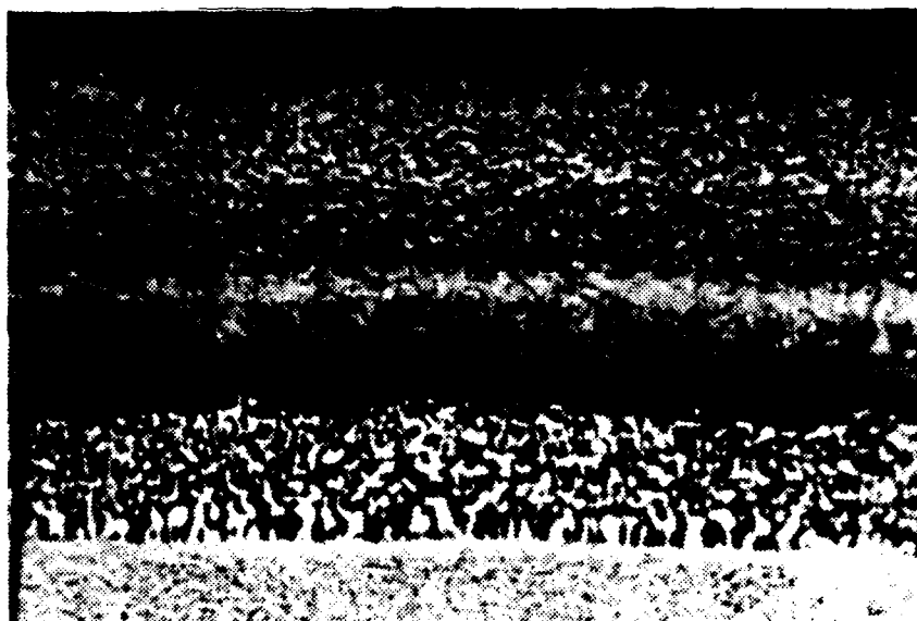
Figure 9. Coating No. 5 - High Pt Diffusion, Outward Ni, Etched (425x)
