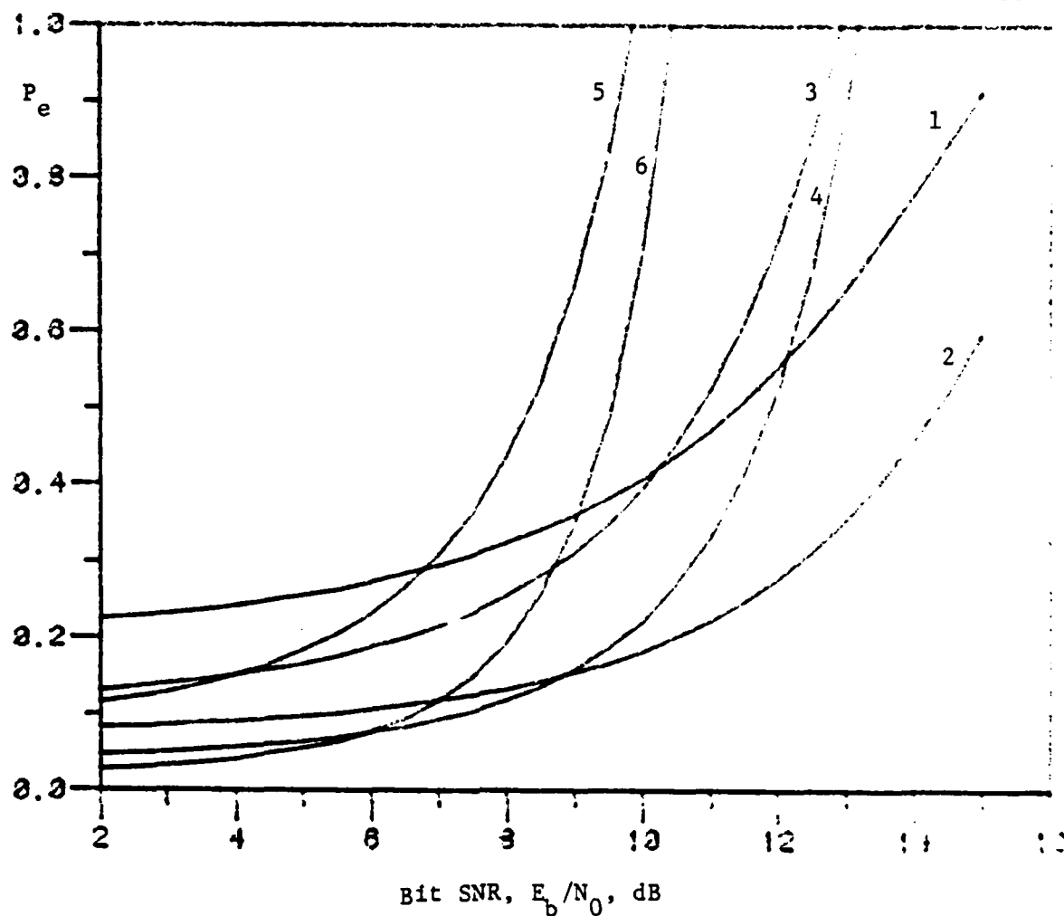
Figure A.2. Weighted graphs of c \cdot P_e\left(\frac{n}{N} \frac{E_b}{N_0}, x\right) with n = 5 , N = 32 . Six fixed values of x\left(\triangleq \frac{n}{2} \frac{E_b}{N_0}\right) are used.
