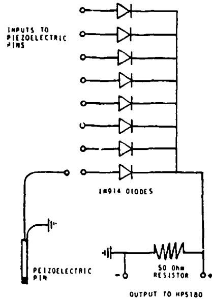
Fig. 7. Circuit for Multiplexing Piezoelectric Pin Response.
