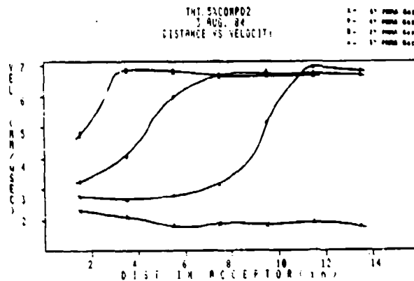
Fig. 18. Velocity vs Distance along Acceptor for TNT/5%-Wax
