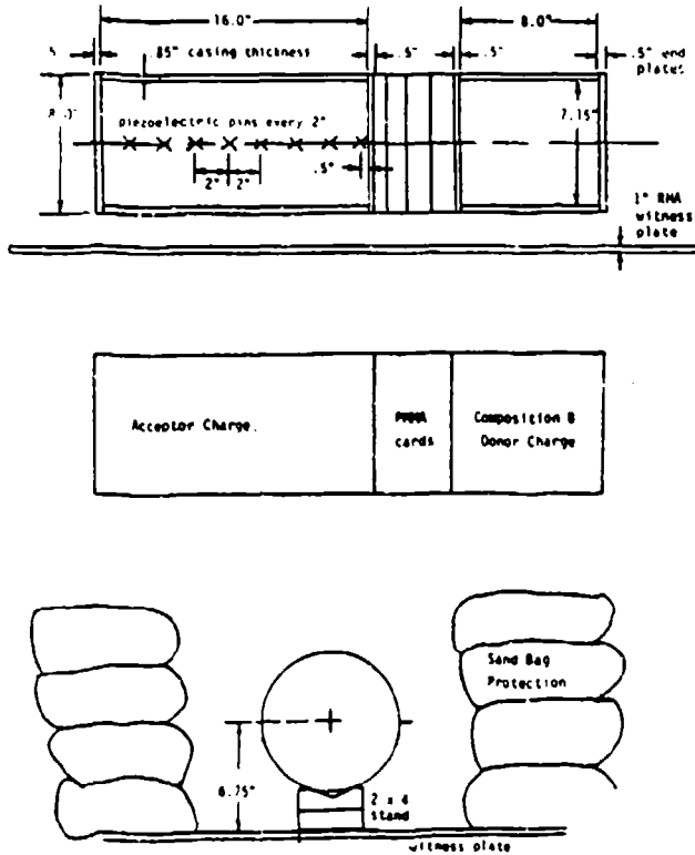
Fig. 1. Set-up of the Super Gap Test
