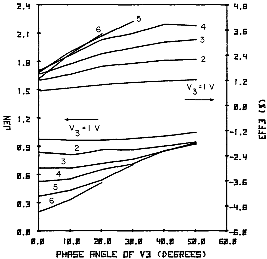
FIG. 2.40 J_{3N} AND Eff_3 VS. \theta_{3V} AT V_1 = 37 V FOR A GaAs UNIFORM DIODE.
