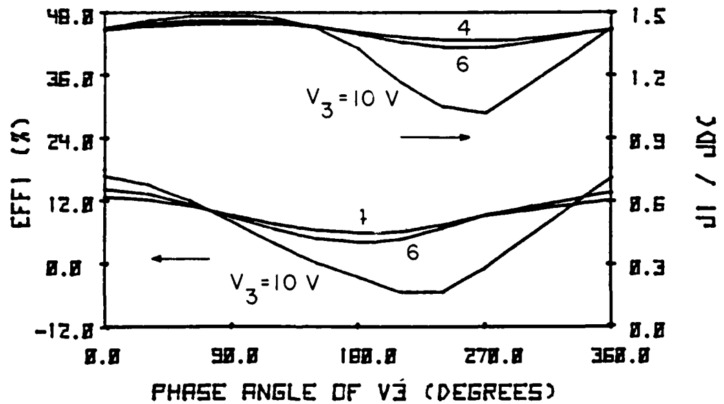
FIG. 2.65 FUNDAMENTAL AND THIRD-HARMONIC EFFICIENCIES AND CURRENTS FOR pin DIODE 3 AT J_{dc} = 7.5 kA/cm 2 AND V_1 = 38 V.
