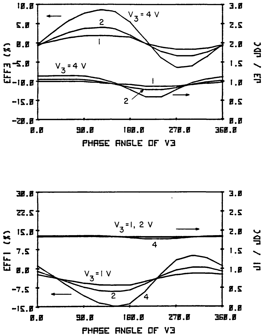
FIG. 2.62 FUNDAMENTAL AND THIRD-HARMONIC EFFICIENCIES AND CURRENTS FOR pin DIODE 2 AT J_{dc} = 7.5\text{ kA/cm}^2 AND V_1 = 16\text{ V} .
