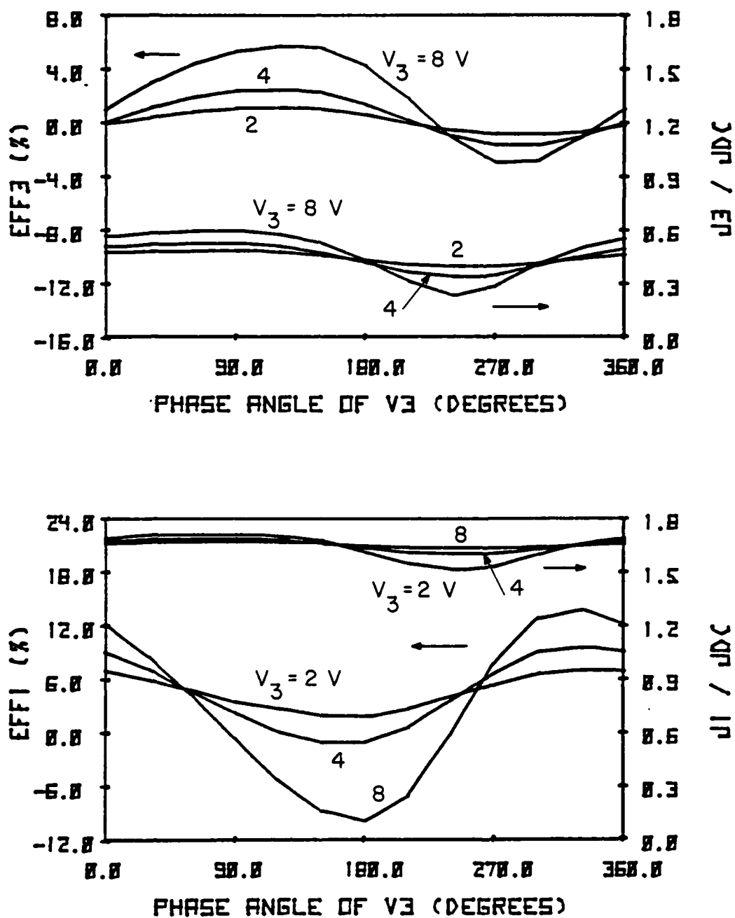
FIG. 2.57 FUNDAMENTAL AND THIRD-HARMONIC EFFICIENCIES AND CURRENT DENSITIES AT J_{dc} = 7.5 kA/cm 2 AND V_1 = 28 V.
