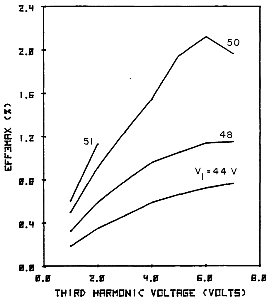
FIG. 2.33 MAXIMUM \text{Eff}_3 VS. THIRD-HARMONIC VOLTAGE AT DIFFERENT FUNDAMENTAL VOLTAGE AMPLITUDES FOR A Si HYBRID DIODE.
