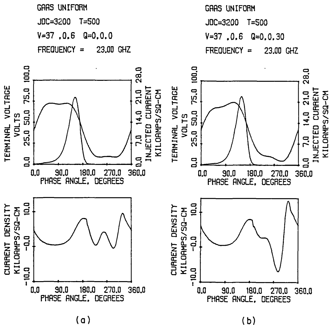
FIG. 2.39 LARGE-SIGNAL SOLUTIONS FOR A GaAs UNIFORM DIODE AT
