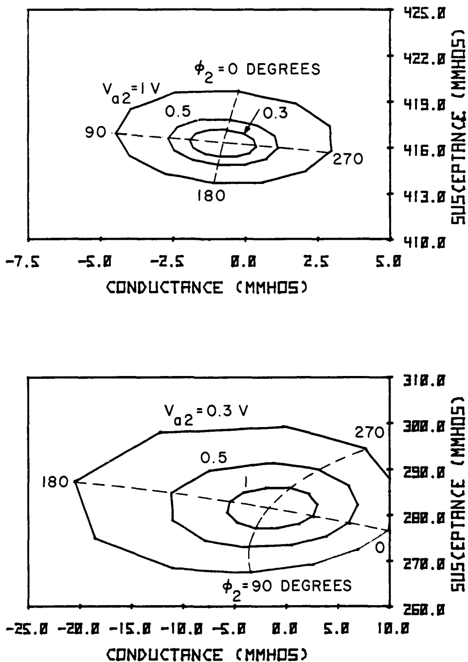
FIG. 3.5 DEVICE HARMONIC ADMITTANCE UNDER THE INFLUENCE OF SECOND-HARMONIC VOLTAGE FOR V_{a1} = 3.5 V, V_{a3} = 0.375 V AND \phi_3 = 0 DEGREES AT f_1 = 23 GHz.
