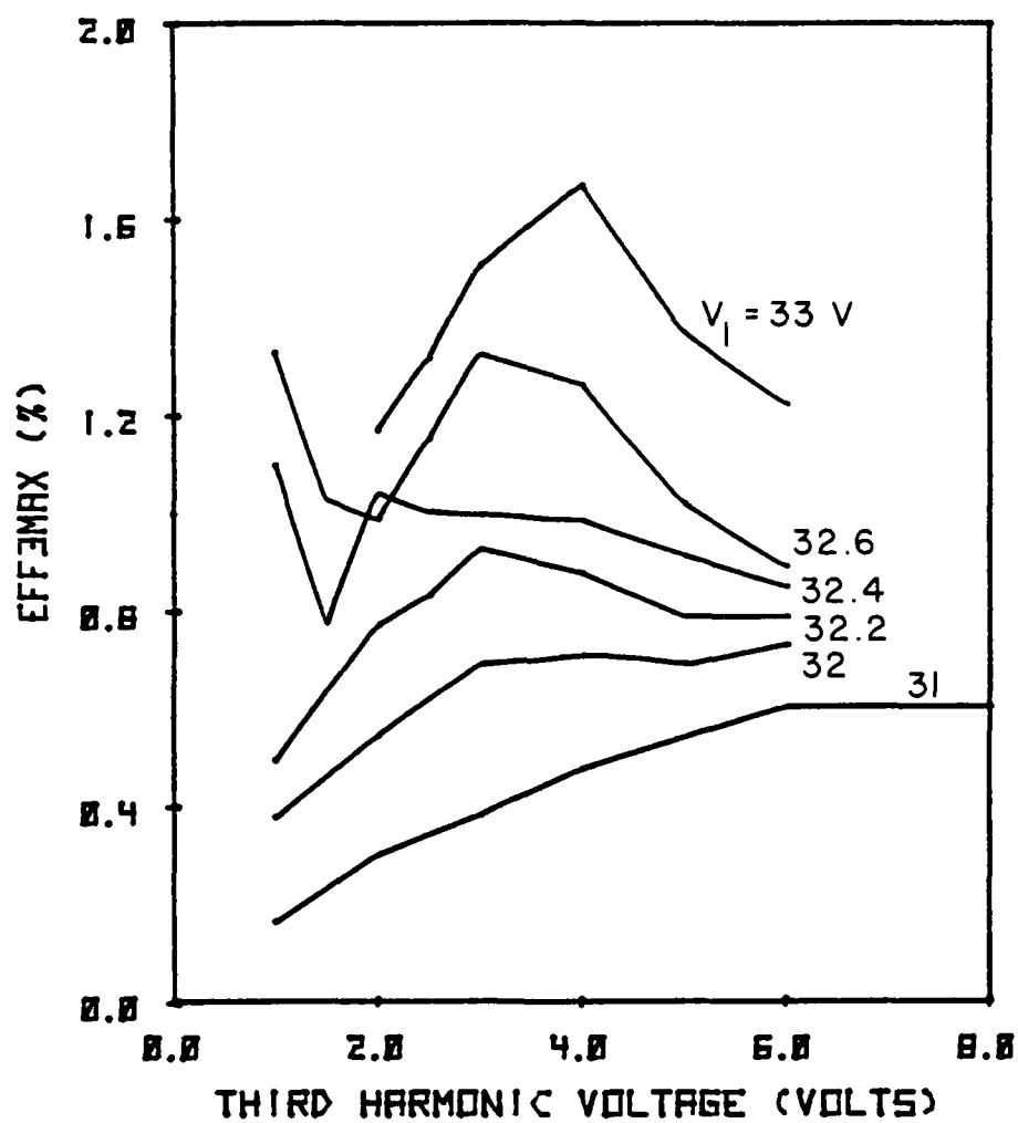
FIG. 2.29 MAXIMUM Eff 3 VS. THIRD-HARMONIC VOLTAGE AT DIFFERENT FUNDAMENTAL VOLTAGE AMPLITUDES FOR A GaAs READ DIODE.
