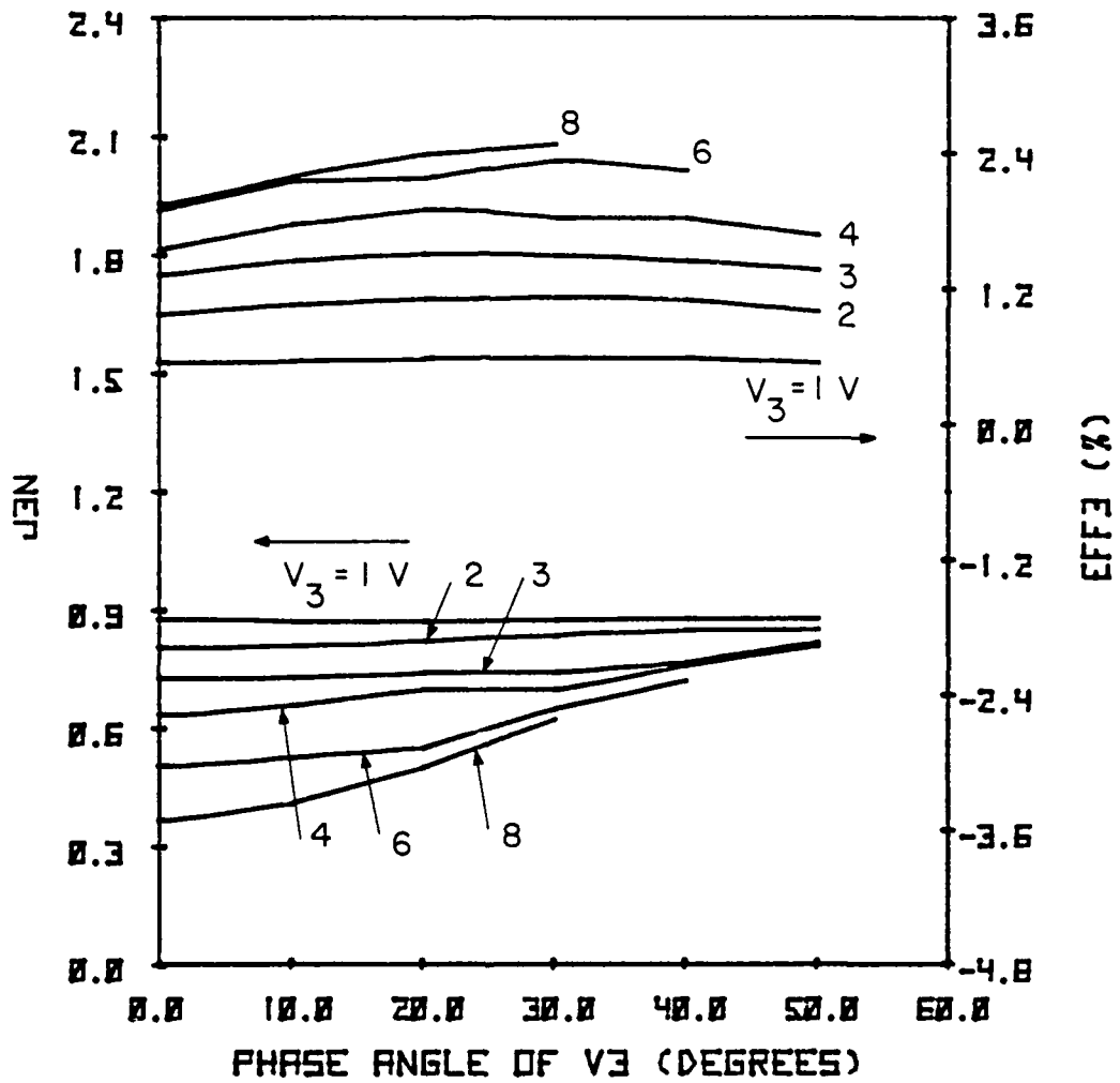
FIG. 2.36 J_{3N} AND \text{Eff}_3 VS. \theta_{3V} AT V_1 = 64 V FOR A Si UNIFORM DIODE IN TWO-FREQUENCY OPERATION.
