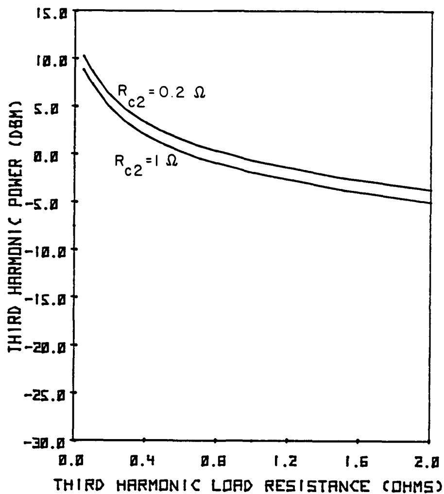
FIG. 3.10 OUTPUT POWER AT THE THIRD-HARMONIC FREQUENCY ( \sim 69 GHz) OBTAINED AT R_s = 0 \Omega FOR DIFFERENT HARMONIC LOAD RESISTANCES. ( R_{c2} = 0.2 AND 1 \Omega AND R_{c3} = 0.1 TO 2 \Omega )
