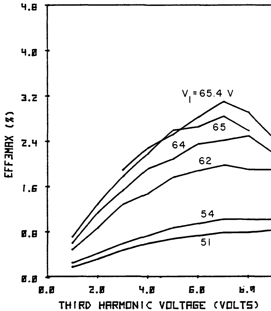
FIG. 2.37 MAXIMUM Eff 3 VS. THIRD-HARMONIC VOLTAGE AT DIFFERENT FUNDAMENTAL VOLTAGE AMPLITUDES FOR A Si UNIFORM DIODE.
