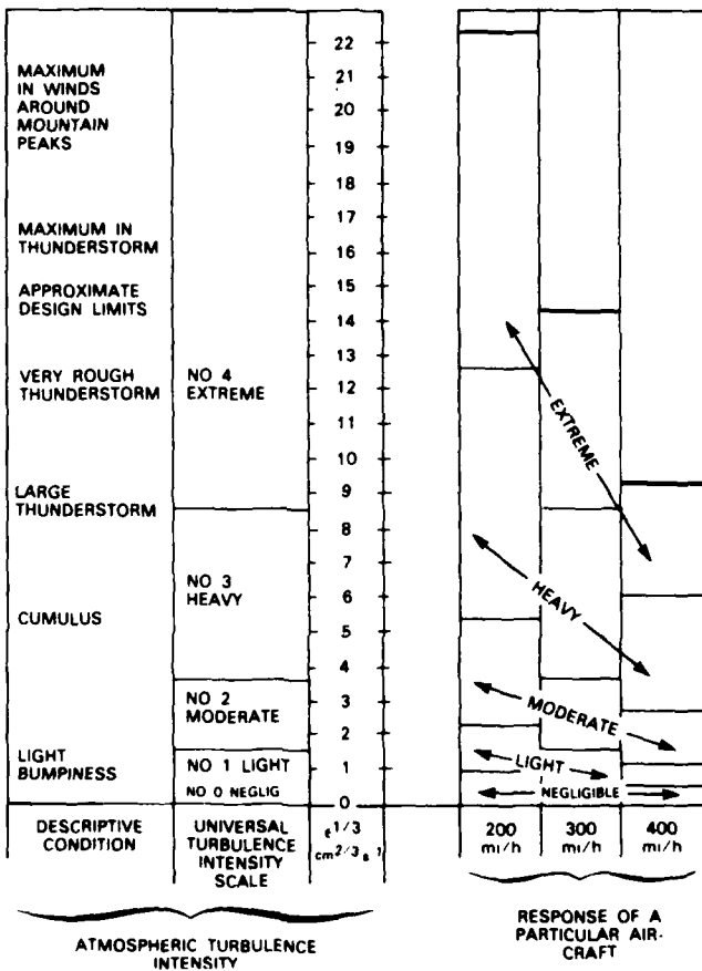
Figure IV-12. Turbulence scale suggested by MacCready 9 .
