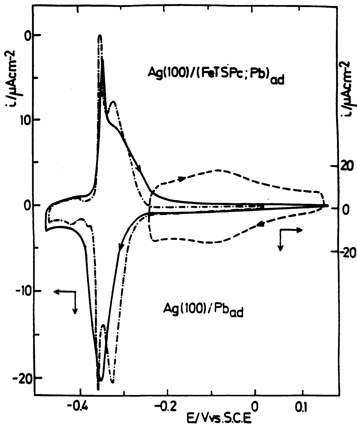
Fig. 3. Underpotential deposition of Pb on the Ag(100) surface in 0.1 \text{ M HClO}_4 with 10^{-3} \text{ M Pb}^{2+} , without (---) and with (—) preadsorbed Fe-TsPc. Sweep rate 5 \text{ mV s}^{-1} . Dashed line gives the curve obtained with the sweep rate 0.2 \text{ V s}^{-1} (see text).
