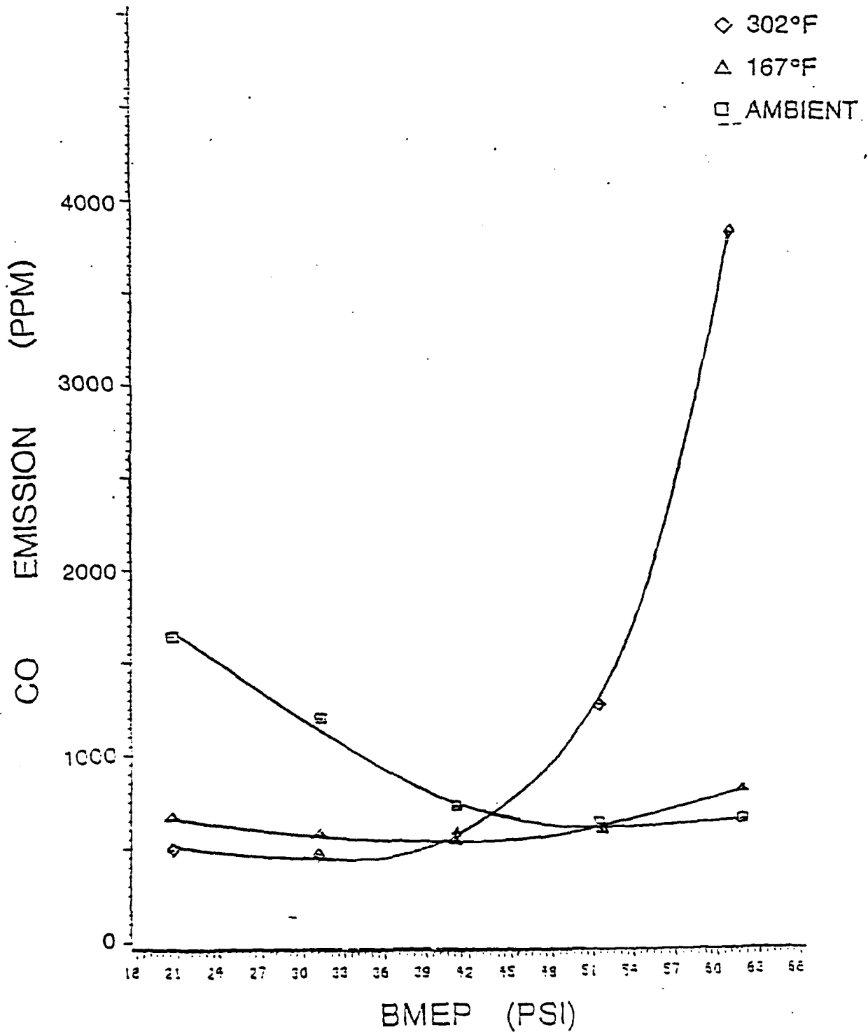
Figure 41 Effect of Engine Load and Air Intake Temperature on Co Emission For 30% w/Diesel Emulsion at 2000 RPM
