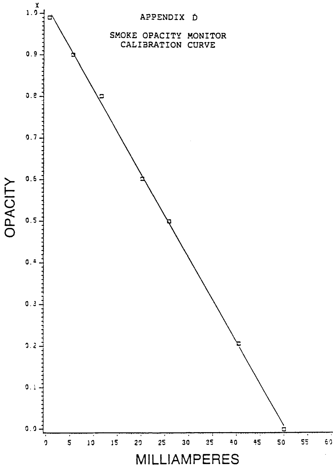
SMOKE OPACITY MONITOR CALIBRATION CURVE
