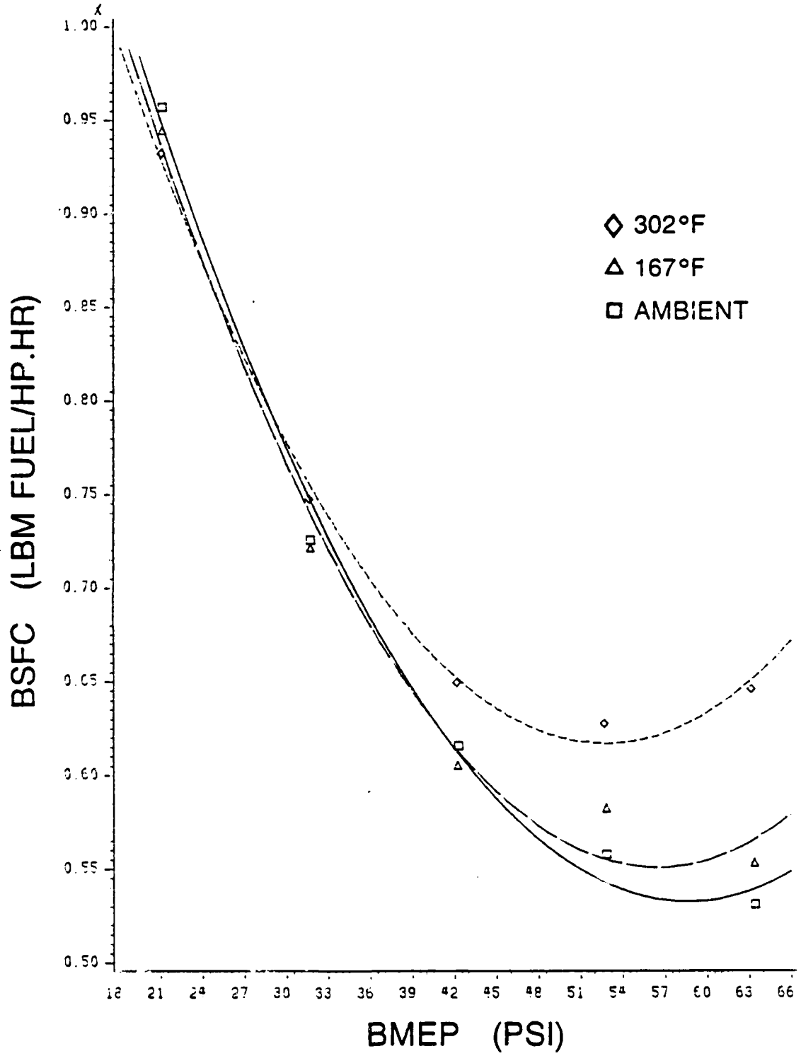
FIGURE 21 EFFECT OF ENGINE LOAD AND INTAKE AIR TEMPERATURE ON THE BSFC FOR 45 % WATER / OIL EMULSION AT 2000 RPM
