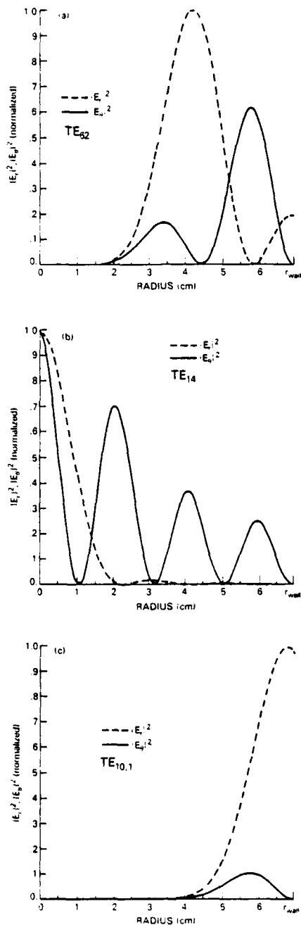
Fig. 5. Predicted microwave power as a function of radius across the experimental output window for (a) the TE 62 mode, (b) the TE 14 mode, and (c) the TE 10,1 mode. Each mode is separately normalized to a peak value of 1.0.
