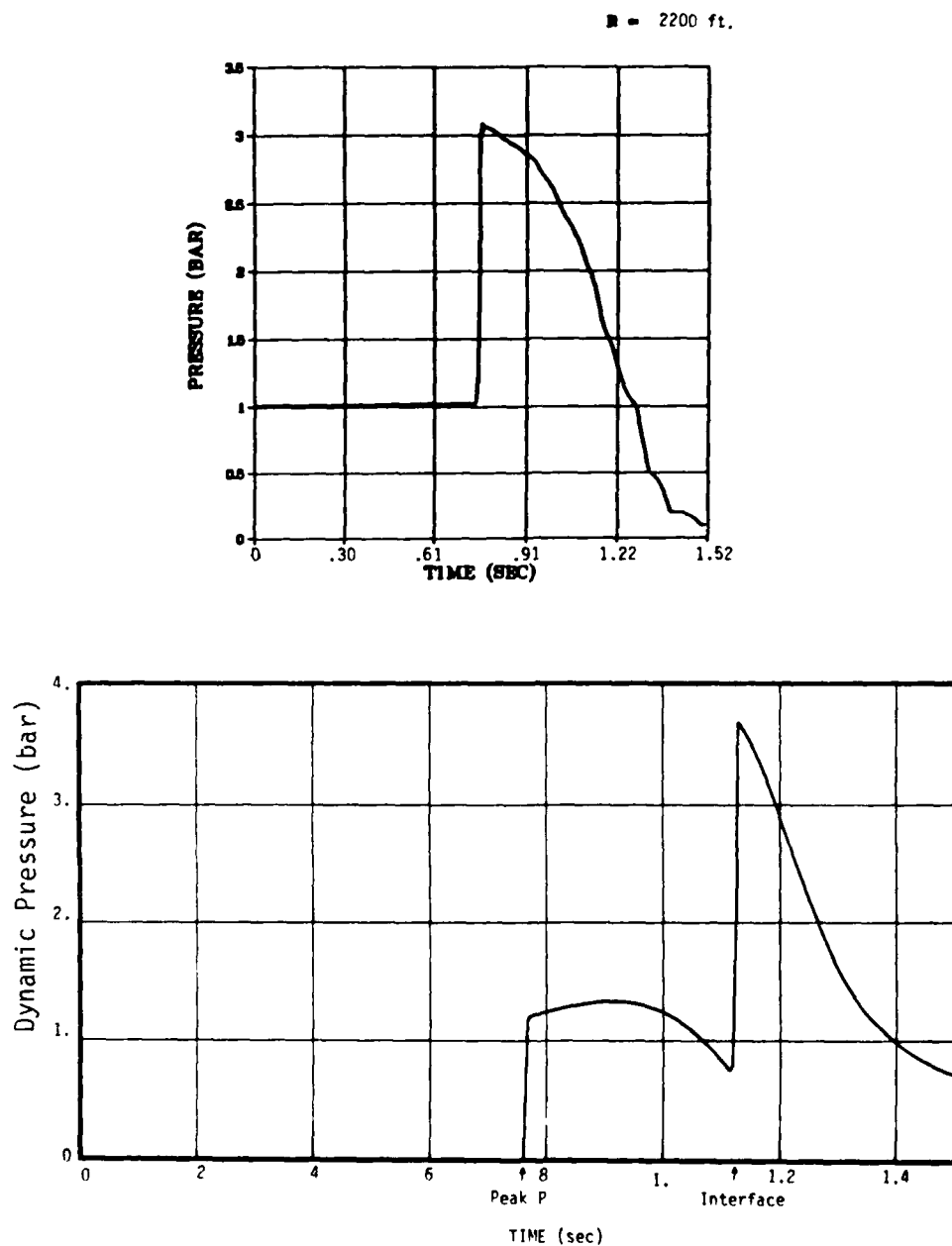
Figure 4.15. Static and dynamic pressure expected at the 2200 ft test chamber of DASACON from a compressed N_2 driver. The compression chamber is 5 ft in diameter and 165 ft long. The valve between the two chambers was assumed to open instantaneously. The initial driver pressure was 200 atm, and the temperature was ambient.
