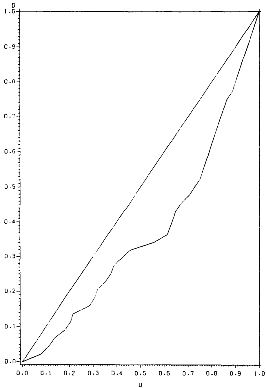
Figure 2. INTERNATIONAL AIRLINES DATA
