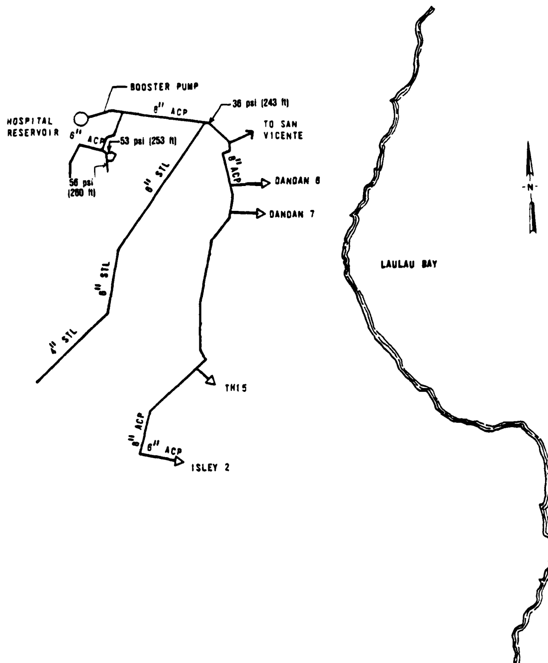
Figure A3. Isley/Dandan system: distribution schematic and static pressures and heads
