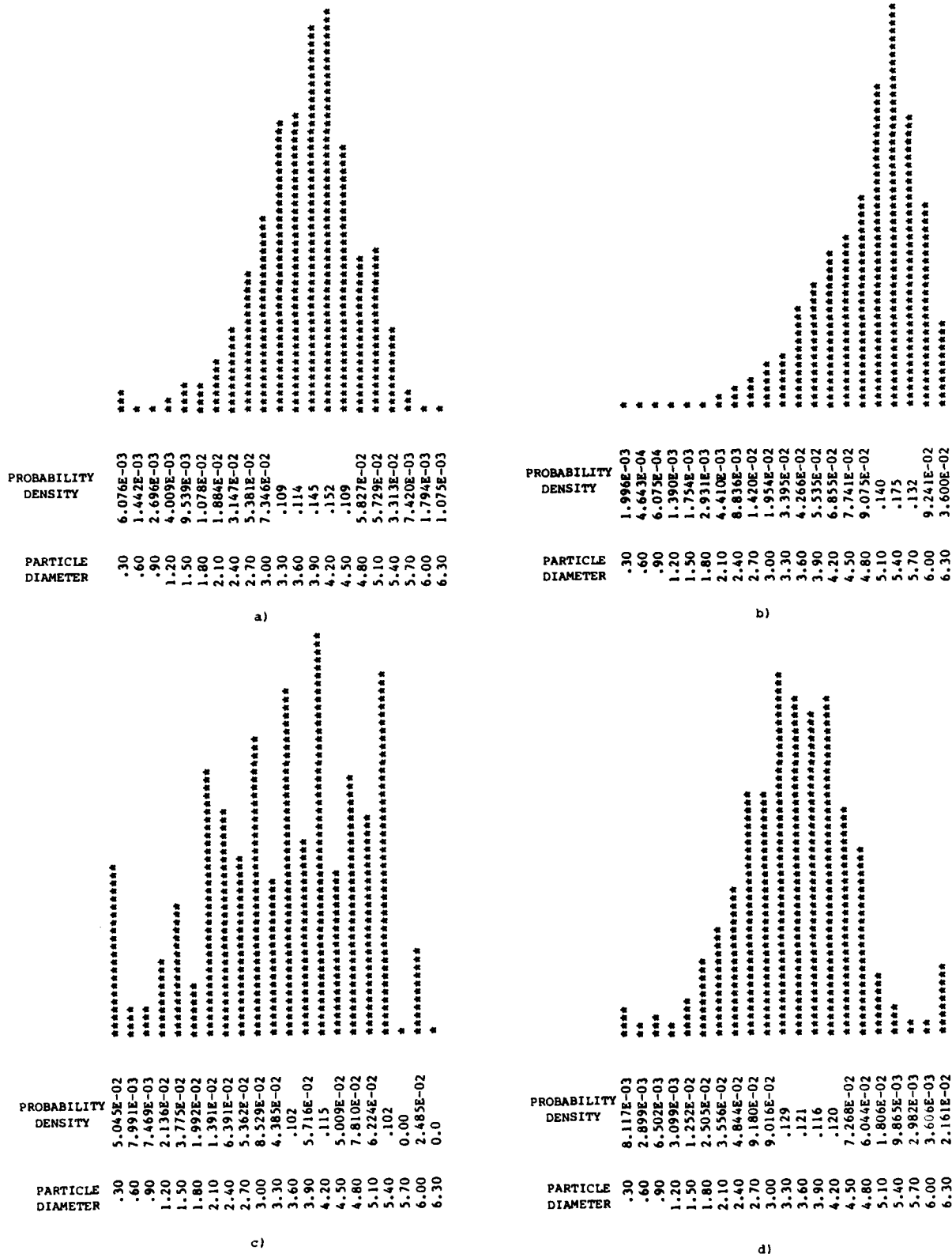
Figure 10. Comparison of ensemble averaged mass distribution for a) XM49 fog oil generator, b) M3A3 fog oil generator, c) VEESS diesel oil generator near the instrumentation cluster, and d) 30 m from VEESS oil generator...Smoke Week III....From Nelson and Farmer 1981. 2
