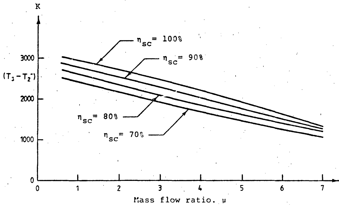
FIG. 2 CURVES USED TO DETERMINE PROPERTIES OF COMBUSTION PRODUCTS AT STATION 3.
