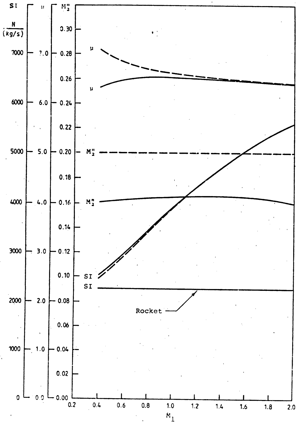
——— Optimum performance curves with M_2 unrestricted - - - Optimum performance curves with M_2 fixed at 0.2 FIG. 3 OPTIMUM VALUES OF SI AND CORRESPONDING VALUES OF \mu AND M_2 VERSUS M_1 FOR REFERENCE CONDITIONS.
