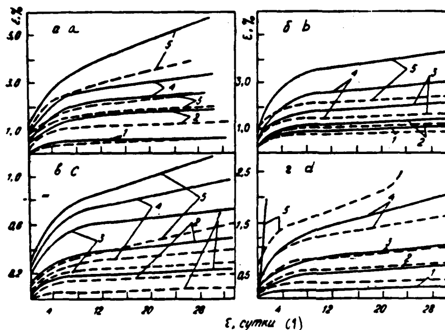
Fig. 1. Creep of P-12 (a) , STD (b), PETF (c), and PMMAF (d) in air (dashed lines) and in a physiological solution (solid lines) in the compression process at different values of \sigma/\sigma_{kp} : 1 - 0.05; 2 - 0.1; 3 - 0.2; 4 - 0.3; 5 - 0.4. Key: (1) days.
