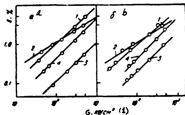
Fig. 2. Dependence of the maximum of nonstationary creep P-12 (1), STD (2), PETF (3), and PMMAF (4) in air (a) and a physiological solution (b) on stress \sigma under compression. Key: (1) \text{kg/cm}^2 .
