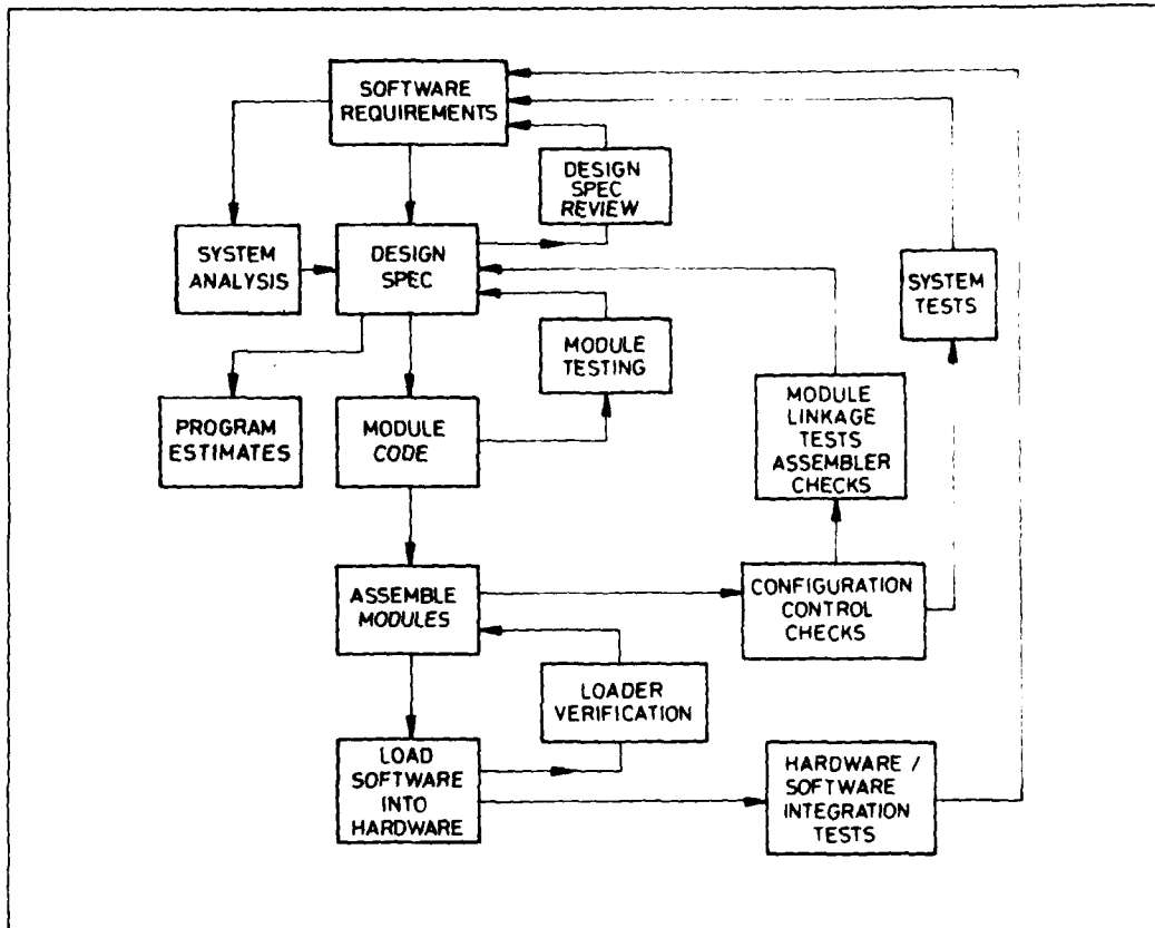
Figure 8 Software Development Process
