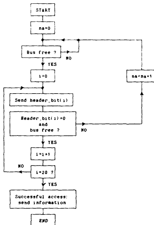
Figure 8: The CSMA/FIFO channel access algorithm (see figure 7 for content of vector "header_bit")
