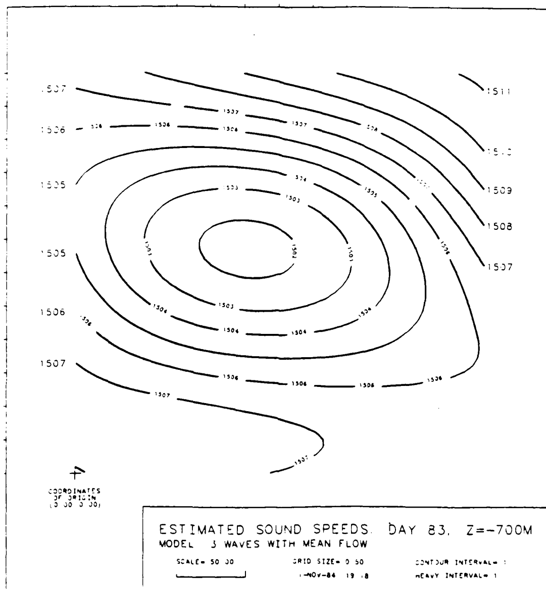
Figure 5.12. Sound-speed map at a depth of 700 m of the optimally estimated wave field in the experimental square on yearday 83. Contour interval is 1 m/s and the reference sound-speed at this depth is 1506 m/s.
