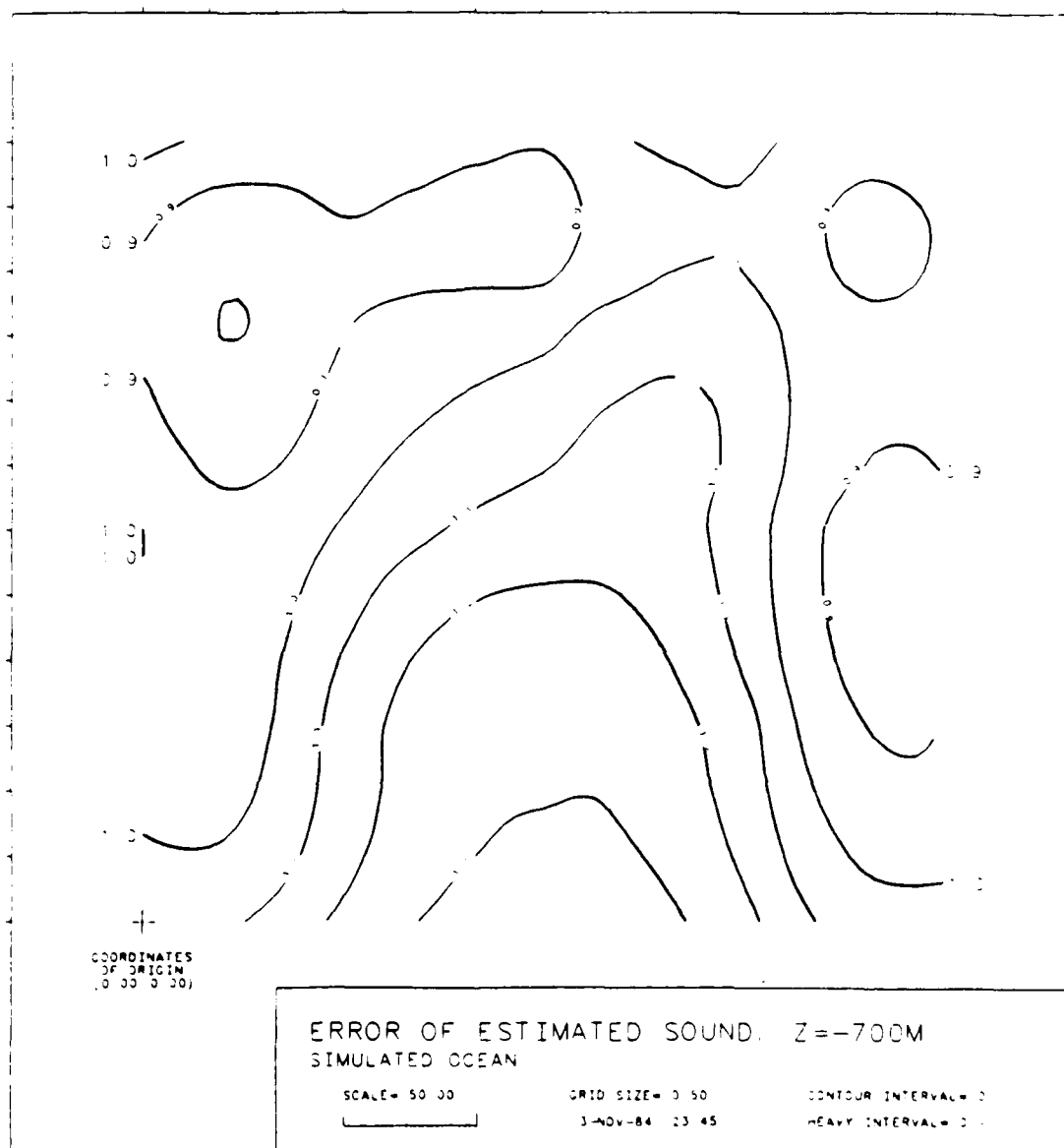
Figure 7.2. Standard deviation, at a depth of 700 m in the tomographic square, of the linear, tomographic sound-speed perturbation estimate in the presence of 200 m (rms) untracked mooring motion. The sound-speed perturbation has an rms value of 2 m/s and a horizontal correlation length of 100 km. The experimental noise is 5 ms (rms). Contour interval is 0.1 m/s.
