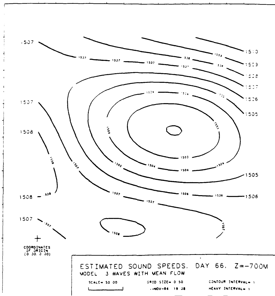
Figure 5.10. Sound-speed map at a depth of 700 m of the optimally estimated wave field in the experimental square on yearday 66. Contour interval is 1 m/s and the reference sound-speed at this depth is 1506 m/s.
