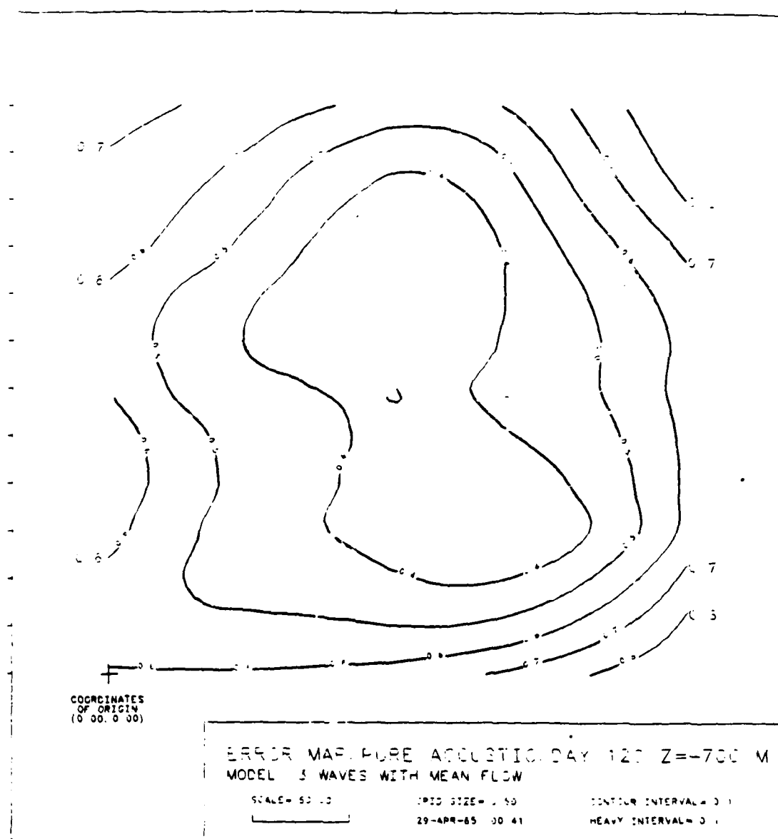
Figure 6.5. Contours of the standard deviation, at a depth of 700 m in the experimental square on yearday 120, of a pure acoustic estimate of the sound-speed perturbations in the wave field. Contour interval is 0.1 m/s.
