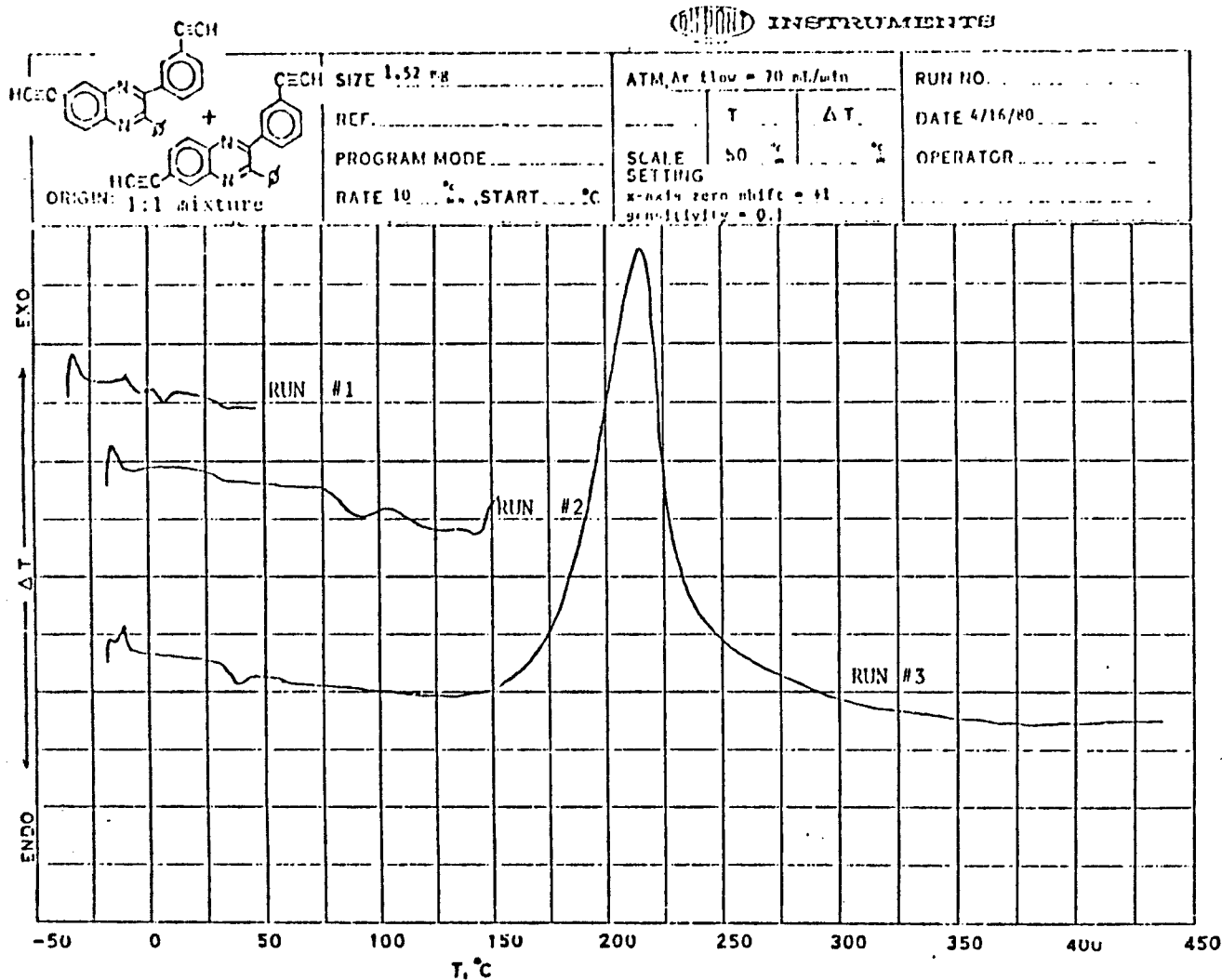
Figure 6. The Composite of Successive Partial DSC Scans of the 1:1 Mixture of 6-ethynyl-3-(3-ethynylphenyl)-2-phenylquinoxaline and 6-ethynyl-2-(3-ethynylphenyl)-3-phenylquinoxaline
