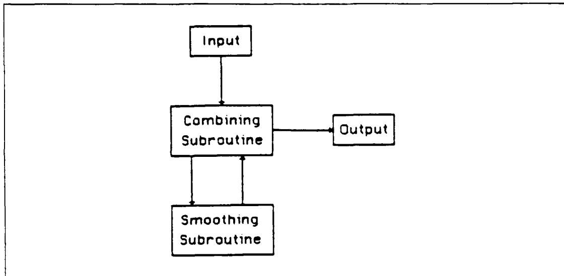
Figure 2.1 Supersmoother Subroutines.
