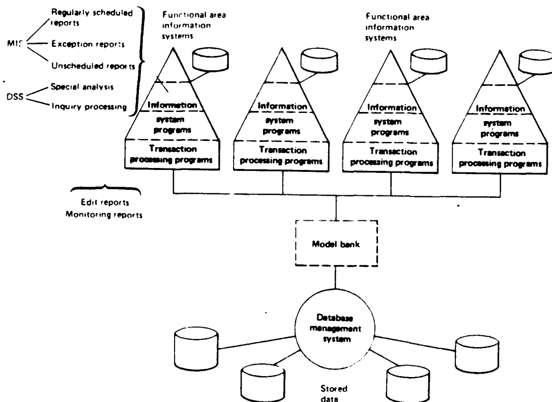
Figure 2. Federation of Information Systems with DBMS
