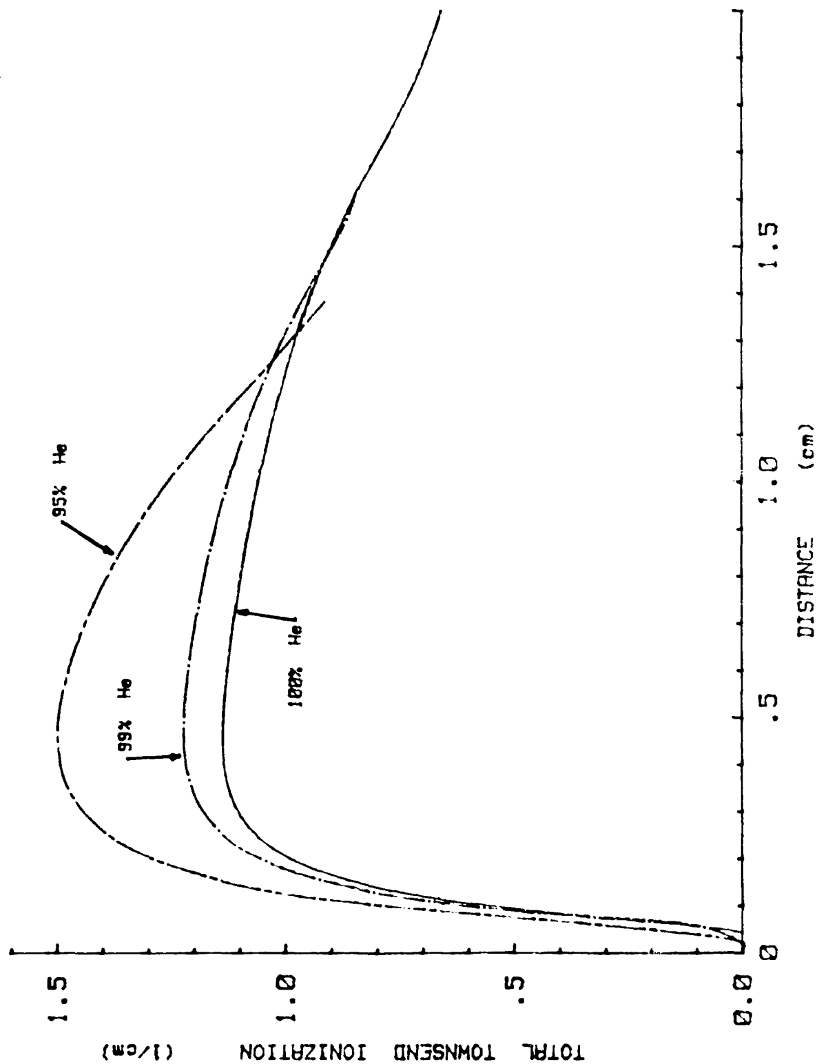
Figure 21 COMPARISON OF TOWNSEND IONIZATION COEFFICIENT IN He/HCl MIXTURES
