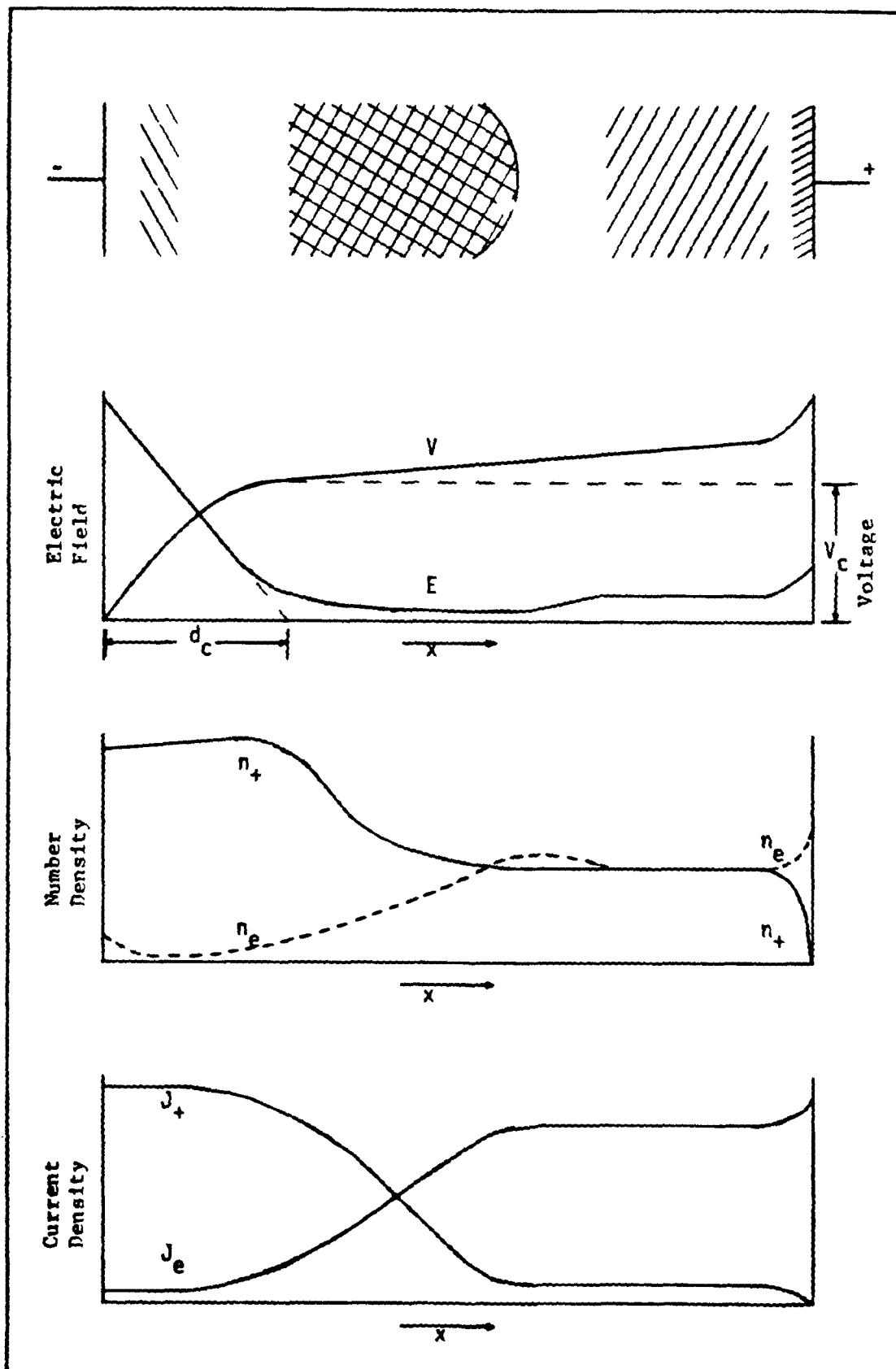
Figure 1 Discharge Parameters as a Function of Discharge Length
