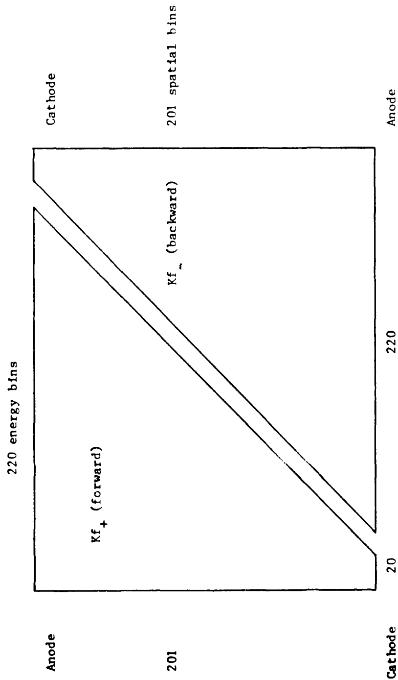
Figure 17 STORAGE ARRAY FOR COLLISION INTEGRAL IN SHEATH CODE
