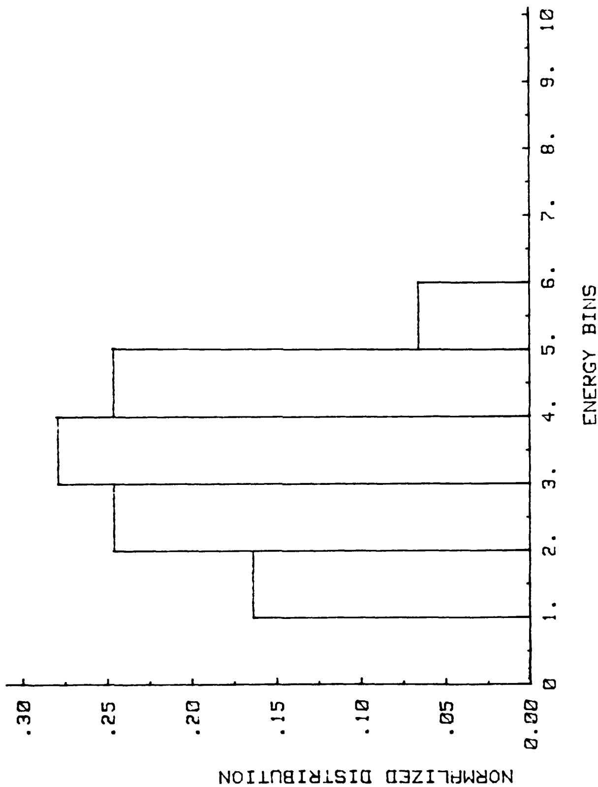
Figure 60 ELECTRON ENERGY DISTRIBUTION AT THE CATHODE
