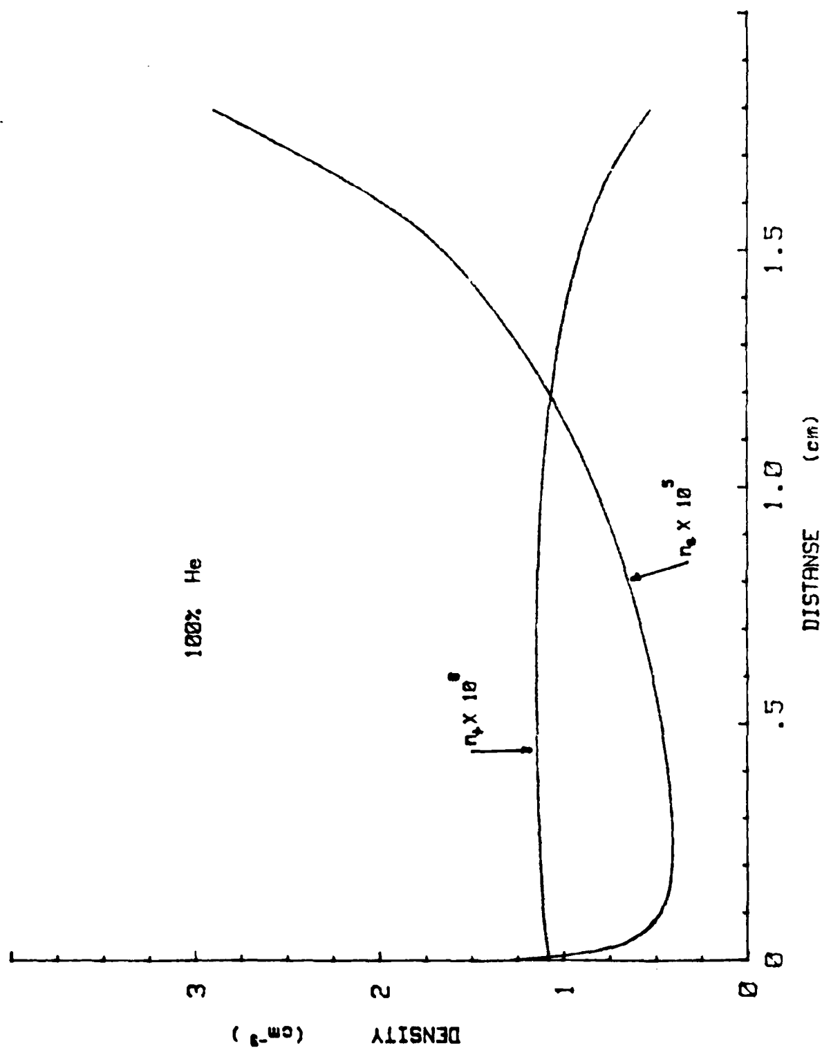
Figure 26 CHARGED PARTICLE DENSITIES IN 100% He
