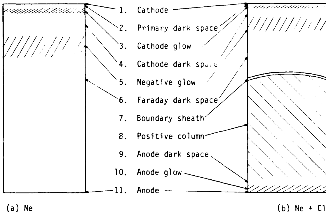
Figure 2 Effect of Adding an Electronegative Gas to a Rare Gas Discharge
