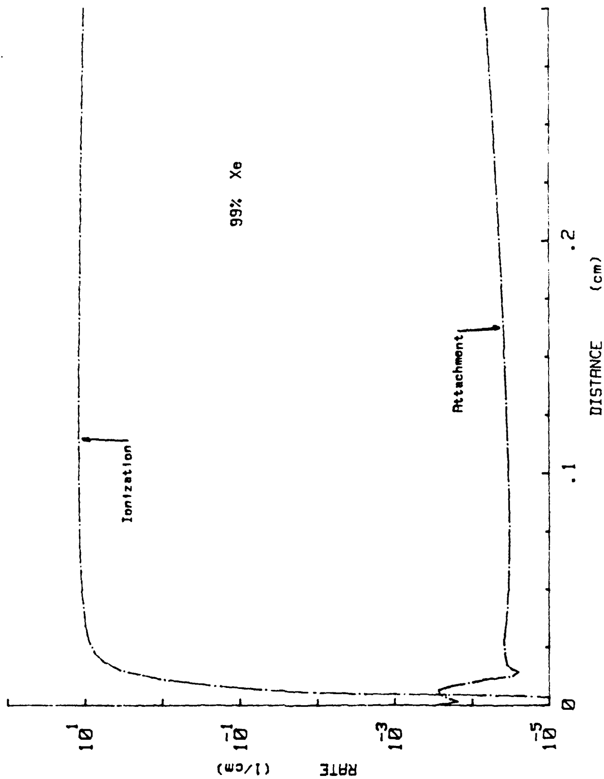
Figure 40 COMPARISON OF IONIZATION AND ATTACHMENT COEFFICIENT IN 99/1 Xe/HCl
