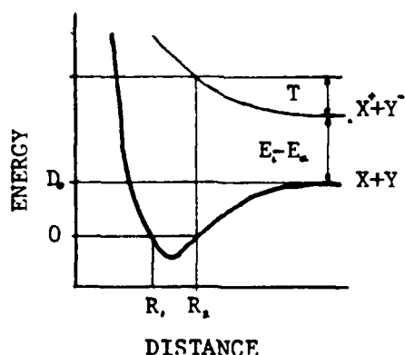
Fig 59. Potential Energy Curve For Ion Pair Formation
