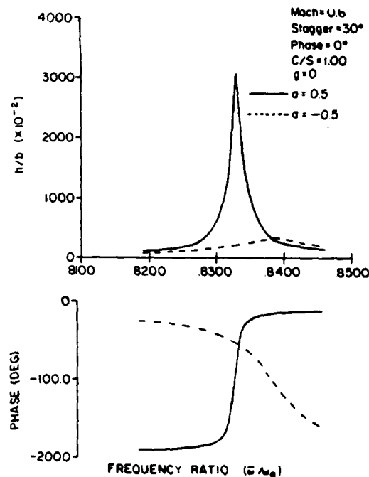
Fig. 14 Effect of elastic axis location on the coupled translational response for (\dot{\omega}/\omega_n) near \omega_n .
