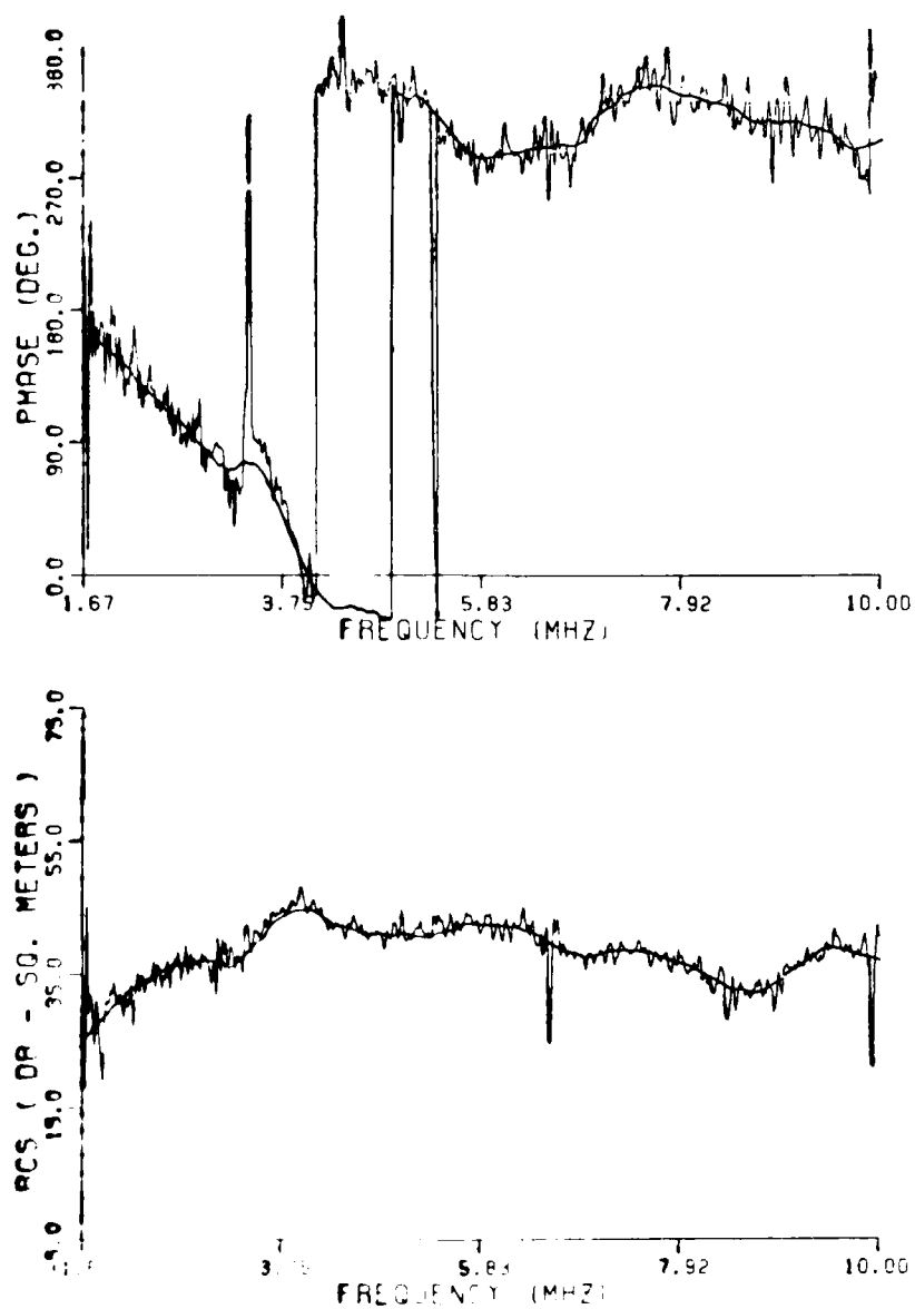
Figure A.10. Ship D at 0 degrees.
