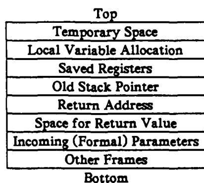
Fig. 2.2. A typical call frame.
