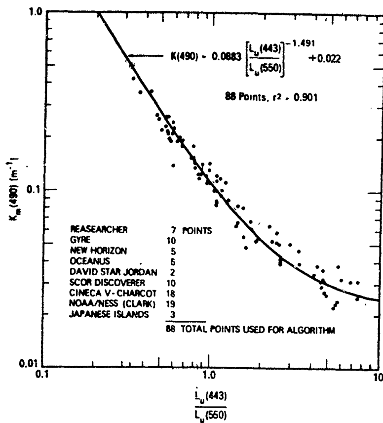
Figure 1. Relationship of the upwelling ratio of 443/550 to the diffuse attenuation coefficient
