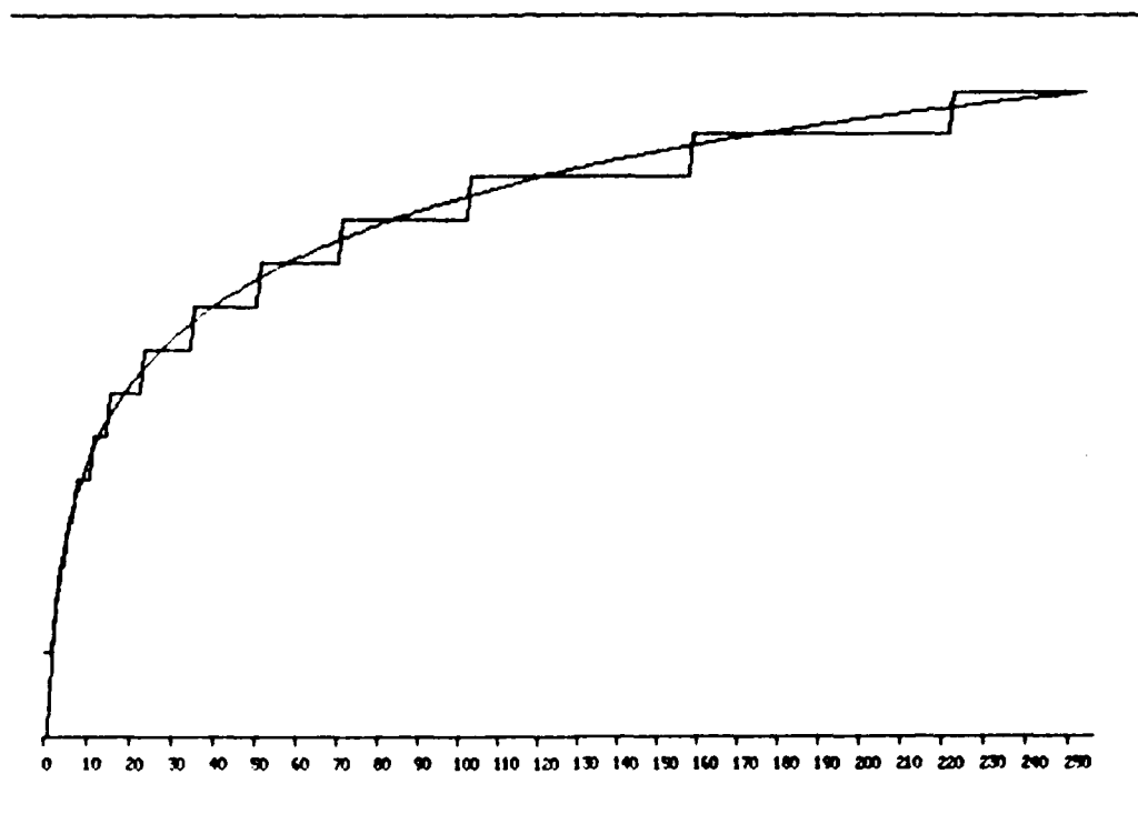
Figure 7: The LOG PLA. (Top) Table used by LOG. The value produced by the PLA is given by the output number associated with the largest number in the IN column not greater than the input. (Bottom) A comparison of the results produced by LOG and the logarithm function. The two plots are normalized to give the same value when the input is 255. The standard error of the LOG PLA over the input range is 0.13.
