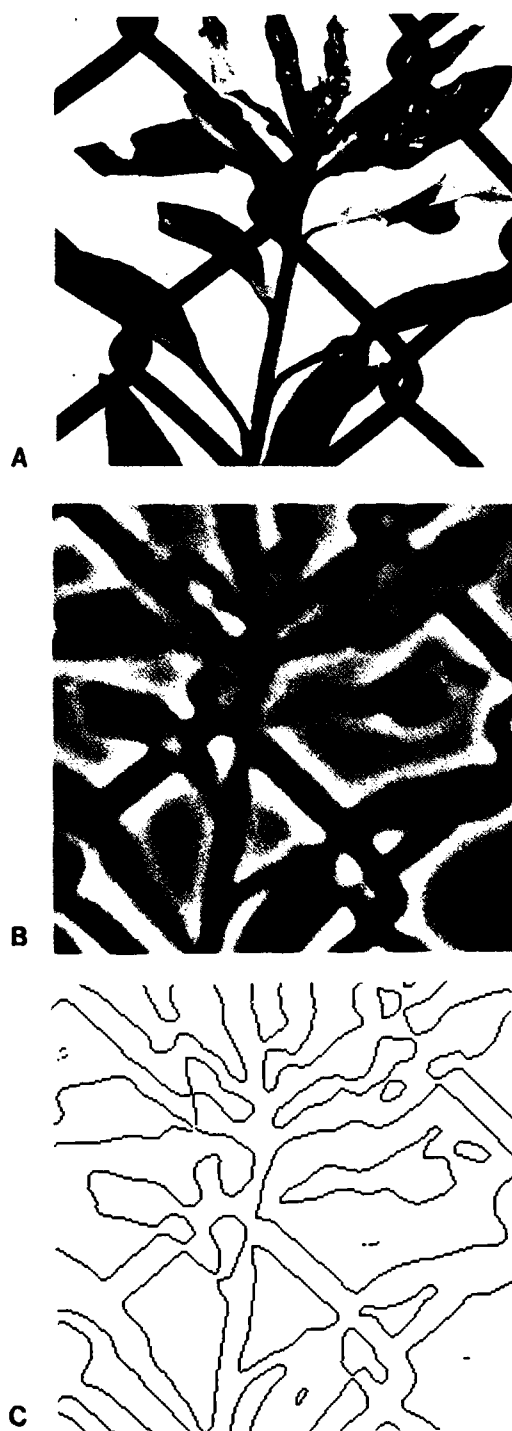
Figure 3: Zero-crossing Example. (A) The original image; (B) After convolution with a \nabla^2 G mask with central-panel width of 12 pixels; (C) Zero-crossings. (This figure is taken from [Marr & Hildreth, 1979])
