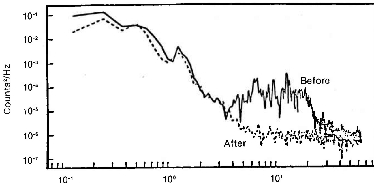
Figure 17(a). Uncorrected power density spectrum of vertical component OBS Suzy data; comparison of OBS spectra recorded before and after ship departure.
