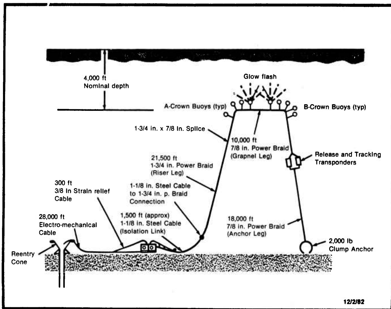
Figure 21. Deployed configuration of the BPP IRR.
