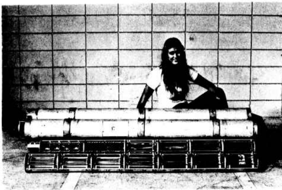
FIGURE 5. Recording package. Two aluminum tubes about 2 m in length contain batteries, electronics, and recorders for recording continuous data from the borehole for up to 75 days unattended.
