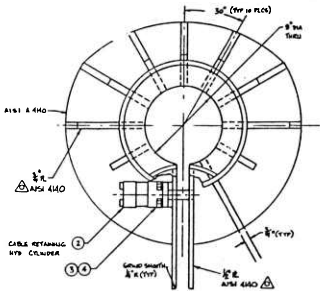
SECTION 2-C
