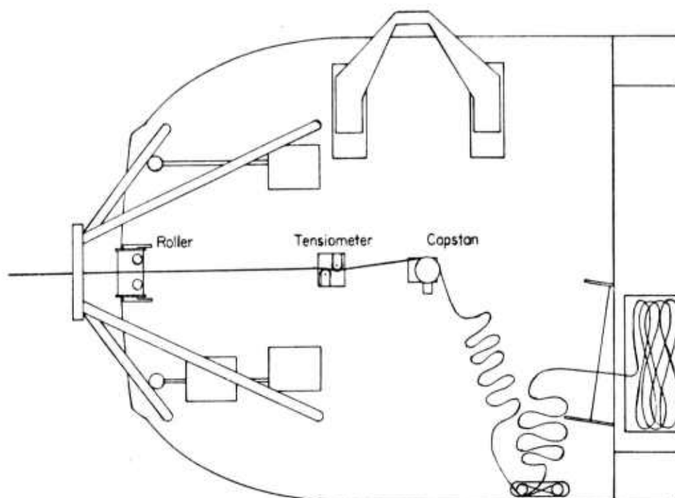
FIGURE 15. Recovery of recording package.
