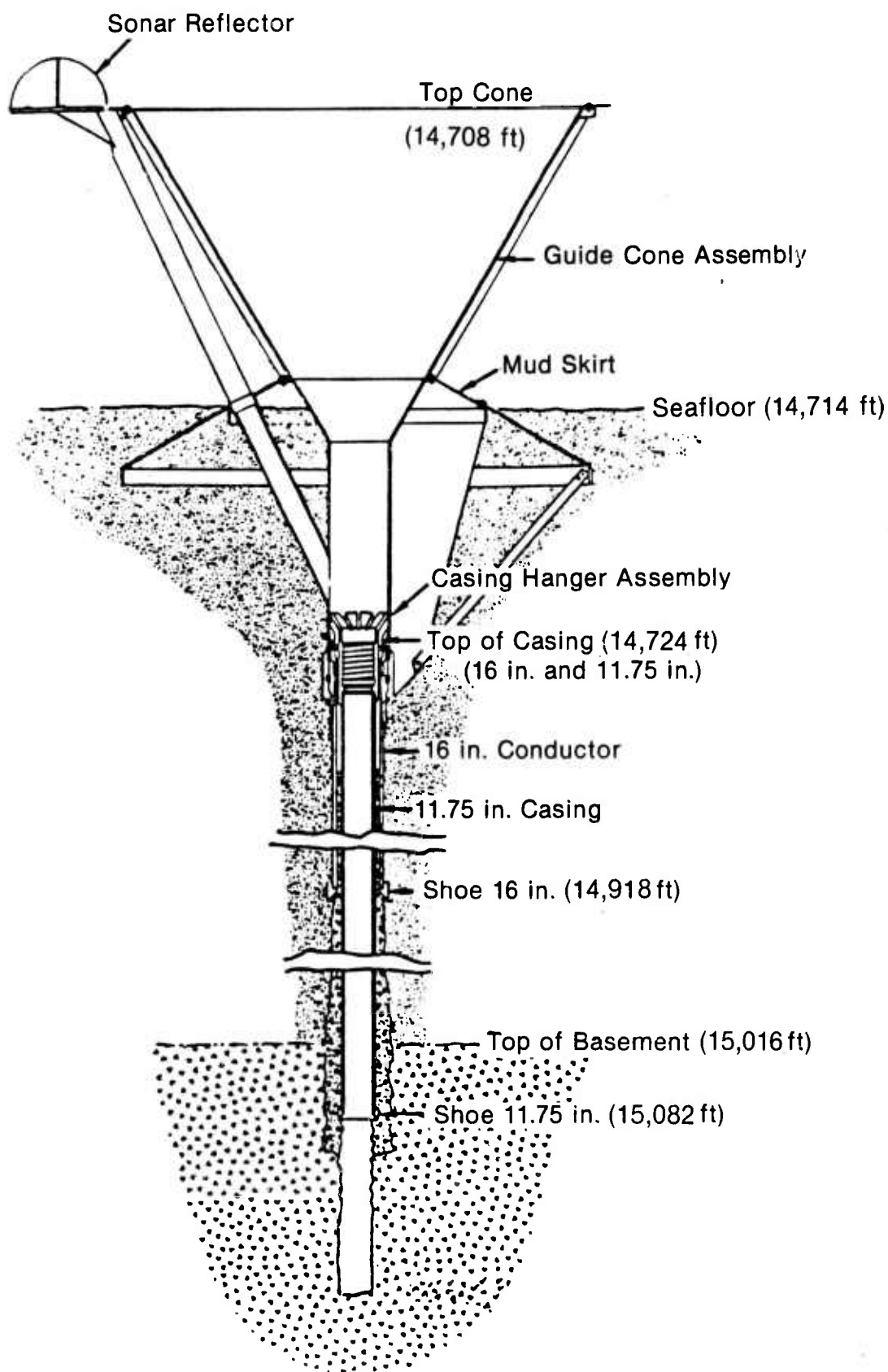
Figure 2. DSDP/MSS reentry cone.
