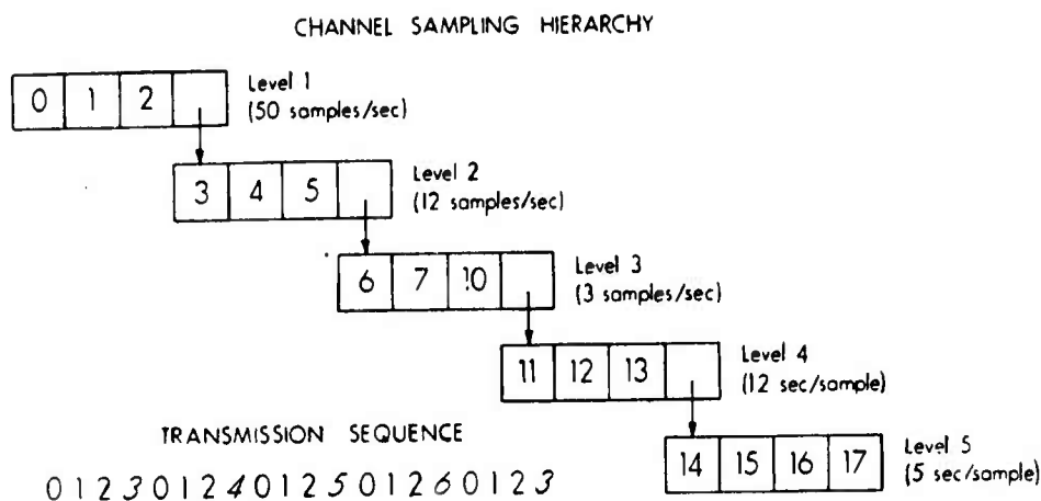
FIGURE 8. Channel sampling hierarchy: 16 channels are sampled at five different rates, from 50 samples/sec to 5 sec/sample.
