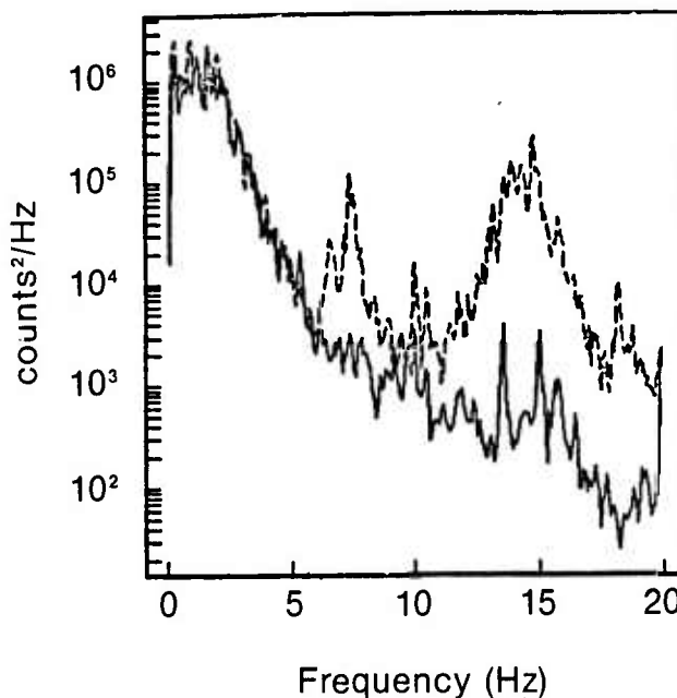
Figure 17(b). Sampling of low ship noise from the MSS in comparison with data observed with CHALLENGER dynamic positioning system in operation.
