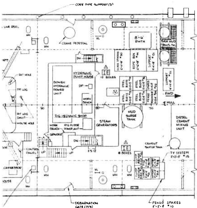
PLAN 4-B IN DECK LAY-OUT AMES 62 THRU 150
