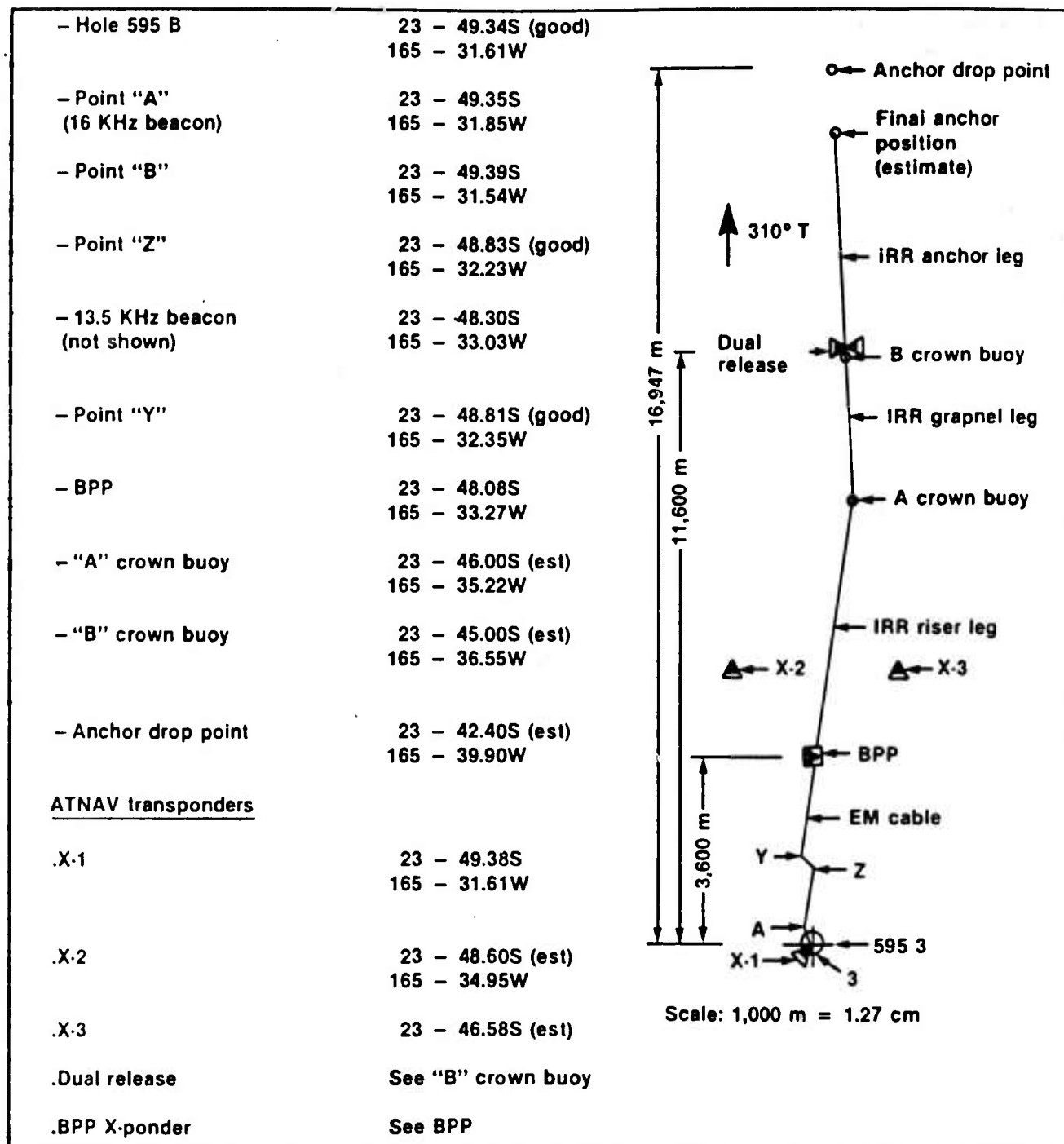
Figure 5. A sketch of the positions of deployed IRR system components, MSS-83.
