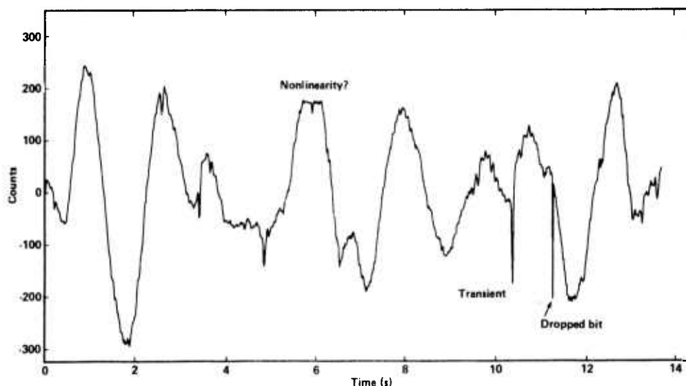
Figure 5. Record sample from channel L1, illustrating characteristics of MSS noise data. Low-frequency (0.2-0.3 Hz) energy dominates the time series. Features typical of those which contribute to noise are the dropped bit near 11 s; the frequent, random, unidirectional transients, such as the one labeled near 10.5 s; and the truncated low-frequency peak centered at 6 s. The last may result from an instrument nonlinearity. Units are digital counts, and positive amplitude corresponds to upward mass movement.
