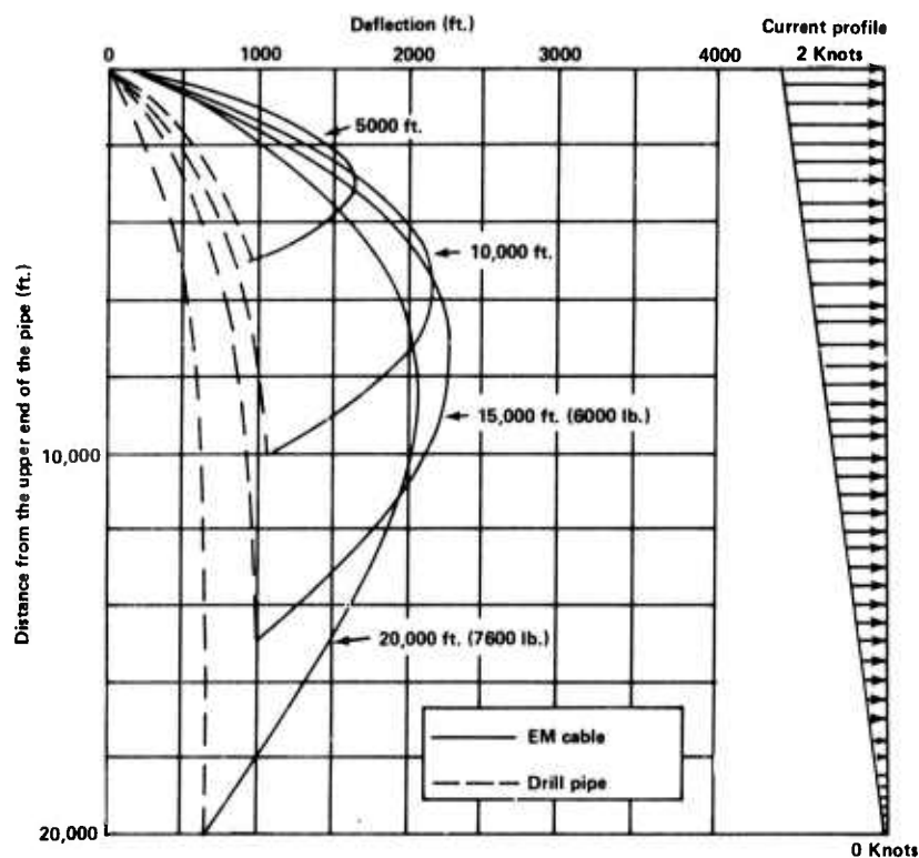
Figure 3. Deflections introduced in the cable and drill pipe by a 2-knot current, which decreases monotonically with depth.
