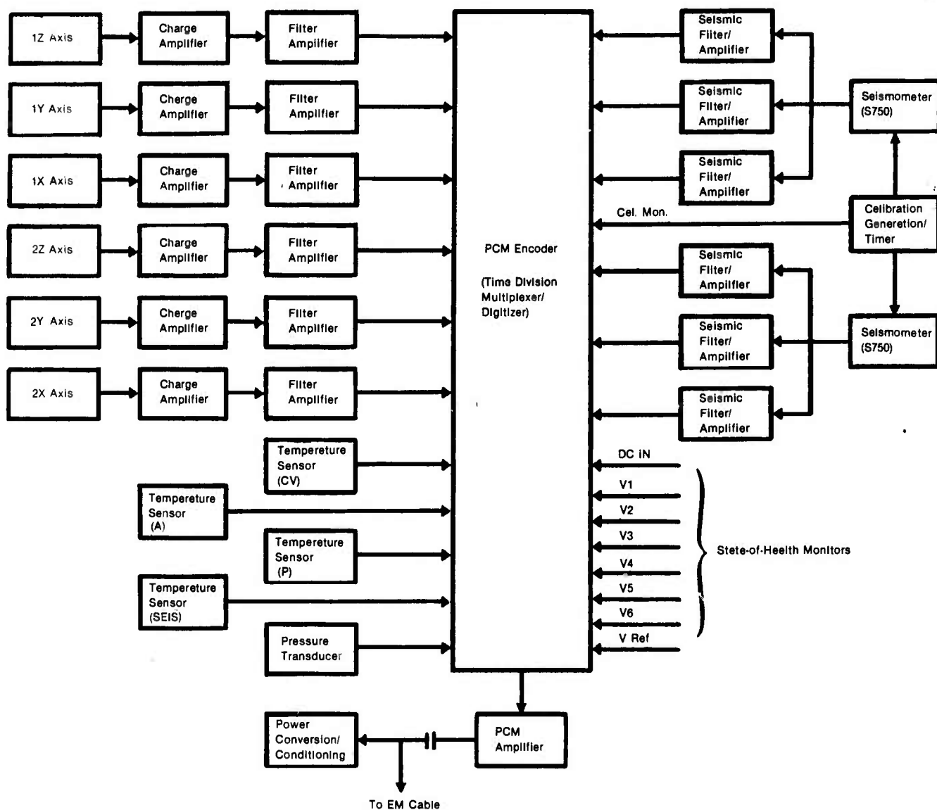
Figure 11. MSS-81 BIP functional block diagram.
