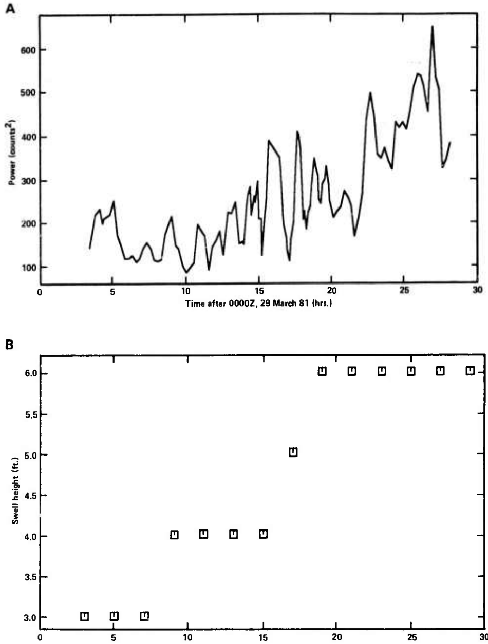
Figure 11. Temporal variations of (A) borehole noise levels and (B) local swell height. The noise level was estimated from integrated, smoothed power densities computed from 13.65 s of uncorrected channel U2 data sampled at approximately 15-min. intervals. A three-point running mean was applied to the integrated values. The swell height was recorded bihourly on the Challenger's deck log.
