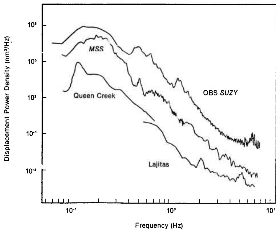
Figure 25. Comparison of subbottom noise levels from OBS Suzy, the MSS, and two land sites (Lajitas, Texas and Queen Creek, Arizona).
