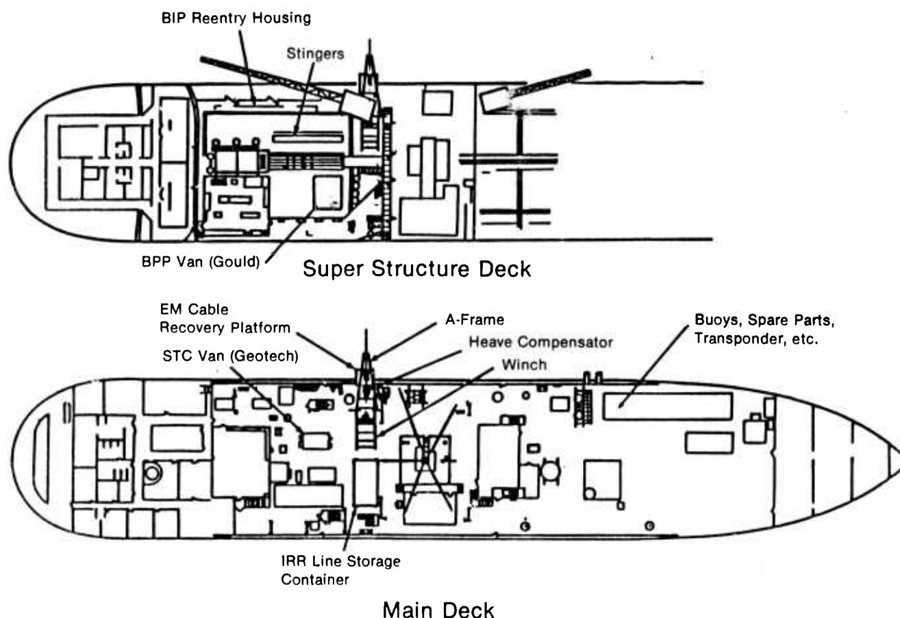
Figure 17. General layout of MSS equipment aboard the GLOMAR CHALLENGER.
