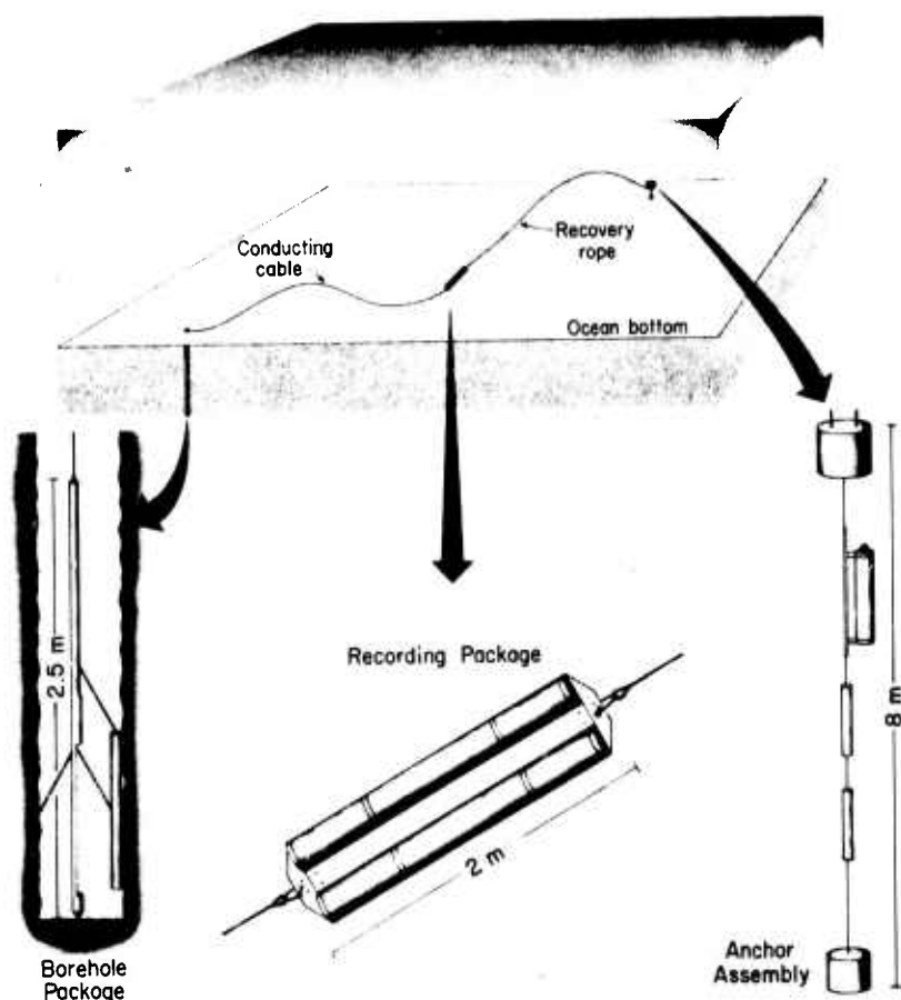
FIGURE 1. The ocean subbottom seismometer system. The borehole package is emplaced in a deep sea drill hole with power transferred to it, and data sent from it, through a conducting cable connected to a recording package. The recording package is attached to a floating rope that is in turn connected to a float-anchor assembly for recovery.
