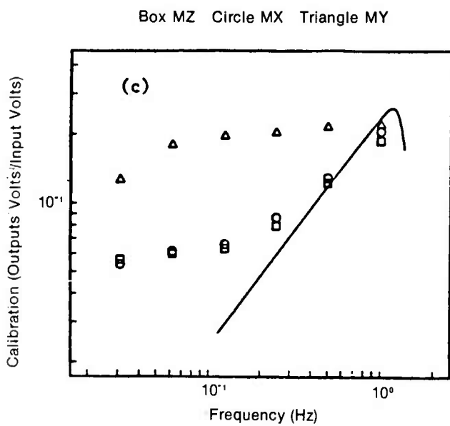
Figure 11. Teledyne calibrations of properly functioning channels.
