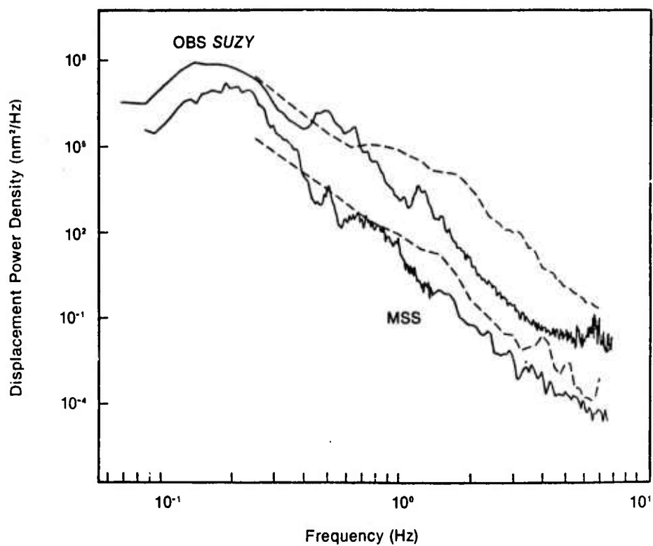
Figure 24. OBS Suzy and MSS high-resolution low-variance estimates of vertical-component ocean-bottom noise.
