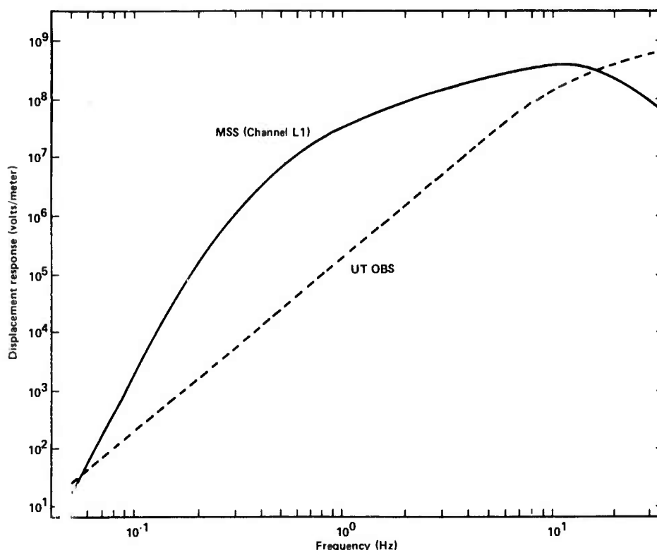
Figure 3. Displacement responses of Leg 78B seismic systems. The MSS employed two vertical-component, short-period, force-feedback, piezoelectric seismometers (Teledyne Geotech model S-700') whose outputs were filtered to prevent aliasing and then digitized at 75 samples/s. The MSS response is peaked near 11 Hz, and falls off at 12 dB/octave toward lower frequencies and at 15 dB/octave to the Nyquist frequency. The University of Texas (UT) ocean-bottom seismometer system consisted of a triaxial set of critically damped, 10-Hz Mark L6 geophones whose outputs were sampled with an 8.352-ms digitizing interval. The UT OBS response increases with frequency at 18 dB/octave up to 10 Hz, and at 6 dB/octave thereafter.
