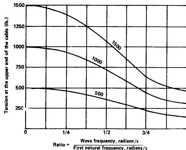
Figure 2. Dynamic tension at the upper end of the cable versus the ratio of the wave frequency to the first natural frequency of the cable for dynamic tensions of 500, 1000, and 1500 lb.
