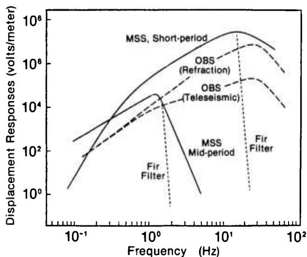
Figure 1. Ocean bottom seismometer selectable frequency responses.
