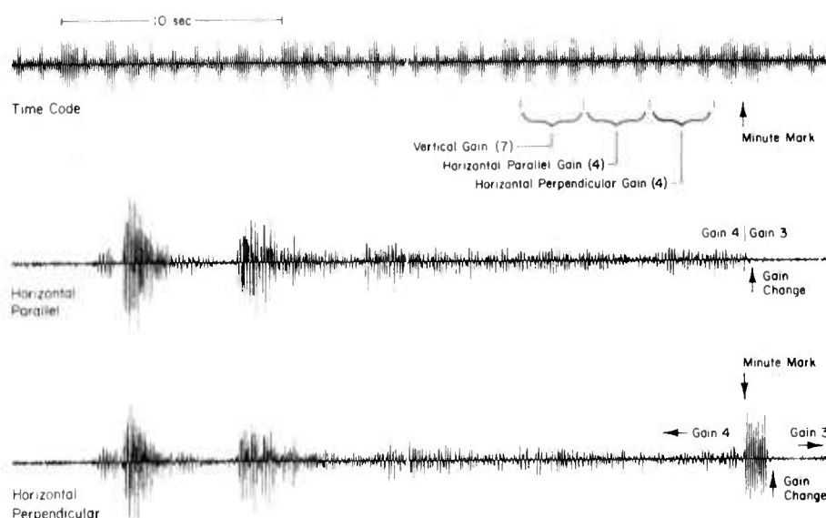
FIGURE 12. Automatic gain ranging. A large change in signal or background level causes the gain to change 12 dB at the next minute mark. The gain is recorded as part of the time code.
