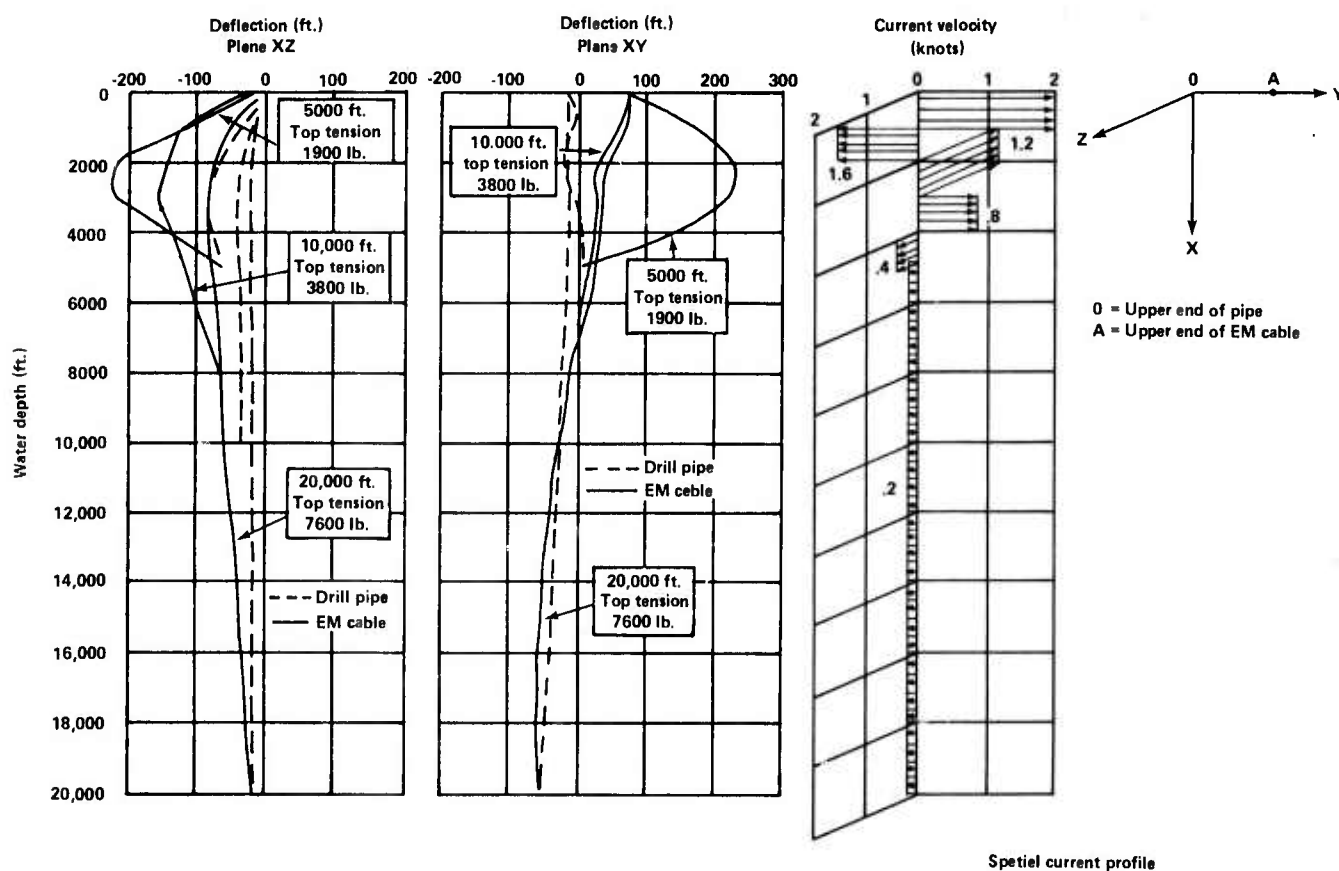
Figure 4. Deflected shape of cable and drill pipe due to a spatial current profile for 5000-, 10,000-, and 20,000-ft. water depths.
