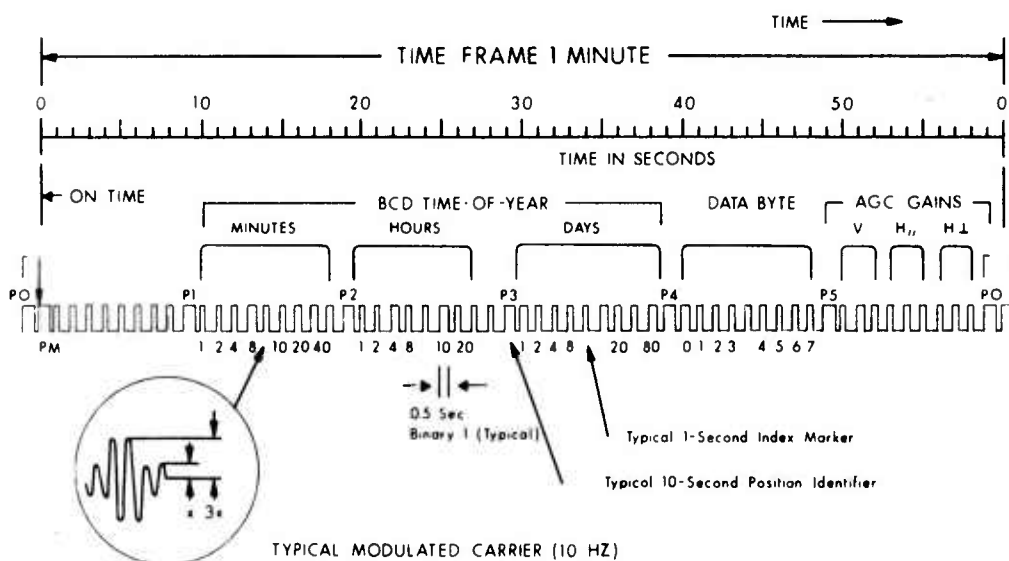
FIGURE 11. Time code. In addition to time, the code contains the recorded geophone gains and the digital data from the borehole package recorded at a rate of one sample/channel/32 min. On playback, the 10 Hz carrier is used in phase lock to control digitization rate.
