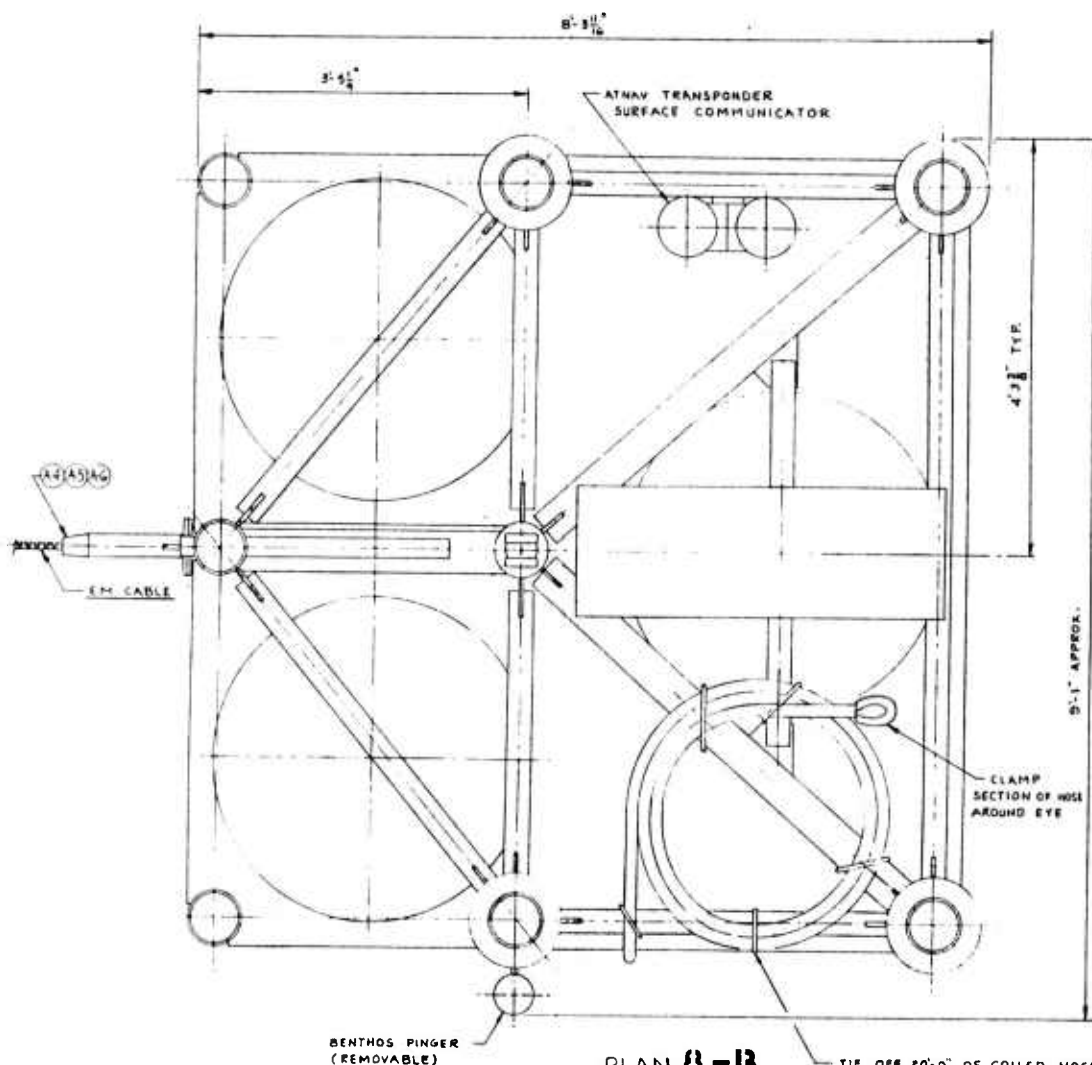
PLAN 8-13
