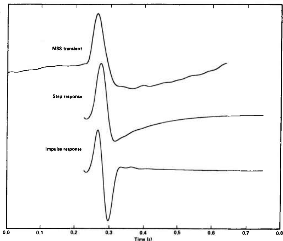
Figure 8. Transient shape compared with the MSS responses to a step and to an impulse in displacement. The transients observed in the MSS data resemble the step responses more closely than the impulse responses, and are taken as such for the purpose of computing the transient-noise spectrum shown in Figure 6.
