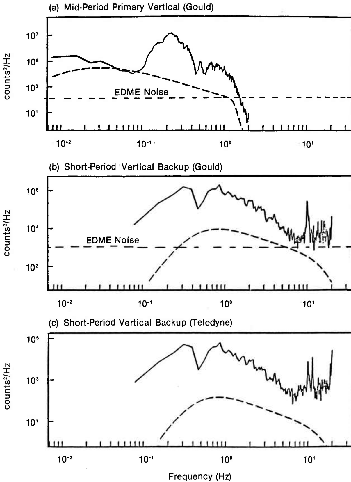
Figure 12. Comparison of power spectral density estimates of simultaneous vertical component Teledyne and Gould data with instrument noise spectra (not corrected for instrument response).
