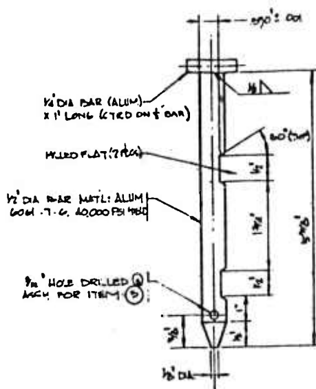
DETAIL 2-D SHEAR PIN (10 REQ'D, INCLUDING SPARES) SCALE: FULL SIZE
