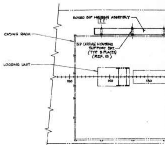
PLAN 9-C
