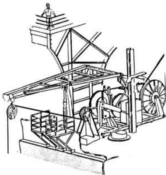
Figure 18. General layout of the EM cable winch, idler sheave, A-frame, sheave, and heave compensator aboard the GLOMAR CHALLENGER.
