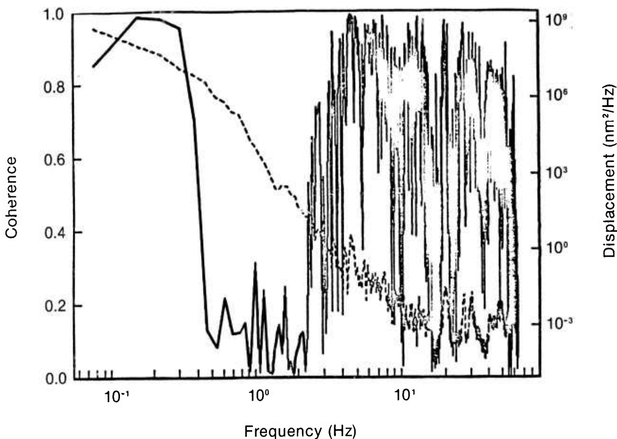
Figure 26. Coherences between OBSs Suzy and Lynn (1 Feb.).
