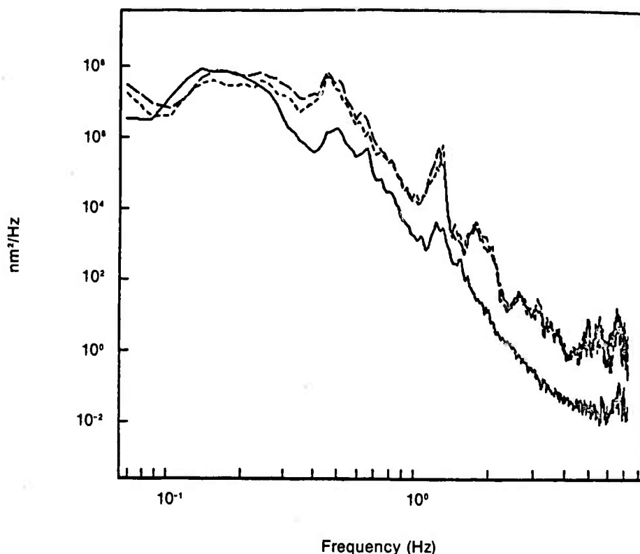
Figure 21. OBS vertical and horizontal noise levels (lesser noise levels are from vertical sensor).
