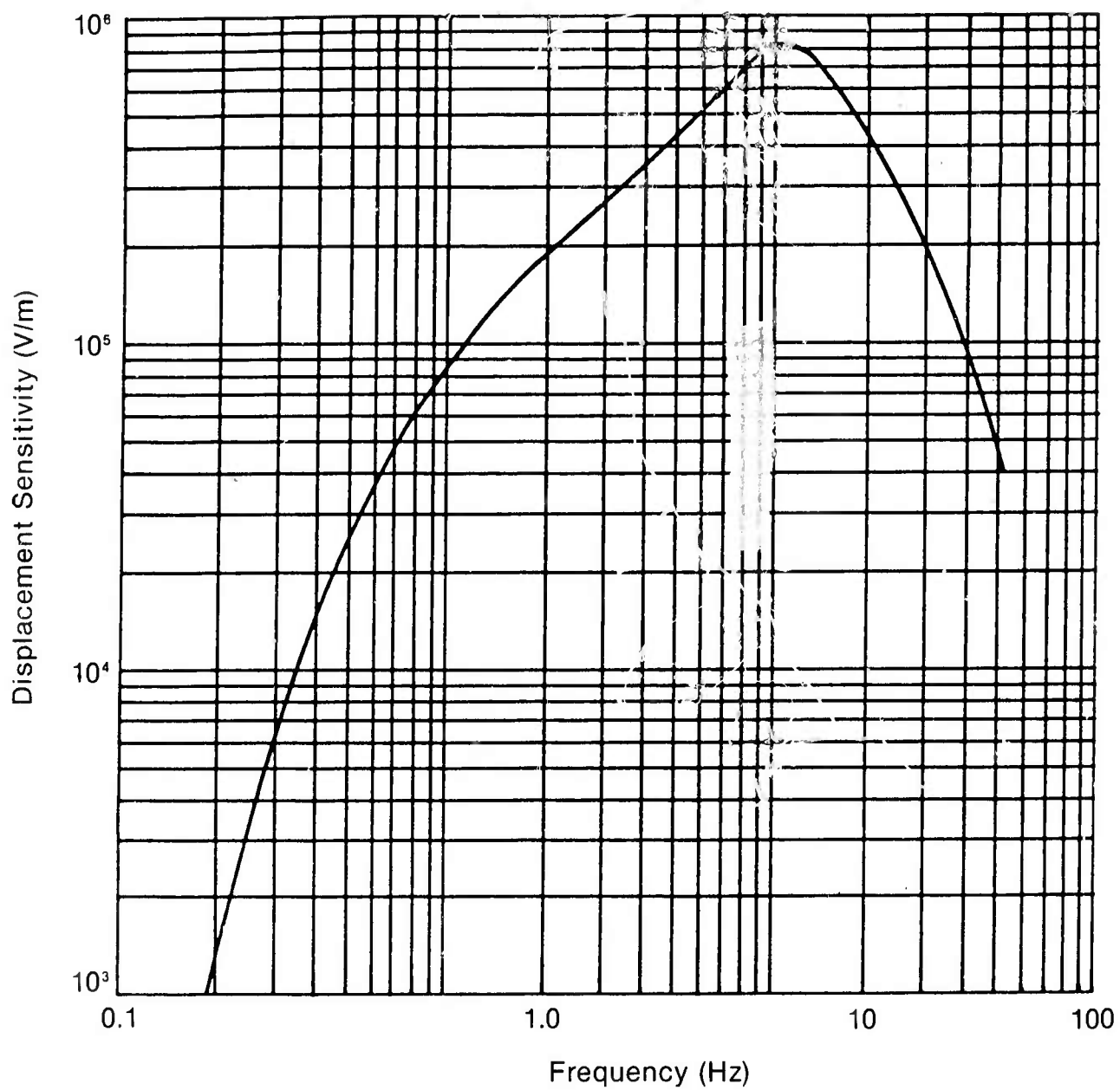
Figure 8. BIP normalized seismic channel frequency response curve.
