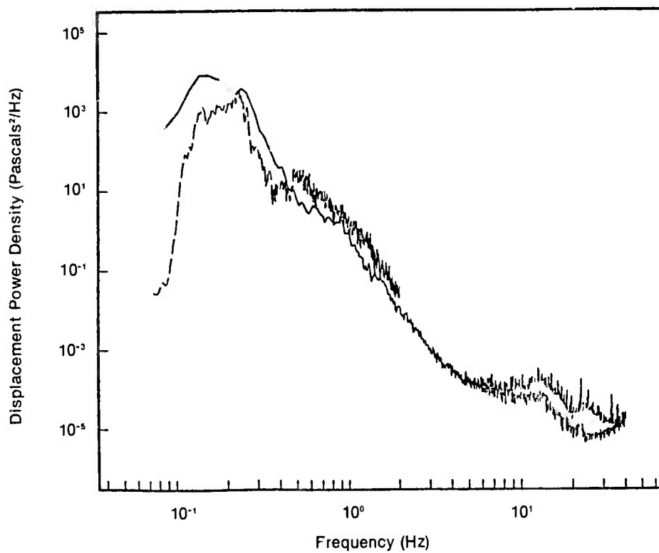
Figure 23. Ocean-bottom pressure spectra of ambient noise from OBS Suzy.
