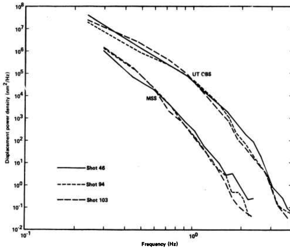
Figure 13. Comparison of corrected UT OBS and MSS noise observations recorded during refraction experiment windows when shots failed to explode. Curves in the upper set were computed from UT OBS data, those in the bottom set from MSS data. The UT OBS was programmed to record a maximum of 40 s per event, but in practice only 34.2 s of data (4096 samples) were available for analysis. Eight segments of 512 time points were used to calculate the estimates for both the UT OBS and MSS data.
