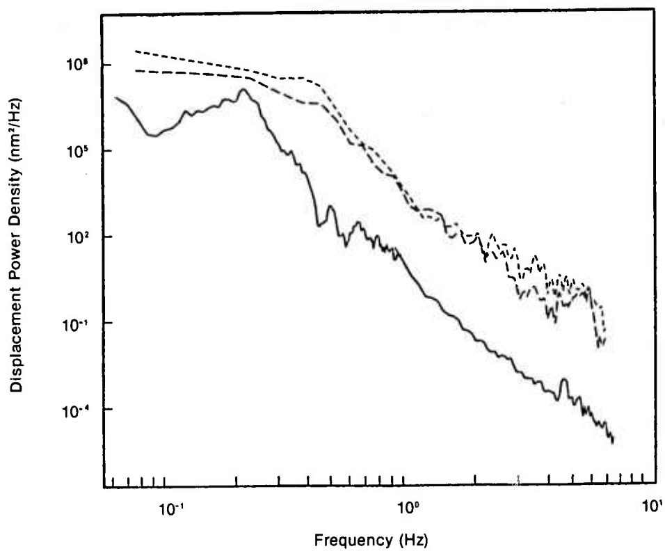
Figure 19. Comparison of horizontal ocean-bottom and borehole noise levels (lower noise level is from borehole).
