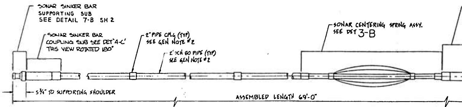
VIEW 3-A SONAR AND SINKER BAR ASSEMBLY N.T.S.
