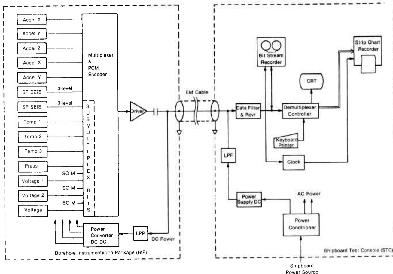
Figure 12. Functional block diagram of the STC (right) and the BIP (left). The EM cable connecting the two instrument subsystems was about 30,000 ft long. (SOH = state of health; 3-level indicates 3 gain bands for the recording.)
