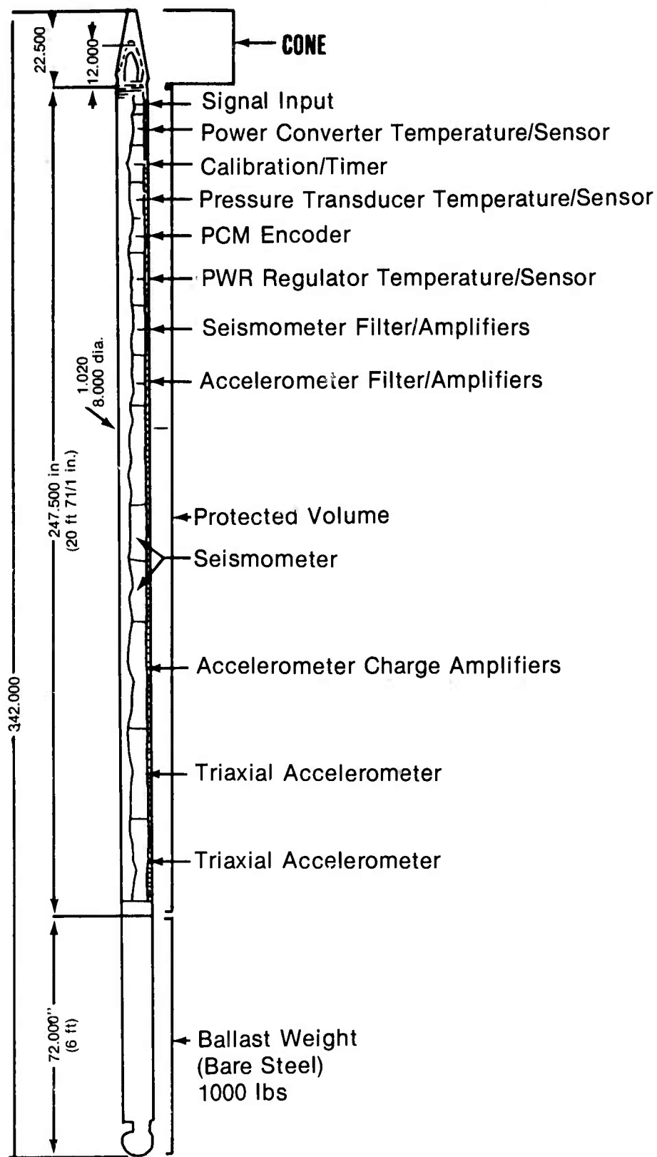
Figure 6. MSS-81 BIP physical layout illustrating components and locations of subassemblies (space is retained for long-period seismometers to be added).
