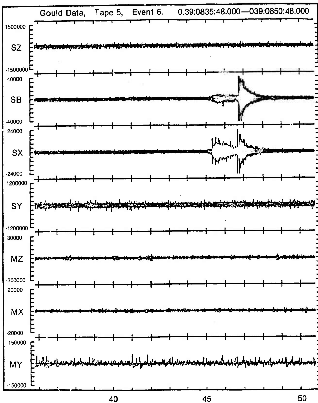
Figure 9. Gould data, tape 5, event 6. Example of multi-channel MSS data from the Gould system. (039:0835:48.000-039:0850:48.000).
