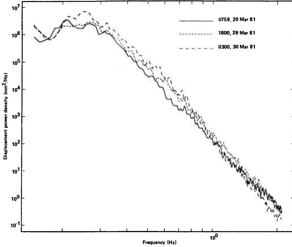
Figure 10. Displacement power densities (in nm 2 /Hz) in Hole 395A at approximately 10-hr. intervals. Each curve was computed from twenty-four 109.2-s samples from channel U2. The spectral shape of the noise was stable over this period, but amplitudes increased with time. Power densities fall at approximately 80 dB/decade beyond the peak at 0.2–0.3 Hz (24 × 8192 points; corrected Channel U2).
