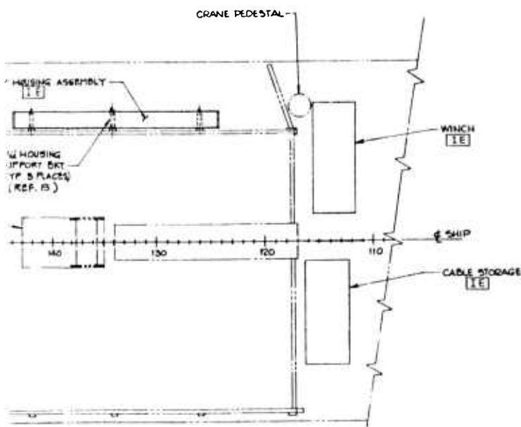
PLAN 9-C E-ENTRY TOOL • MISC. EQPT. STORAGE SCALE 1/8"=1'-0"
