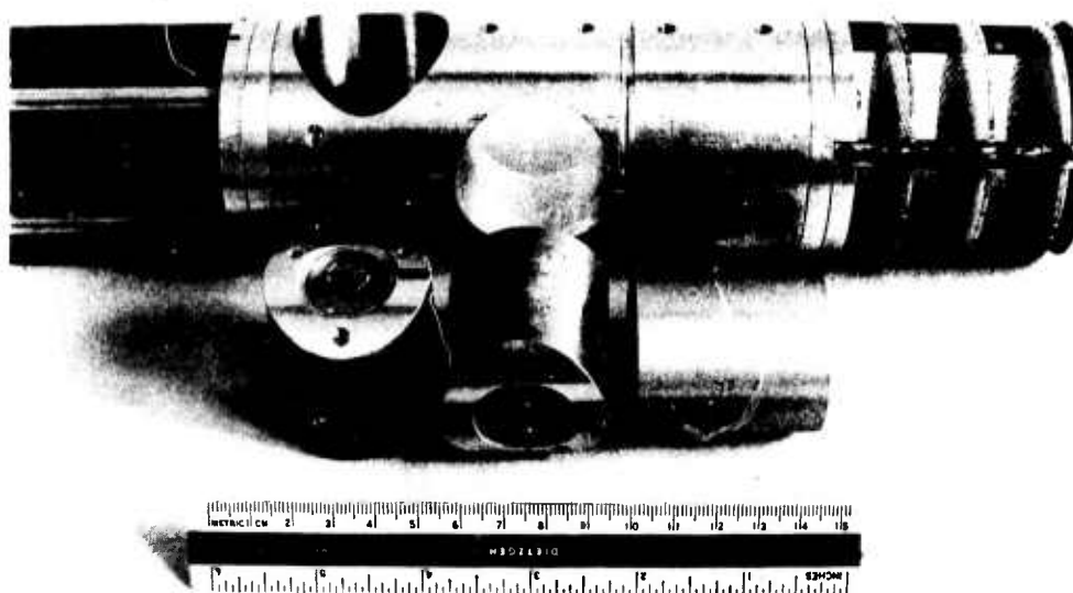
FIGURE 4. Geophones and geophone mounting block in the borehole package. No provision is made for leveling since the geophones will operate up to 5^\circ from vertical and the package tilt can be measured from the tilt meters.
