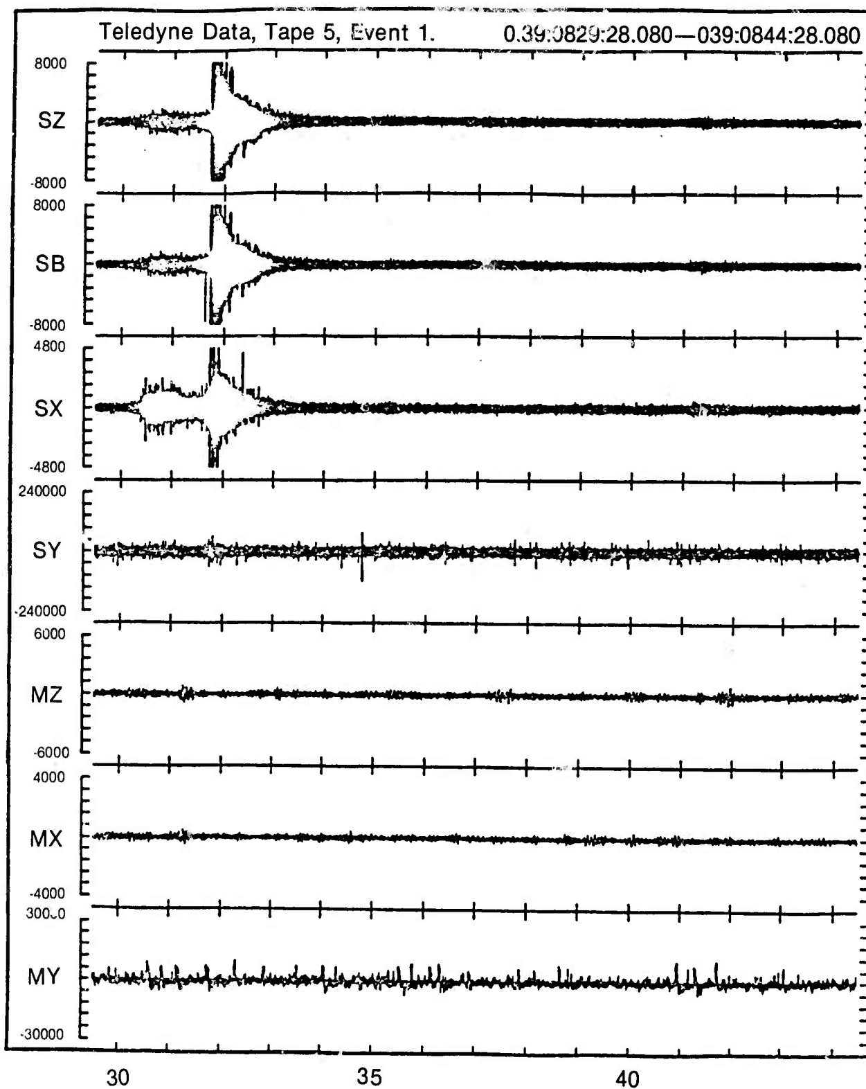
Figure 8. Teledyne data, tape 5, event 1. Example of multi-channel MSS data from the Teledyne system. (039:0829:28.080-039:0844:28.080).
