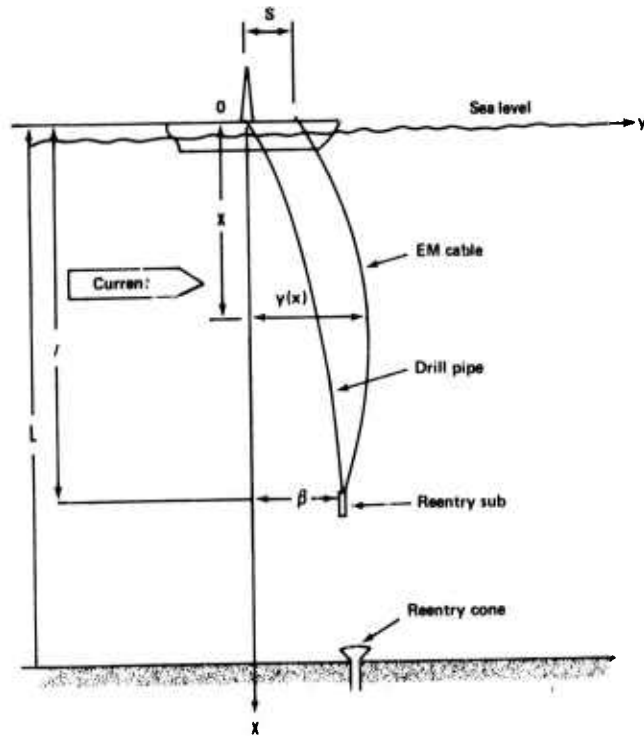
Figure 1. Drill pipe and cable configuration during reentry in the presence of a current. L = water depth, l = drill pipe length, x = point at which deflection is measured, s = initial offset between EM cable and drill pipe, y = deflection of cable, and \beta = deflection of drill pipe.
