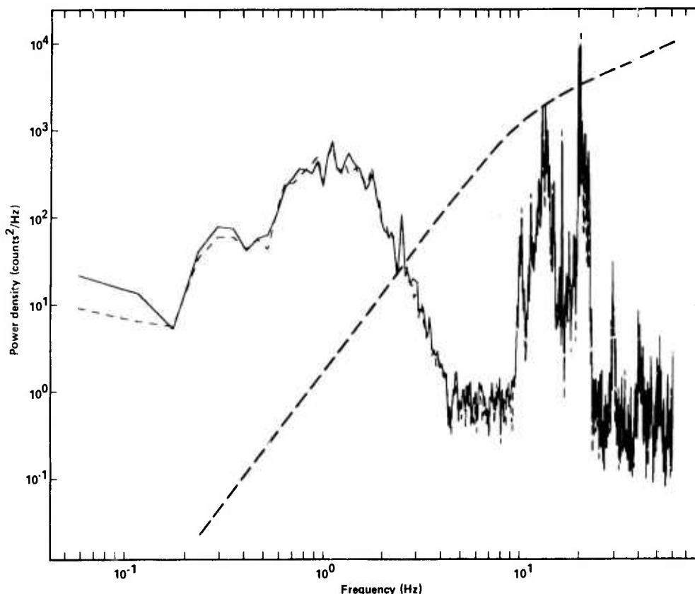
Figure 9. Uncorrected UT OBS power densities. Spectra were computed from eleven 17.1-s segments obtained from six 34.2-s noise samples recorded over a 75-min. period. The large amplitudes between 10 and 25 Hz may be the result of resonance of the OBS frame, and the flat portions above 4 Hz and below 0.18 Hz are probably imposed by instrument noise. Spectra between 0.18 and 4 Hz are thought to estimate reliably the ambient noise levels on the seafloor.
