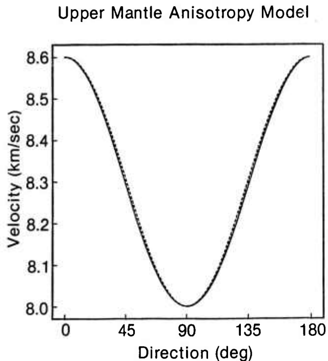
Figure 10. Solid line is the group velocity function for a specific model of upper mantle anisotropy ( \Gamma_{1111} = 73.96 , \Gamma_{2222} = 64.00 , \Gamma_{1212} = 21.716 , \Gamma_{1122} = 25.55 , \Gamma_{1313} = 13.57 \text{ km}^2\text{sec}^{-2} ). Dashed line is the calculated group velocity curve using the Backus approximation applied to this model ( v^2 = 68.98 + 4.98 \cos 2\theta ).
