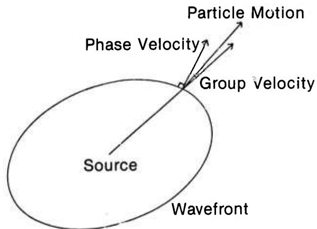
Figure 2. Wavefront from point source in homogeneous, anisotropic medium. At a point on the wavefront, the group velocity vector, phase velocity vector, and particle motion vector all point in different directions.
