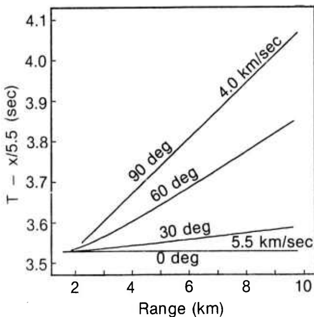
Figure 8. Travel time for the Stephen anisotropy model along lines at various angles from the fast direction in the anisotropy. Curves start at the closest range at which head waves are generated. Travel-times have been reduced at 5.5 km/sec, the velocity of the fast direction in the anisotropic medium. Travel-time curves at azimuths of 30 and 60 degrees are slightly curved, while travel-time curves at 0 and 90 degrees (corresponding to anisotropic symmetry axes) are straight.
