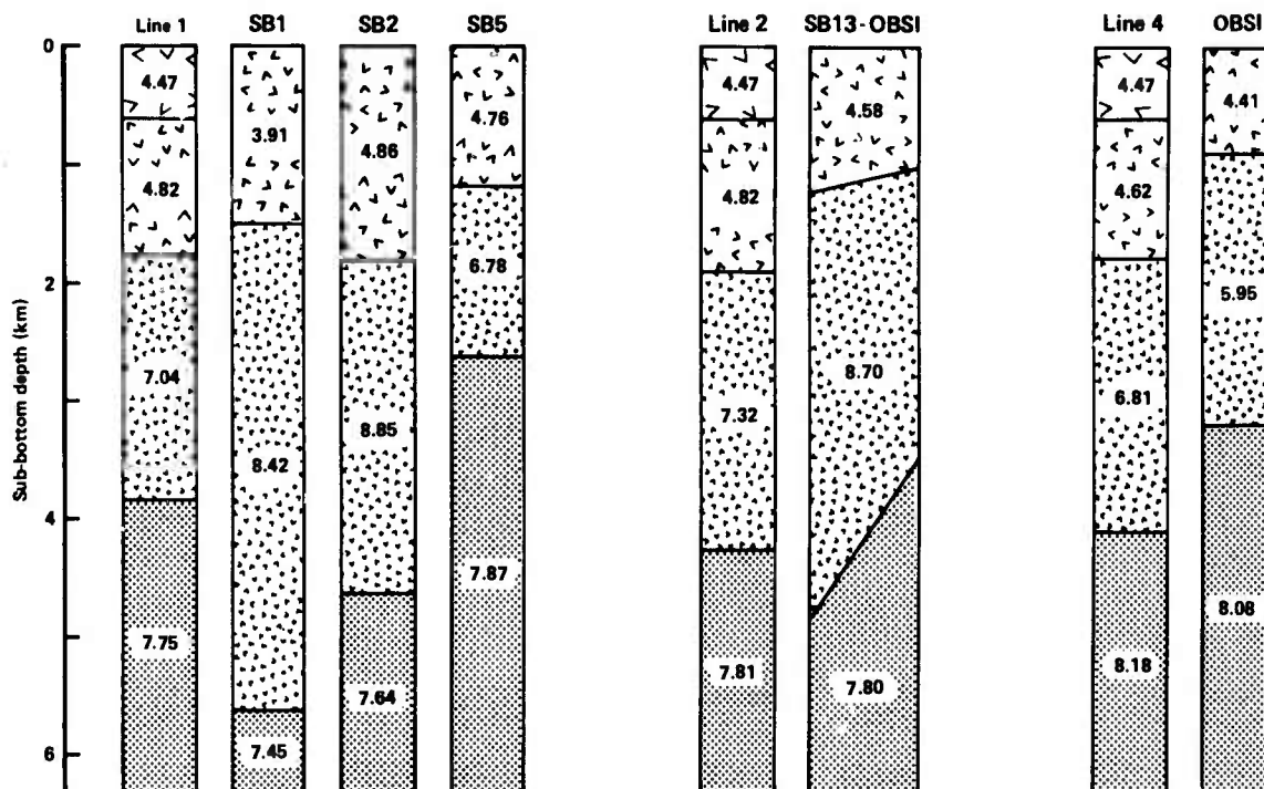
Figure 7. Comparison of crustal velocity structure near Site 395 determined from the DARPA borehole seismometer experiment (Lines 1, 2, and 4) with co-located seismic refraction profiles run by Hussong et al. (1979) using sonobuoys and OBS's. Layer velocities in km/s.
