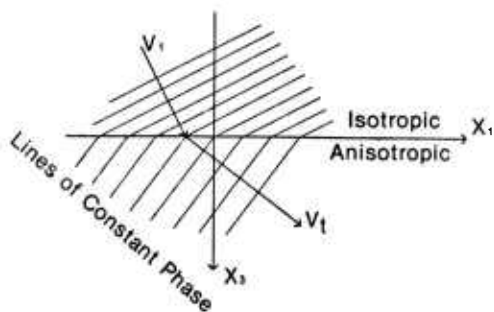
Figure 5(a). Plane p-wave striking an interface between an isotropic layer and an anisotropic layer. Vectors V_i and V_t do not represent rays, but are phase velocity vectors.
