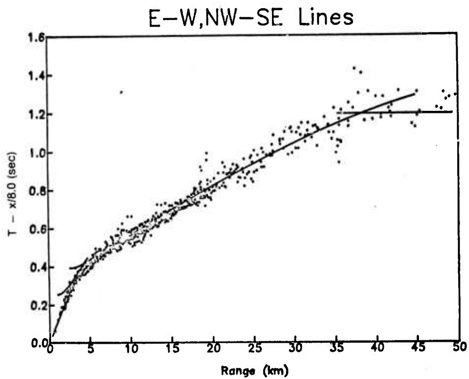
Figure 23. Travel-time curves calculated from model shown in Figure 22 superimposed on the data for a. N-S, NE-SW azimuths b. E-W, NW-SE azimuths
