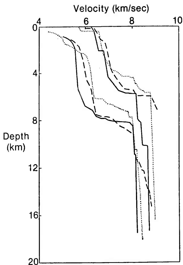
Figure 7. The results of joint linear extremal \tau - p analysis on Lines 4 (dashed line), 5a and 5b (continuous line).
