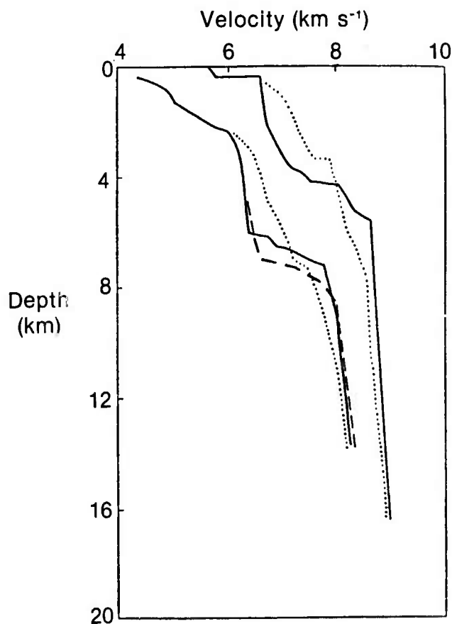
Figure 6. Extremal bounds obtained from Line 4 based on (a) first arrival times alone (dotted line); (b) first arrival times plus an estimate of the lower crust/upper mantle cross-over point (dashed line, only shown where different from (c)); as (b) plus an estimate of the mantle reflection/refraction cusp (solid line).
