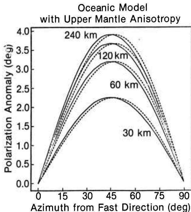
Figure 12. Calculated polarization anomalies for an oceanic model with 6 km of 1.5 km/sec water above 6 km of 6 km/sec crust above an anisotropic upper mantle. Source was assumed to be at surface of water; receiver was assumed to be at surface of crust. Anisotropy model calculations were done as in Figure 11.
