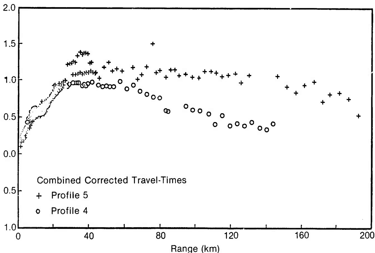
Figure 5. Combined first arrival picks (reduced to 8 \text{ km sec}^{-1} ) from lines 4 and 5 to illustrate the differences in upper mantle arrival times.
