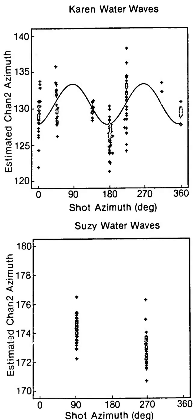
Figure 25. (a) Estimated azimuth of channel 2 (first horizontal) for OBS Karen based on polarization analysis of unclipped direct water waves. The curve shown is the best least squares fit resulting from allowing the ratio of the gains of the two OBS horizontal components to vary. For the curve shown, the true channel 2 azimuth is 130.5 degrees and channel 3 (second horizontal) is 10% more sensitive than channel 2. (b) Estimated azimuth of channel 2 for OBS Suzy.
