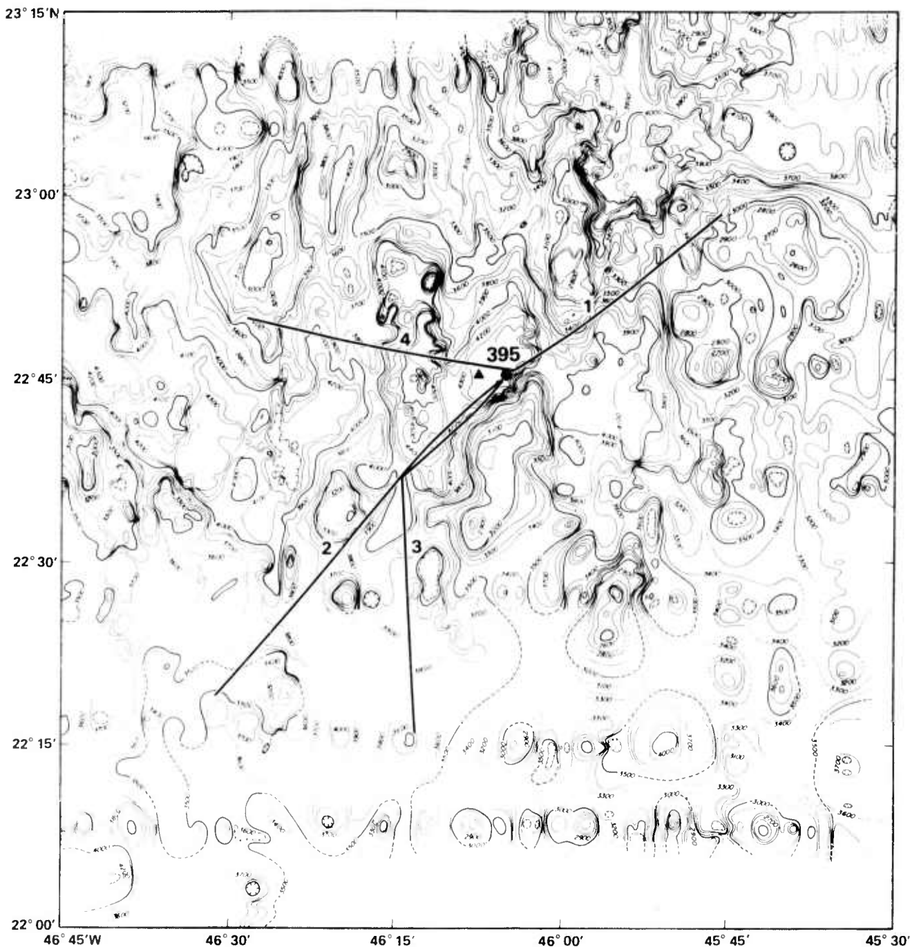
Figure 1. Location of the seismic instrumentation used in the Leg 78B noise experiment. The borehole instrumentation package of the Marine Seismic System (MSS) rested unclamped at the bottom of Hole 395A (22°45.35'N, 46°04.91'W), drilled five years earlier on Leg 45. The ocean-bottom seismometer (OBS) referred to here, one of four deployed during Leg 78B, was approximately 1 to 2 km west of Hole 395A. The OBS launch point (22°45.50'N, 46°05.43'W) is shown as a triangle. Depths shown in corrected meters.
