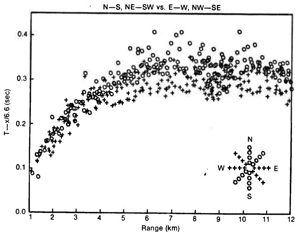
Figure 19. A comparison of N-S, NE-SW arrivals (circles) with E-W, NW-SE arrivals (crosses) at ranges of 1 to 12 km. Arrivals from rays entering the sea floor at depths deeper than 5400 m have been eliminated because of scatter in the data and uncertainties in applying topographic corrections.
