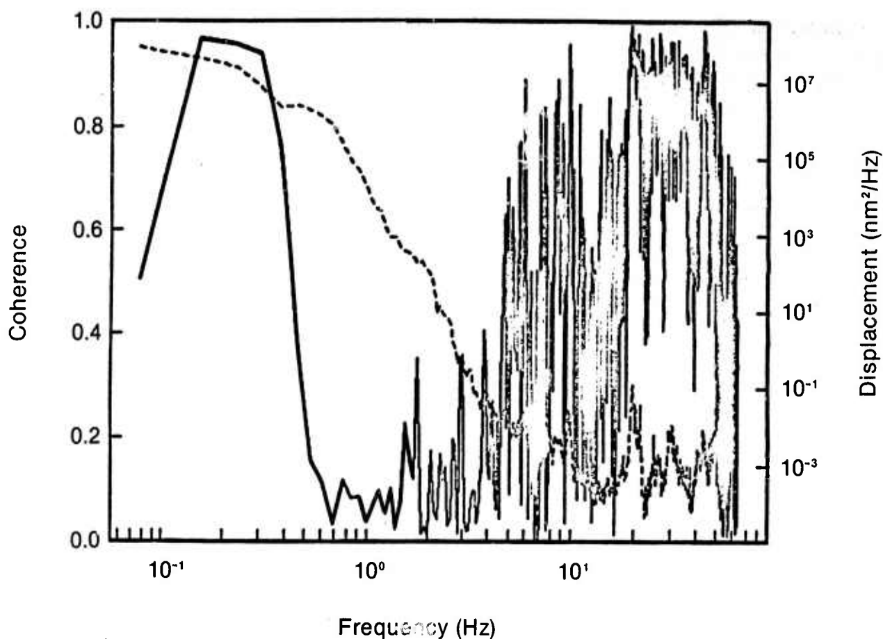
Figure 27. Coherence between OBSs Karen and Jean (3 Feb.).
