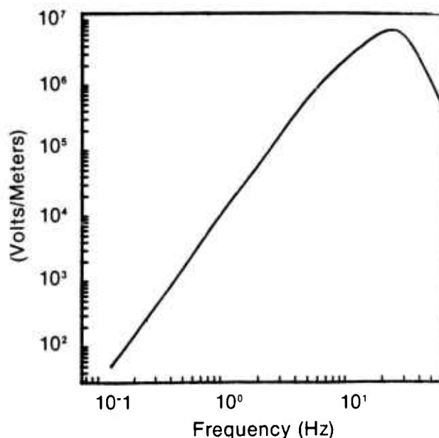
Figure 16. OBS frequency response.
