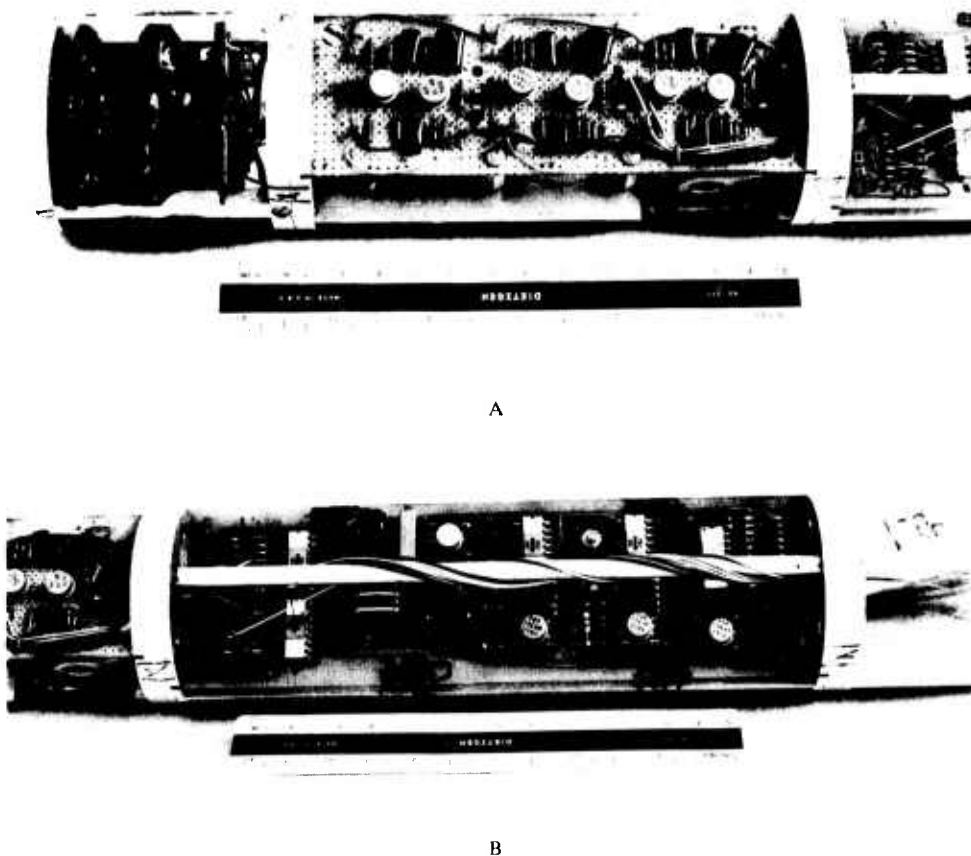
FIGURE 3. A and B. Borehole package electronics showing modular design for ease of replacement and modification.
