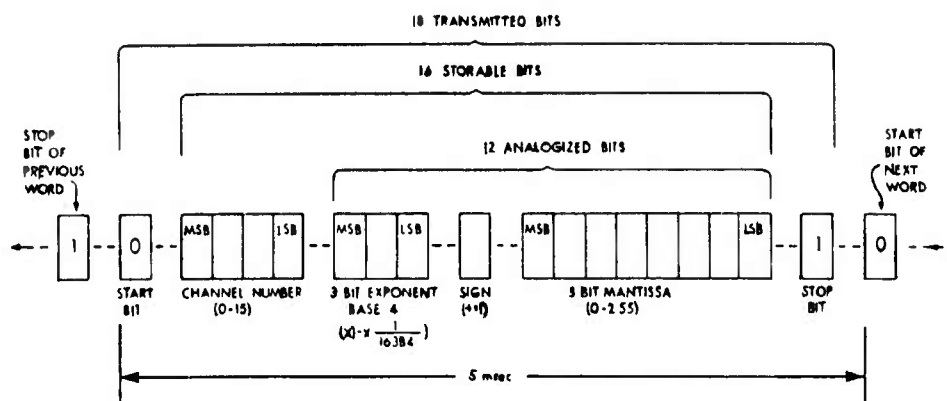
FIGURE 10. Transmission sequence. This sequence is sent up the wire at 200 samples/sec or 3200 bits/sec. The rate is limited by the power available to the system.
