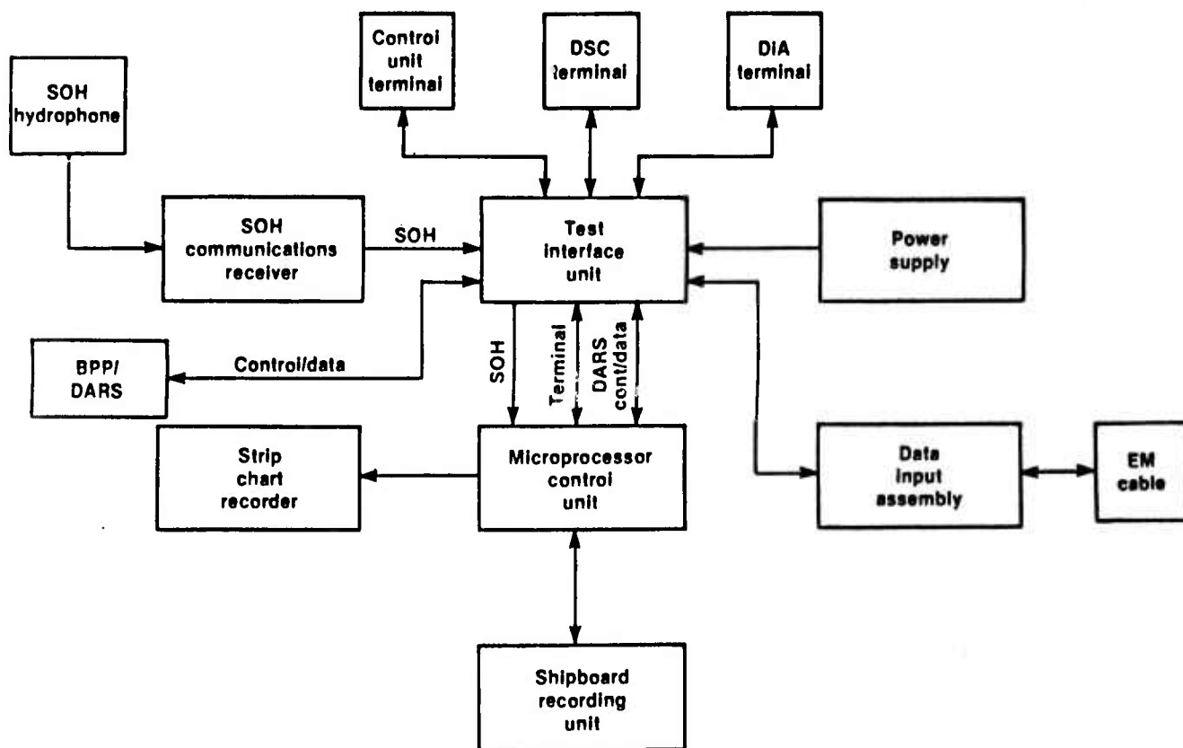
Figure 15. Test equipment rack block diagram.
