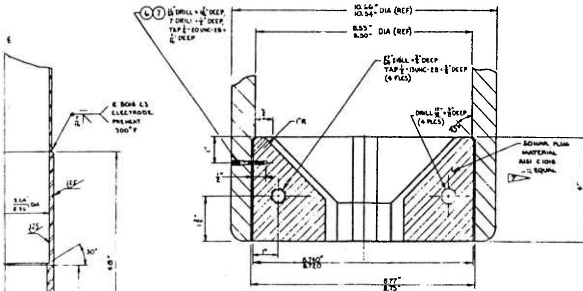
SECTION 8-B
