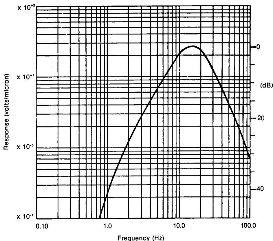
Figure 2. Displacement response of the short-period channels of the MSS.
