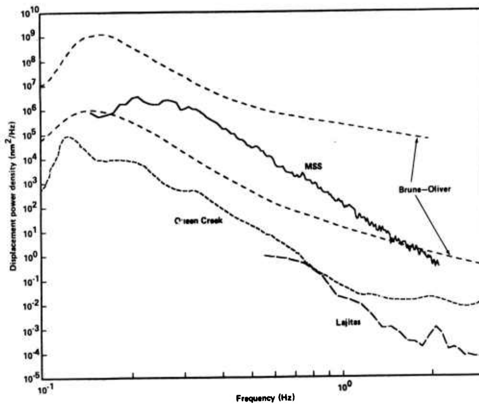
Figure 15. Comparison of the sub-bottom noise spectrum at Site 395 with spectra at two quiet continental sites. The Queen Creek, Arizona curve was taken from Melton (1976), who extracted it from Fix (1972). The Lajitas, Texas data were recorded at an extremely quiet surface site during a time of low winds (Herrin, 1982). Brune-Oliver (1959) curves are from Melton (1976).
