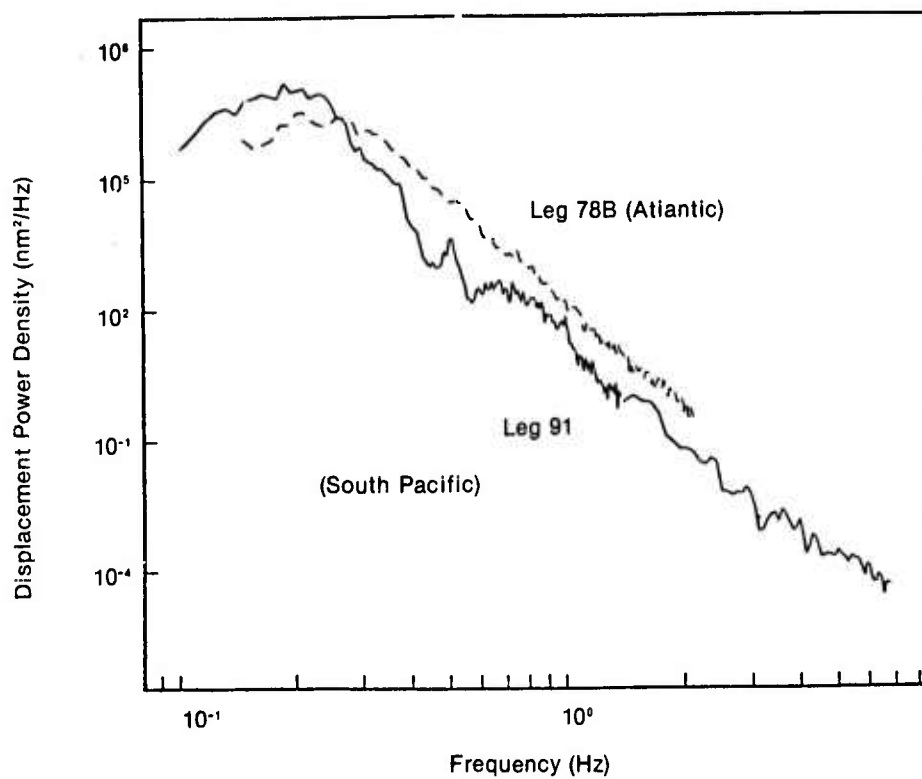
Figure 22. Comparison of MSS vertical-component spectra from DSDP Leg 78B (mid-Atlantic) and DSDP Leg 91.
