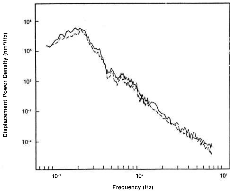
Figure 20. Similarity of MSS vertical and horizontal (X-sensor) noise levels.
