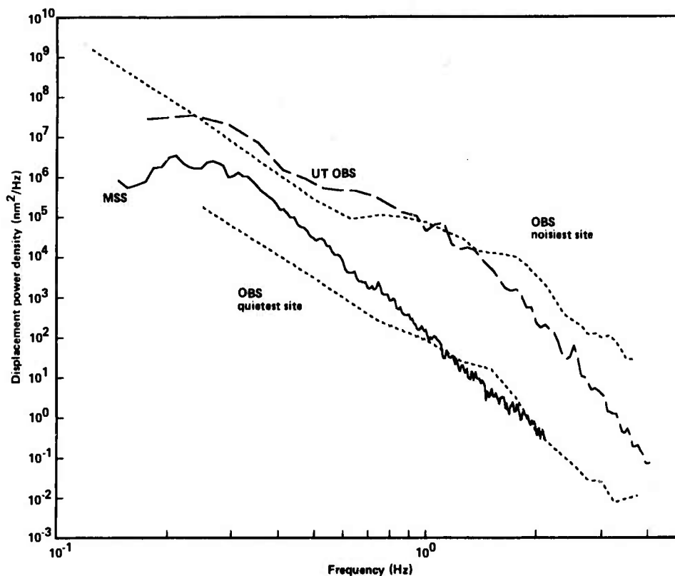
Figure 14. Comparison of Leg 78B noise spectra with OBS observations in the Pacific. The UT OBS data are the same as those in Figure 12; the MSS data are the earliest (and therefore lowest) of those in Figure 10. The two dashed curves are extrema of observations made with the Scripps Institution of Oceanography OBSs. The "noisiest site" was southeast of Hawaii, and the data were fifty-four 8-s samples; the "quietest site" was on the East Pacific Rise, and the data were thirty-one 4-s samples.
