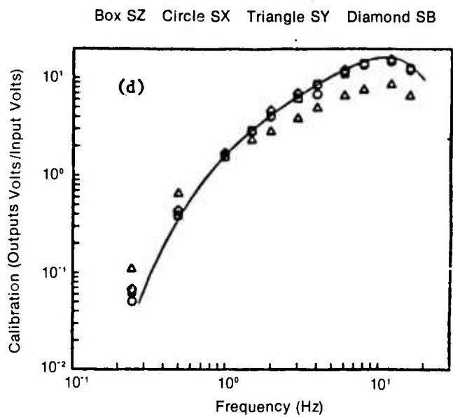
Figure 11. Teledyne calibrations of properly functioning channels.
