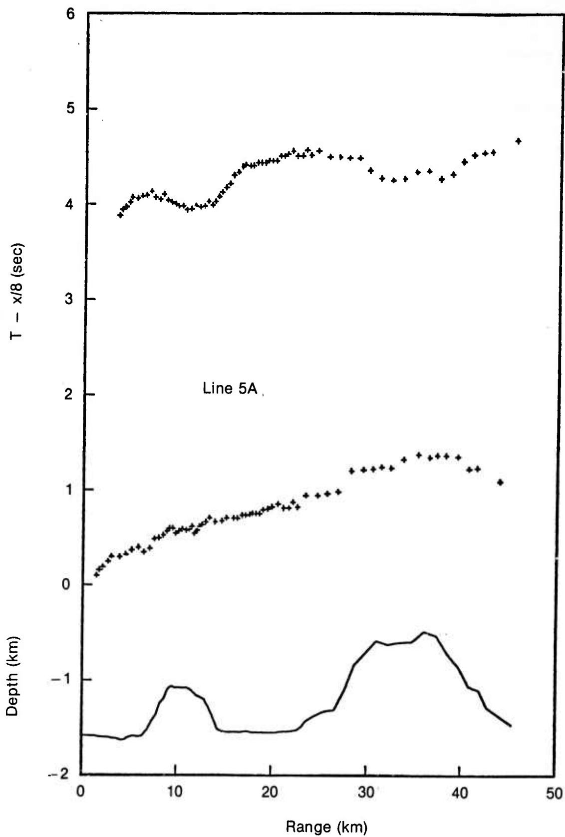
Figure 3 (b). First arrival picks (reduced to 8 \text{ km sec}^{-1} ) before and after application of the water-path and dt/dh corrections (upper and lower curves, respectively) plotted above bathymetry along each profile (Line 5).
