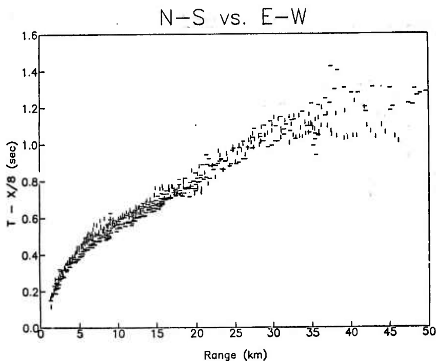
Figure 17(a). P -wave travel-times for shots at azimuths along a N-S line (shown as vertical bars) compared to shots at azimuths along an E-W line (shown as horizontal bars). Between about 5 and 15 km the E-W arrivals are early, while at ranges greater than 35 km, the N-S arrivals are early.
