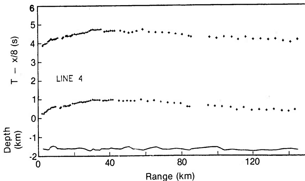
Figure 3 (a). First arrival picks (reduced to 8 km sec -1 ) before and after application of the water-path and dt/dh correction (upper and lower curves, respectively) plotted above bathymetry along each profile (Line 4).
