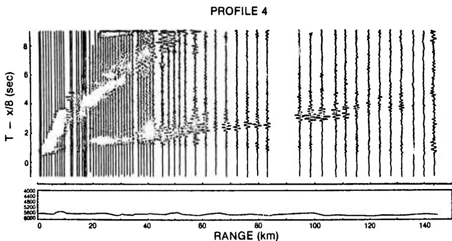
Figure 4 (a). Unfiltered record-sections (reduced to 8 \text{ km sec}^{-1} ) after application of the water-path and dt/dh corrections. Selected traces are from a short-period vertical seismometer (Line 4).
