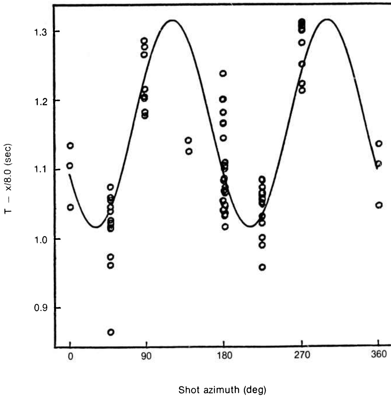
Figure 21. Travel-time vs. shot azimuth for shots at ranges between 35 and 50 km. Times have been reduced at 8 km/sec. Arrivals from rays entering the sea floor at depths shallower than 5200 m have been eliminated. Curve is least squares fit for function of form
