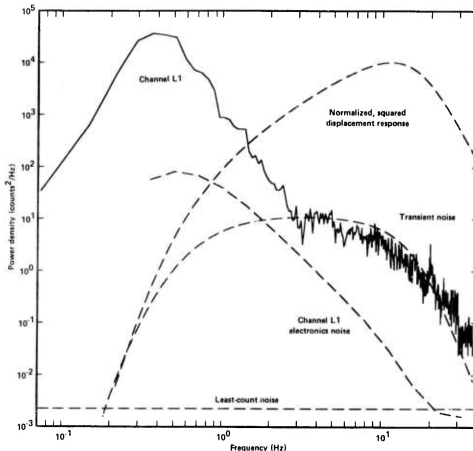
Figure 6. Power spectral densities of MSS data compared with estimates of instrument noise. The data (solid line) were computed from eight 13.65-s samples from channel L1, with no instrument correction applied. The electronics noise was estimated from RMS power values of \frac{1}{2} -octave bandwidth provided by Teledyne Geotech. The least-count noise level is that expected from uniformly distributed errors owing to the representation of a continuous quantity by a finite digital word. The transient-noise spectrum, which is attributed to the frequent, impulsive features identified in Figure 5, was computed from equation A24 (see Appendix), and defines the high-frequency limit of reliable microseismic noise estimates. Also shown in this figure is the squared, normalized MSS displacement response.
