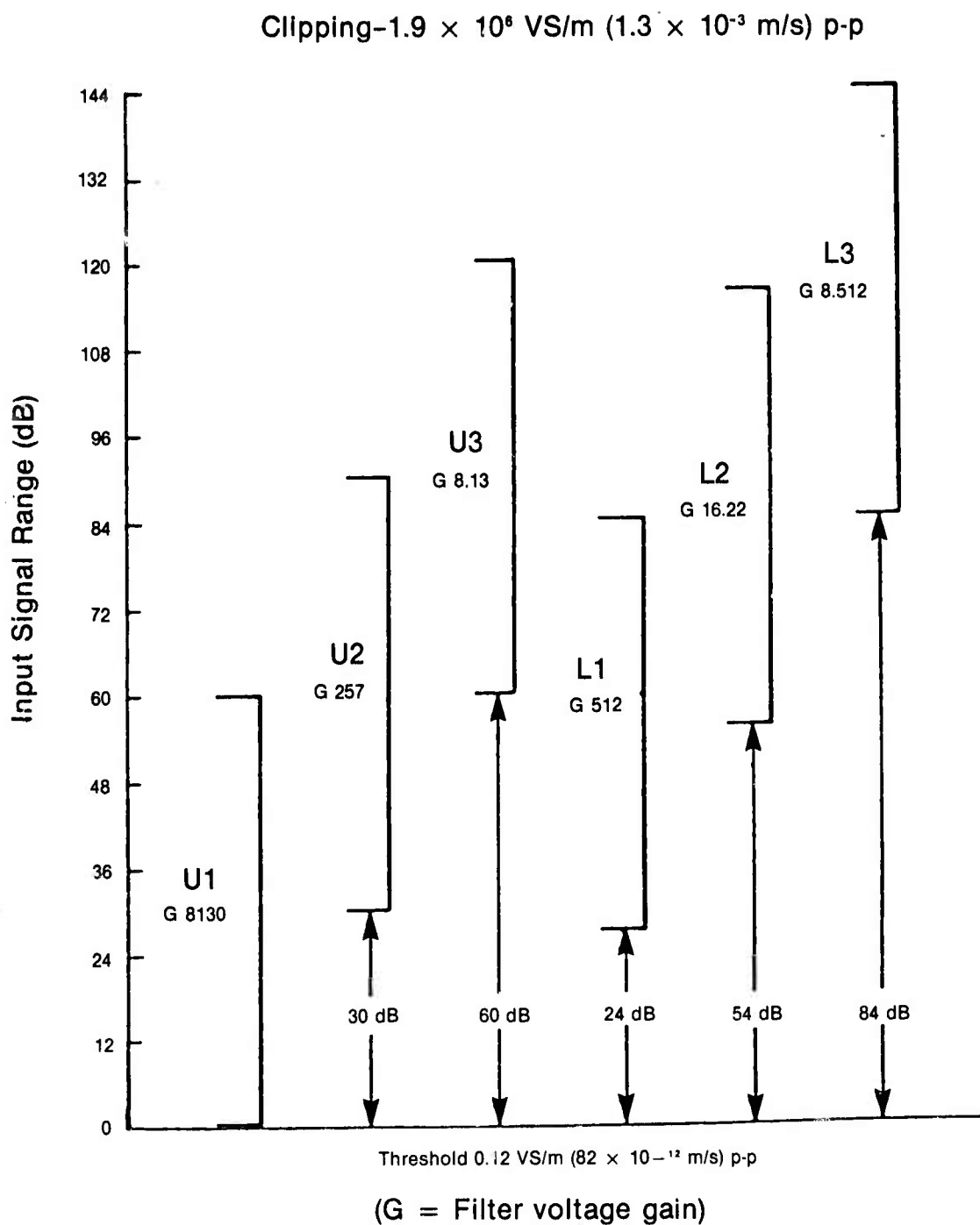
Figure 7. Dynamic gain ranging format used for BIP. L and U designations refer to lower and upper seismometer positions in the BIP.
