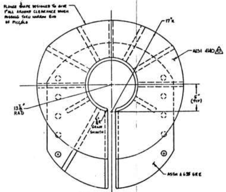
SECTION 4-D
