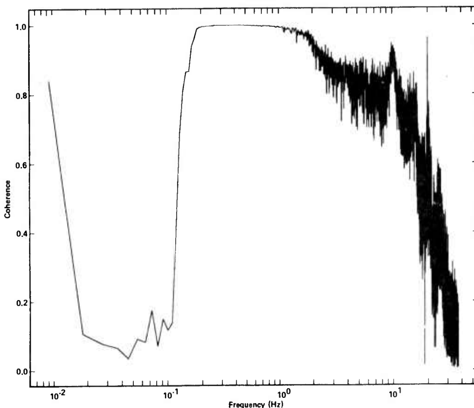
Figure 7. Coherence between the highest-usable-gain channels of each of the MSS seismometers (L1 and U2). The coherence spectrum was computed from twenty-four 109.2-s samples from each channel. The energy is highly incoherent below 0.16 Hz, where response roll-off causes instrument noise to dominate.
