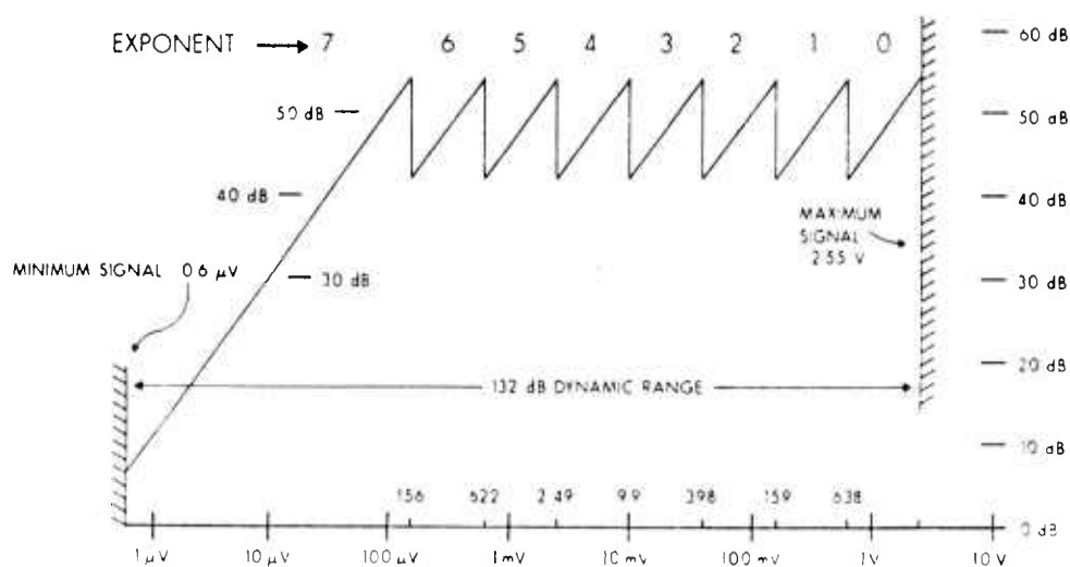
FIGURE 9. Signal amplitude vs. digital signal-to-noise ratio. A 12-bit floating point word with a 3-bit (base 4) exponent and a 9-bit mantissa is used. This is equivalent in total dynamic range to 132 dB with resolution of better than 1% of the signal amplitude.
