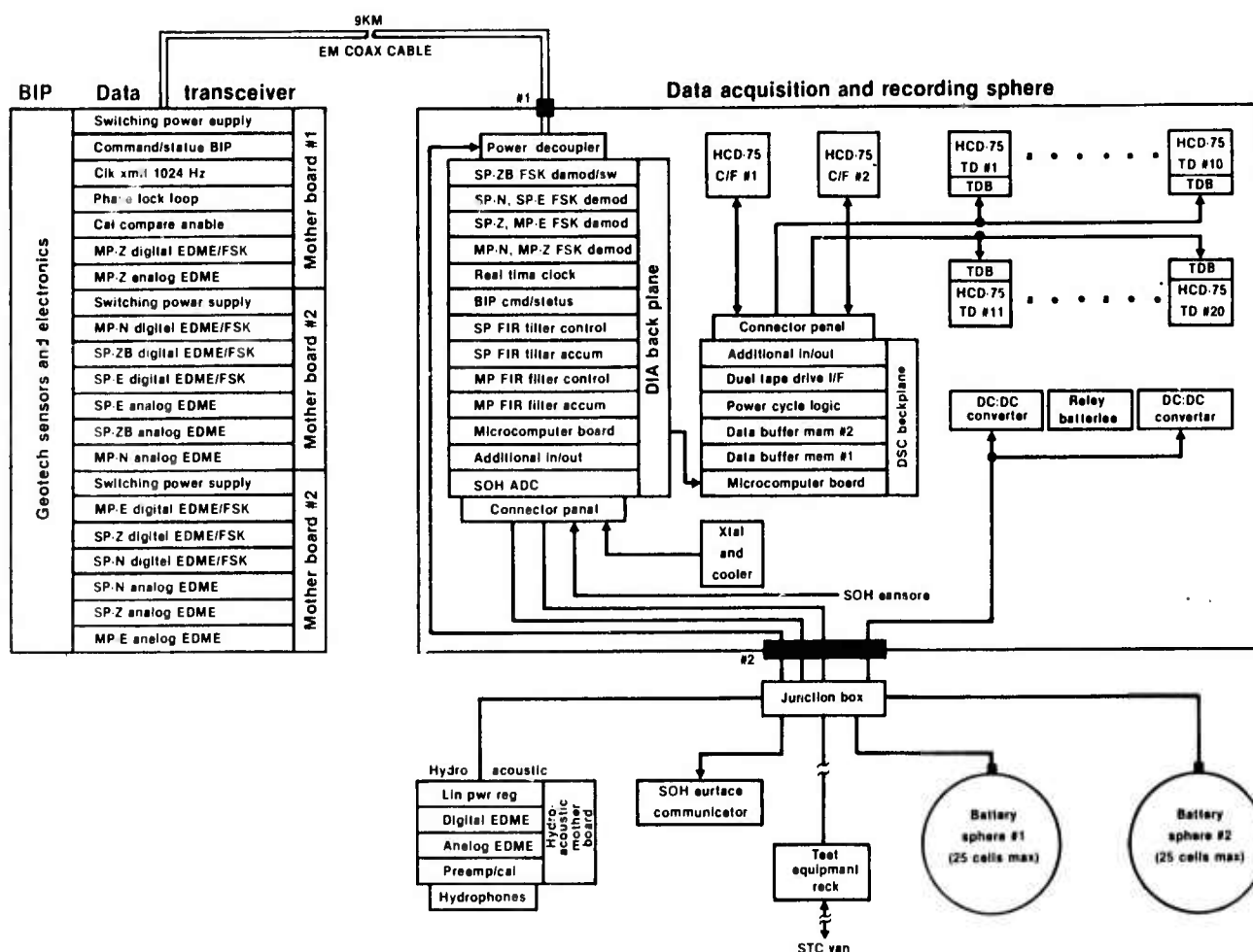
Figure 14. Diagram of BPP and DARS components.
