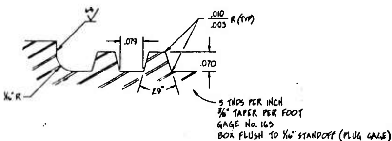
DETAIL 4-B N.T.S. (FROM VIEW 4-C)
