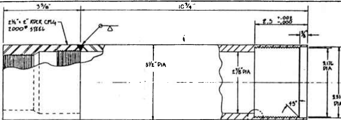
DETAIL 4-C SONAR SINKER BAR COUPLING SUB N.T.S. (FROM VIEW 3-A)
