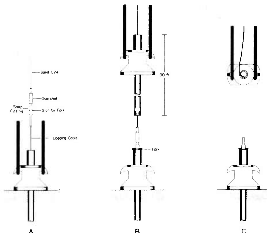
FIGURE 13. Pipe stripping. When the borehole package is in place, the drill pipe is stripped from around the cable as discussed in the text.
