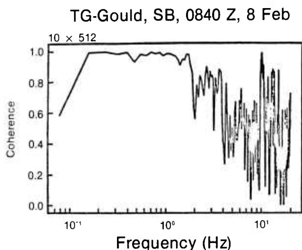
Figure 13. Decline of SB data stream coherence at high frequencies due to ship generated noise. (SB, 0840Z, 8 Feb.).
