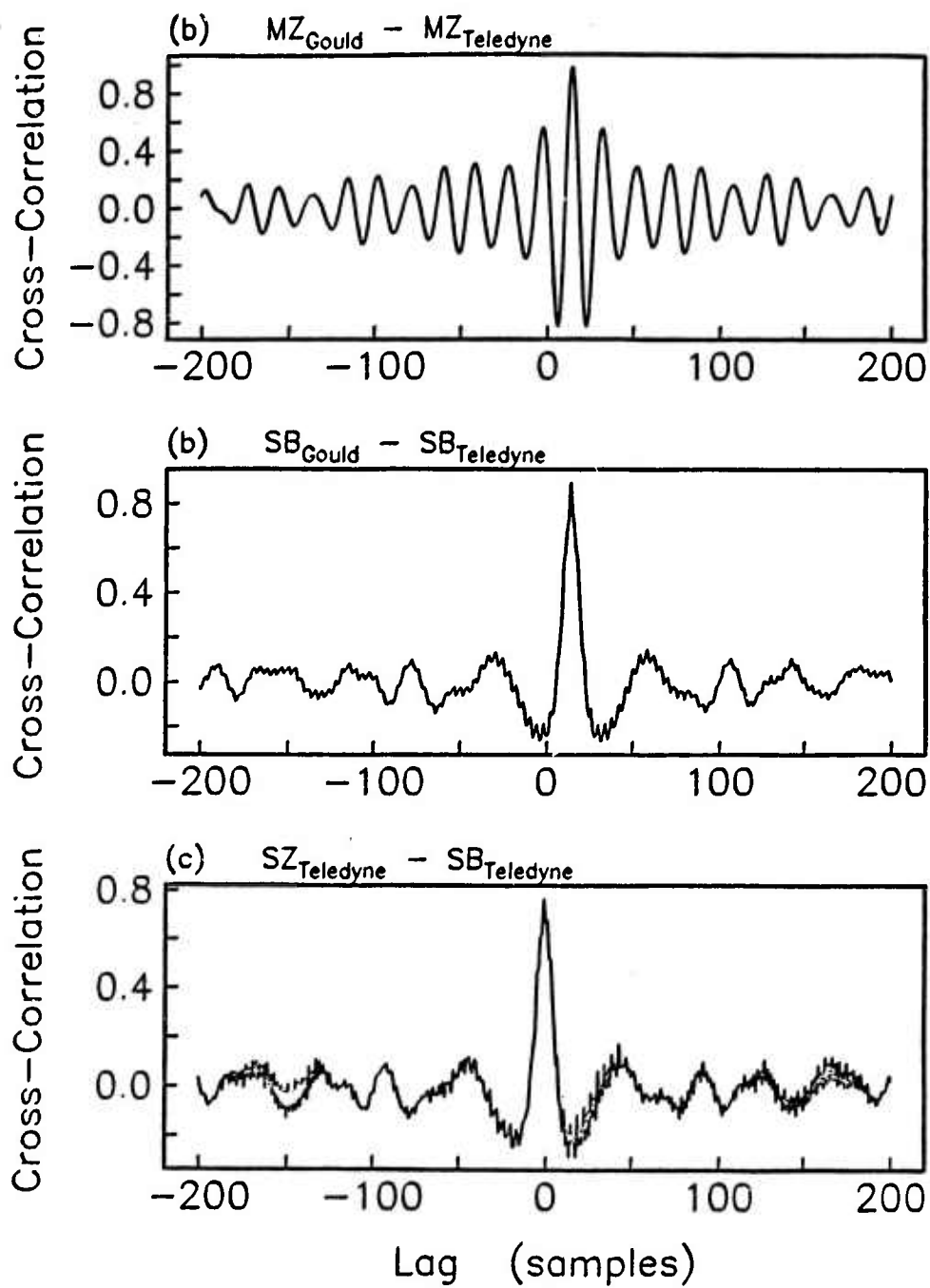
Figure 10. Relative amplitudes and timing between Gould and Teledyne recording systems with cross-correlations and linear regressions of corresponding channels.
