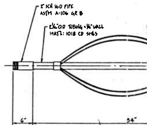
DETAIL 3-B SONAR CENTERING SPRING SCALE: 1 1/2\" = 1'-0\" (FROM VIEW 3-A)
