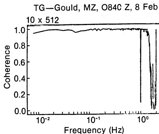
Figure 15. Mid-period coherence, SB data stream, (0840Z, 8 Feb.).
