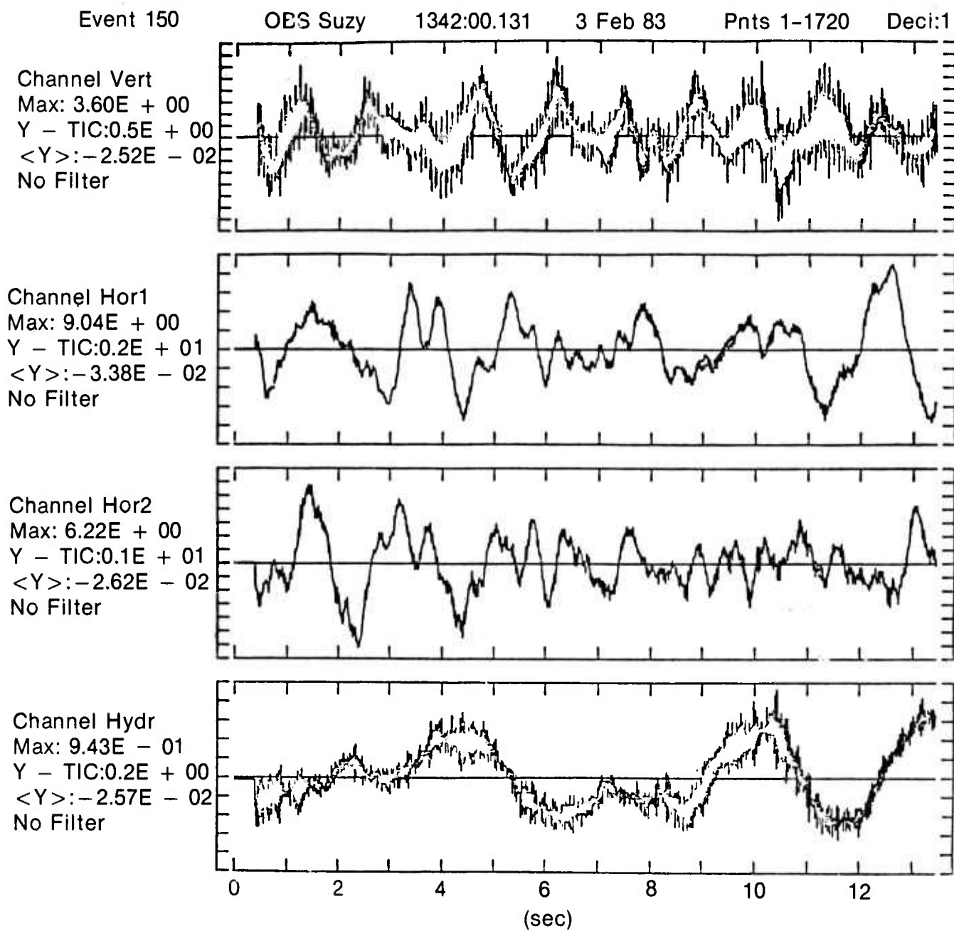
Figure 16. Typical 4-channel OBS noise data (OBS Suzy, event 150, 1342:00.131, 3 Feb., pnts 1-1720).
