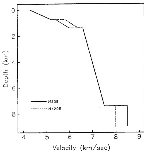
Figure 22. Anisotropic velocity vs. depth model which satisfies the Ngendei travel-time data. Solid line is velocity model at N30°E azimuth; dashed line is at N120°E azimuth.
