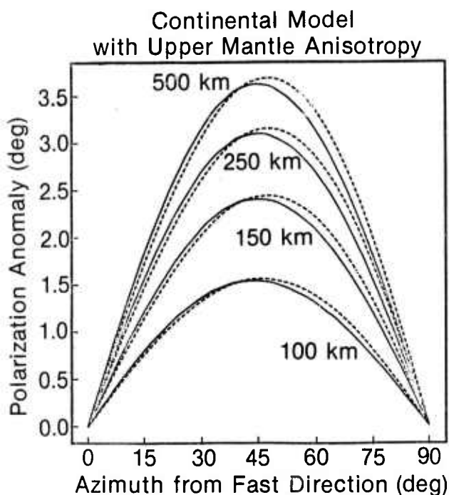
Figure 11. Calculated polarization anomalies for a continental model with 30 km of 6 km/sec crust above an anisotropic upper mantle with a 20 velocity variation from 8.0 to 8.6 m/sec. Solid lines were calculated from the slowness surfaces for the exact model. Dashed lines were calculated using a least time algorithm on an approximate group velocity function.
