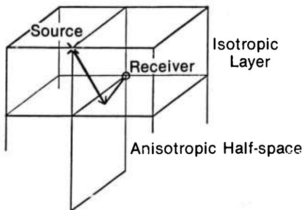
Figure 4. Ray path for a head-wave traveling on an anisotropic half-space generated by a point source in an overlying isotropic layer. The ray path skews to the side, out of the vertical plane connecting source and receiver. The azimuth of the ray at the receiver will differ from the source-receiver azimuth.
