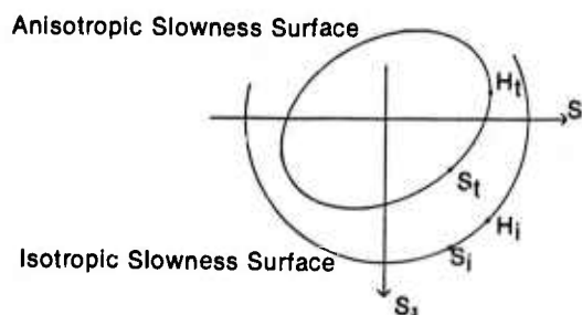
Figure 5(b). Slowness surface representation for p-waves of the isotropic and anisotropic layers. The outer, spherical slowness surface represents the isotropic layer. The inner slowness surface represents the anisotropic layer. Notice that in this example the anisotropic medium has smaller slowness in every direction, or in other words, is faster in every direction. S_i represents the downgoing incident p wave. S_t represents the downgoing transmitted p-wave. The horizontal slowness S_1 is conserved. The head-wave which would propagate in the S_1 direction is given by H_t . H_i corresponds to the incident wave which would generate the head-wave.
