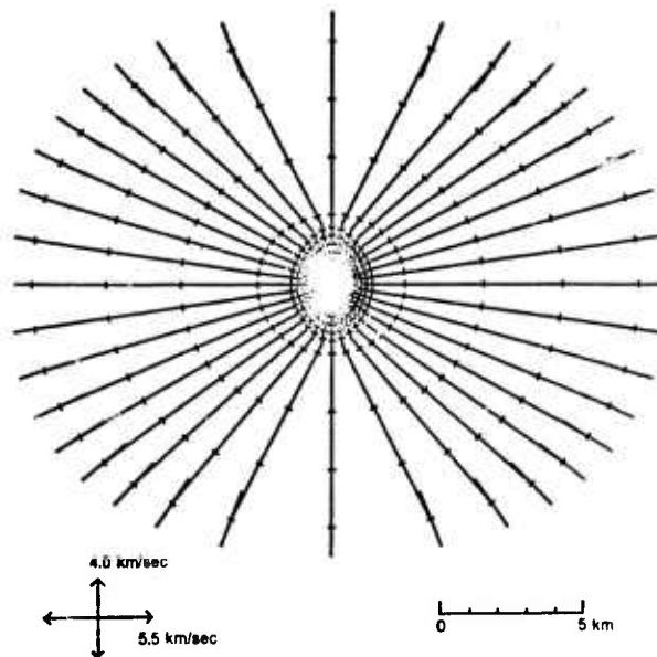
Figure 6(b). Map view of Figure 6a as seen from a point directly above the source. Ray paths turn toward the fast direction in the anisotropic half-space.
