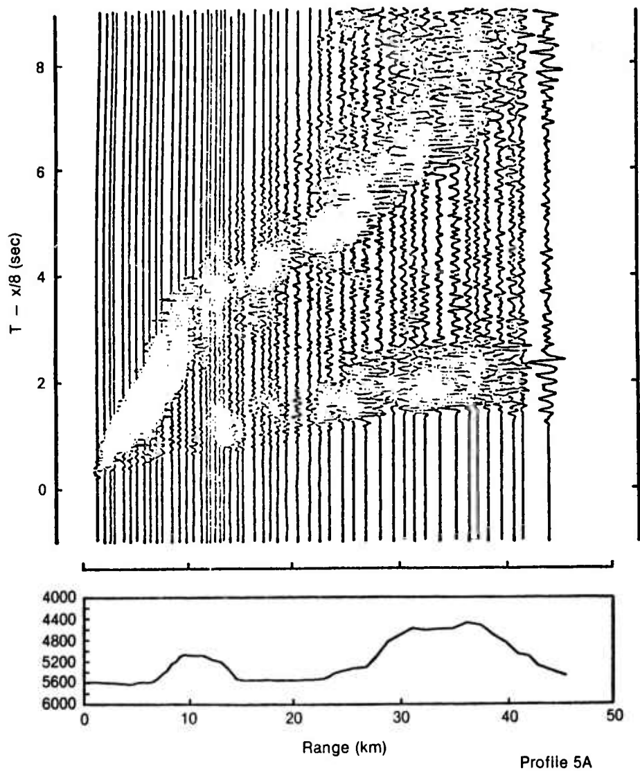
Figure 4 (b). Unfiltered record sections (reduced to 8 \text{ km sec}^{-1} ) after application of the water-path and dt/db corrections. Selected traces are from a short-period vertical seismometer (Line 5a).
