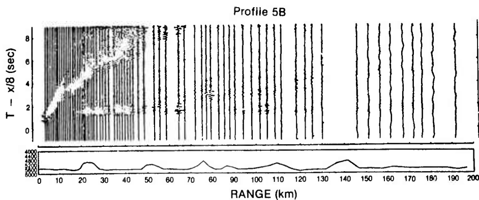
Figure 4 (c). Unfiltered record sections (reduced to 8 \text{ km sec}^{-1} ) after application of the water-path and dt/db corrections. Selected traces are from a short-period vertical seismometer (Line 5b).
