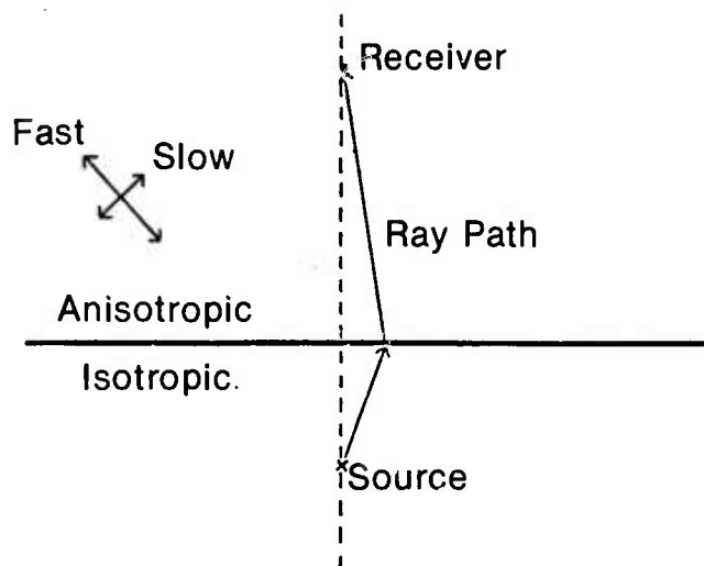
Figure 3. Ray path between a source in an isotropic medium and a receiver in an anisotropic medium. Both source and receiver are along a line perpendicular to the interface. The ray path skews to the side, so that the ray path within the anisotropic medium is rotated toward the fast direction.
