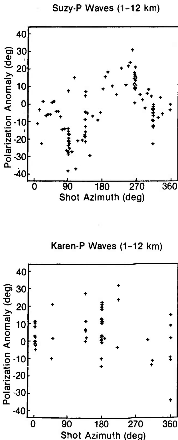
Figure 26. P-wave polarization anomalies for OBS a) Suzy and b) Karen at ranges (corrected to sea floor) of 1 to 12 km. Note the large scatter in the data.
