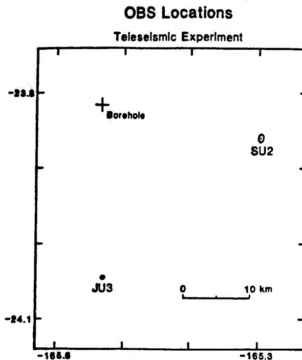
Figure 3(a). Ocean bottom seismometer locations for teleseismic experiment (Suzy-2 and Juan-3).
