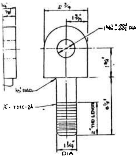
DETAIL 3-D EYE BOLT (2 REQ'D)
