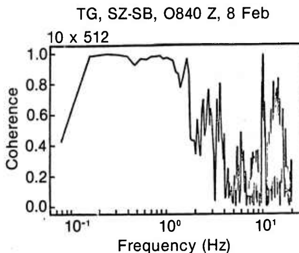
Figure 14. Coherence between SB and SZ Teledyne data streams (0840Z 8 Feb.).
