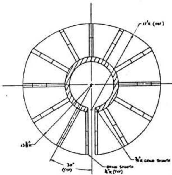
SECTION 6-D
