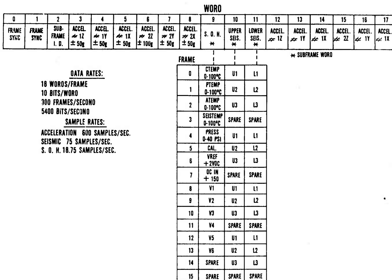
Figure 9. MSS PCM data format.
