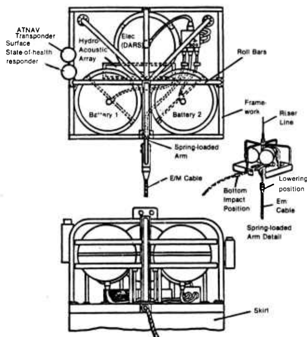
Figure 13. BPP configuration.
