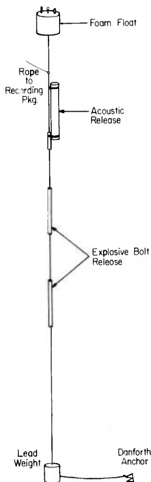
FIGURE 7. Float-anchor assembly. The anchor is released from the float and recovery rope either at a specific time (explosive bolt release) or on command (acoustic release), allowing the float and recovery rope to return to the surface.
