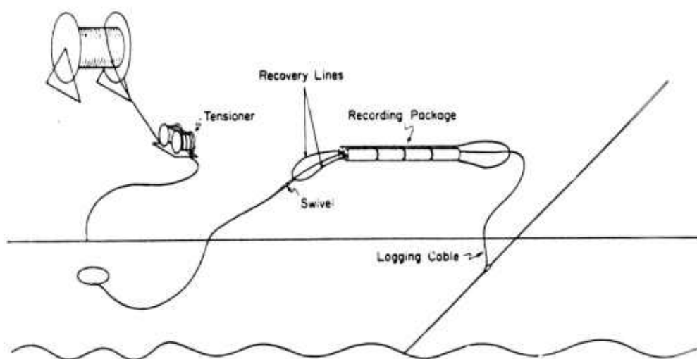
FIGURE 14. Deployment of recording package.
