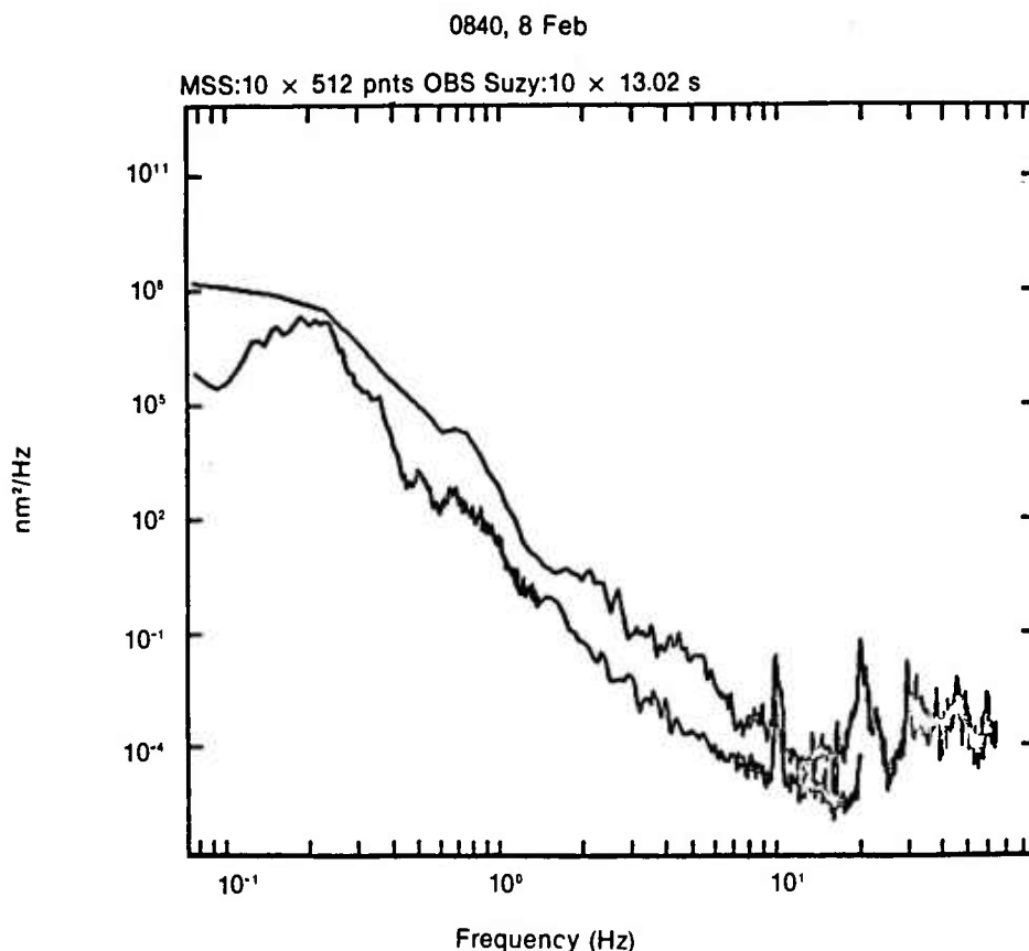
Figure 18. Comparison of MSS and OBS vertical component spectra. MSS levels are about 15 dB lower than OBS levels above 0.3 Hz. (MSS: 10 x 512 pnts, OBS Suzy: 10 x 13.02 x, 0840Z, 8 Feb.).
