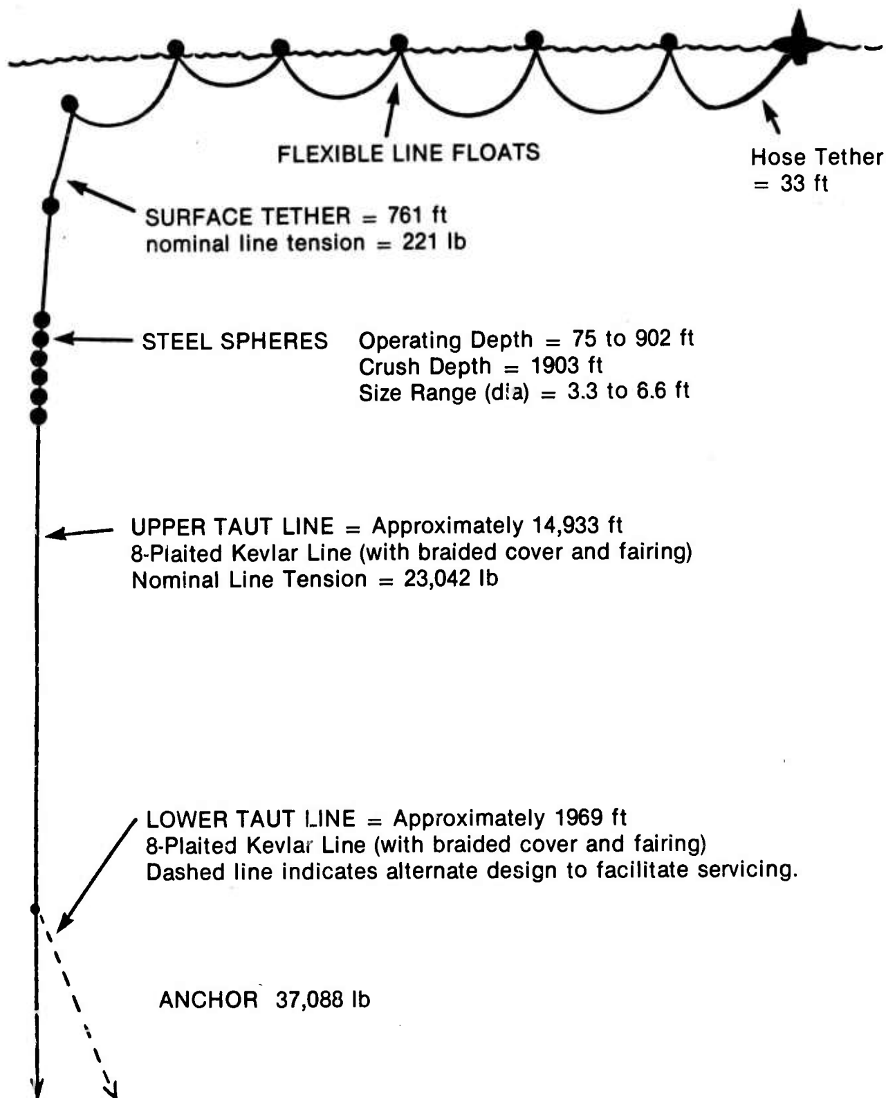
Figure 23. Mooring configuration for MSS satellite telemetry buoy.
