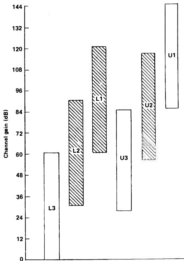
Figure 2. Schematic depiction of the MSS-data channel gains. The outputs of the two vertical-component seismometers, one configured 50 cm below the other, were split into 3 channels each, and the gains of the resultant 6 channels were staggered to yield 144 dB of dynamic range. "U" and "L" refer to the upper and lower seismometers, respectively. The use of a 10-bit unsigned digital word resulted in a range of 60 dB for each channel. Adjacent channels of a seismometer overlapped by 30 dB; the upper seismometer gains were offset from the lower seismometer gains by 24 dB. Because of noise and clipping, only the data from channels L1, L2, and U2 could be used in this study.
