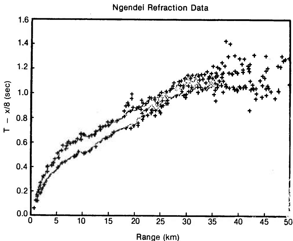
Figure 16. P-wave picks (totaling 1005) from the Ngendei refraction shooting. Topographic time and range corrections have been made and the travel-times reduced at 8 km/sec.
