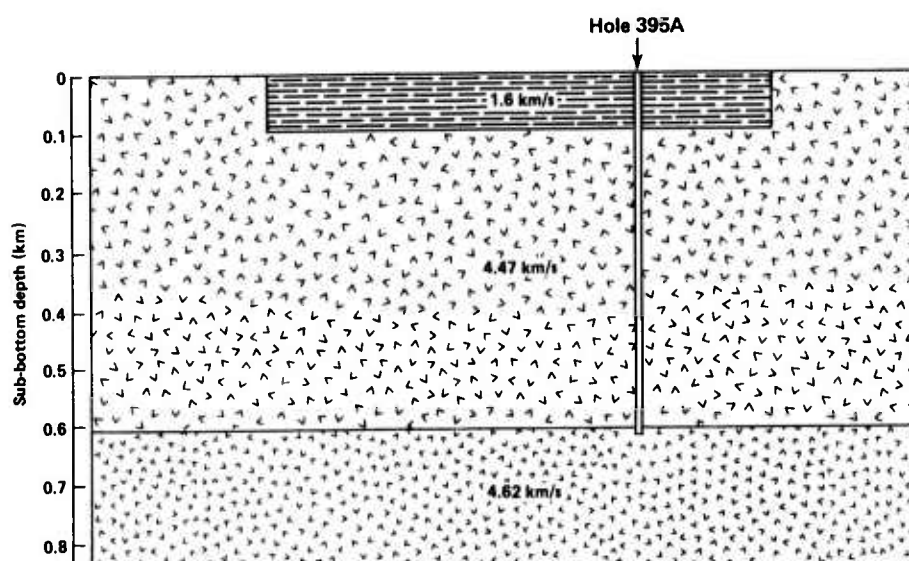
Figure 6. Model of upper crustal velocity structure immediate surrounding DSDP Hole 395A, as deduced from the seismic refraction data. Velocities not corrected for dip.
