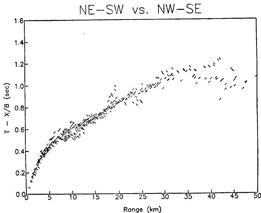
Figure 17(b). NE-SW shots (shown as diagonals to upper right) vs. NW-SE shots (shown as diagonals to lower right). NW-SE arrivals are early between about 6 and 17 km, while NE-SW arrivals are early at ranges greater than 35 km.
