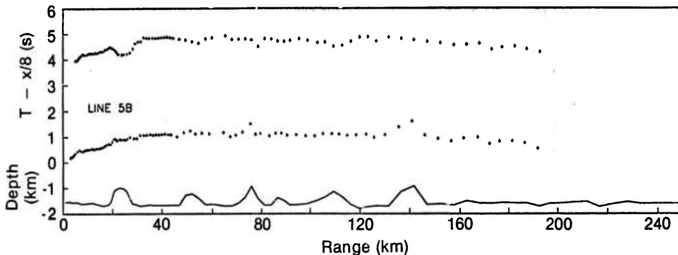
Figure 3 (c). First arrival picks (reduced to 8 \text{ km sec}^{-1} ) before and after application of the water-path and dt/dh corrections (upper and lower curves, respectively) plotted above bathymetry along each profile (Line 5b).
