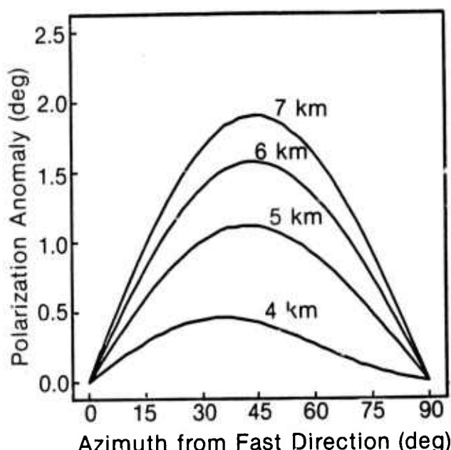
Figure 24. Predicted p -wave polarization anomalies for a simplified Ngendei model. Ranges are from source to receiver; equivalent ranges corrected to the sea floor are about 1.5 km closer. Positive anomalies represent deviations away from the fast direction in the anisotropy.
