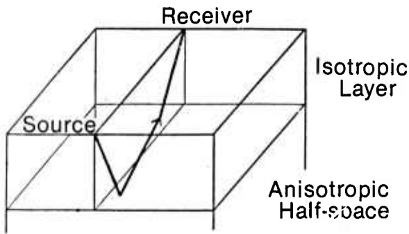
Figure 9. Ray path for a source and receiver on an isotropic layer above an anisotropic half-space. The ray path is skewed, and the ray at the receiver will be at an angle to the vertical plane connecting source and receiver.
