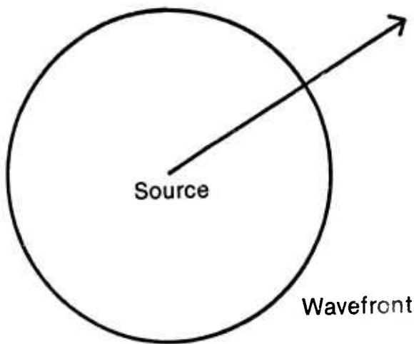
Figure 1. Wavefront from point source in homogeneous, isotropic medium. Group velocity vector is also direction of phase velocity and particle motion for p-waves.
