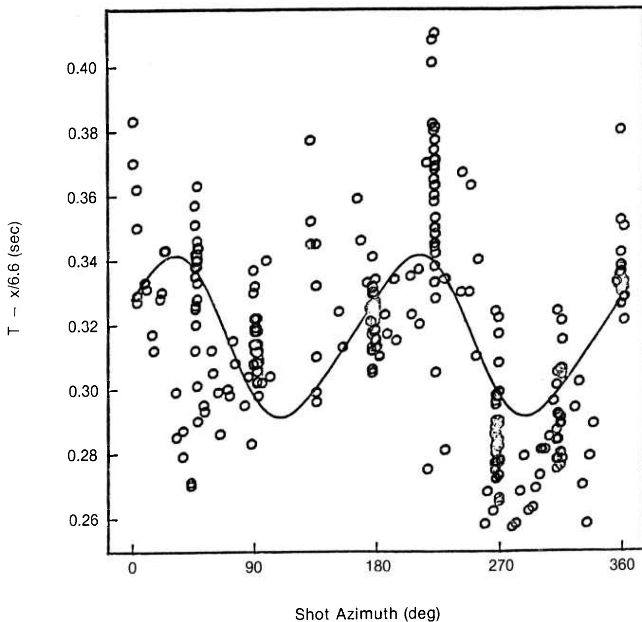
Figure 20. Travel times vs. shot azimuth for shots at ranges of 7 to 11 km. All times have been reduced at 6.6 km/sec. Arrivals from rays entering the sea floor at depths shallower than 5400 m have been eliminated. Curve is least squares fit for a function of the form
