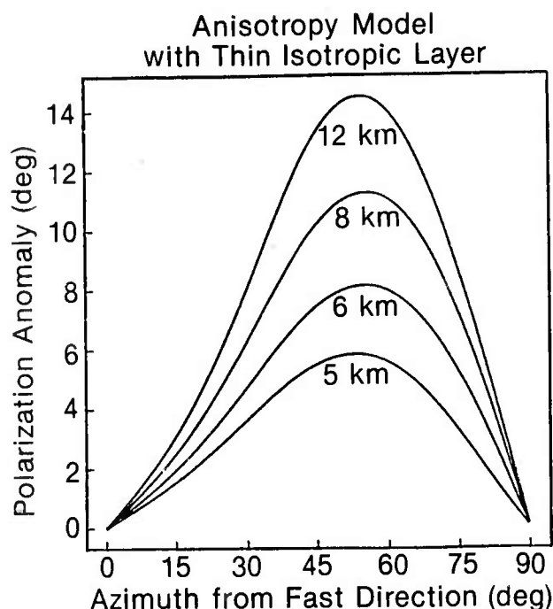
Figure 13. Calculated polarization anomalies for a model of the oceanic crust involving a 1-km thick, 3-km/sec isotropic layer above the Stephen model of an anisotropic half-space. Anomalies are shown at source-receiver ranges of 5, 6, 8, and 12 km. Positive anomalies represent deviations away from the fast direction in the anisotropic half-space.
