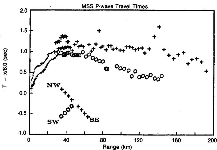
Figure 18. P-wave travel-times as recorded by the MSS. Circles represent shots along a SW line, while crosses represent shots along a NW-SE line. Note the difference in upper mantle velocity.
