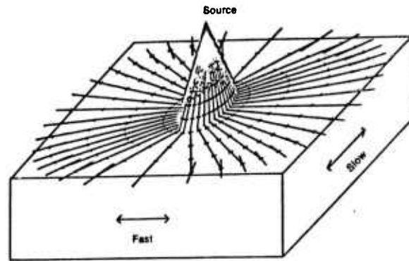
Figure 6(a). Schematic representation of ray paths for the Stephen anisotropy model. Near vertical lines leaving the source correspond to ray paths within the ocean. Horizontal lines correspond to head-wave ray paths on the surface of the anisotropic half-space. The rays shown are at increments of 10 degrees in azimuth leaving the source. Tic marks on the rays occur at intervals of 0.5 second. Black lines at the end of the rays represent particle motion directions for each ray path shown in the anisotropic half-space.
