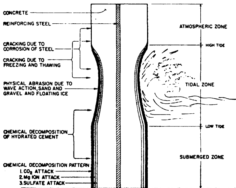
FIGURE 4.13. DETERIORATION OF A CONCRETE STRUCTURE IN SEA WATER (FROM [4.56])
