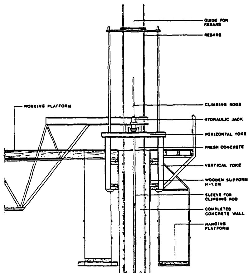
FIGURE 3.9 SLIP FORMING OF CELL WALLS (FROM [3.16])
