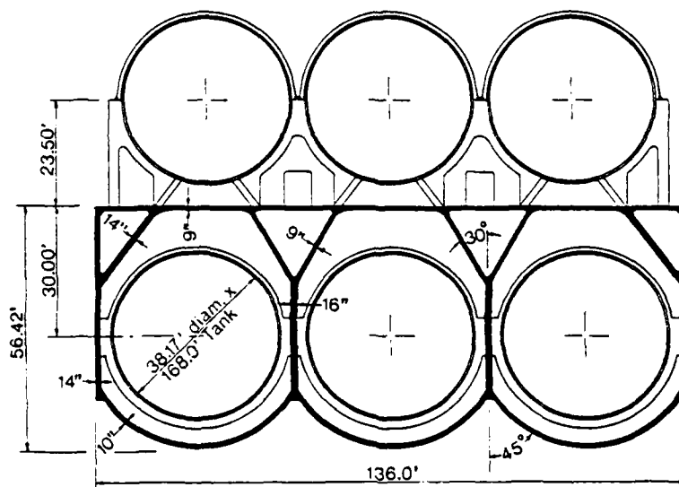
FIGURE 3.13 MIDSHIP SECTION, 65,000-TON CONCRETE LPG FACILITY (FROM [3.28])
