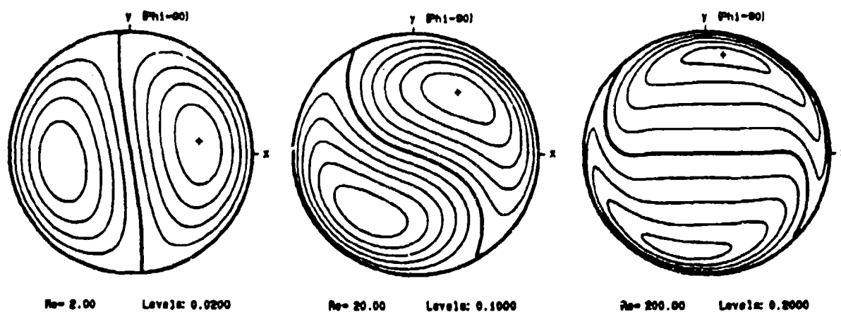
Figure 2. Contour lines of equal axial velocity, v_z/(2e) = \text{const.} , for Re=2 , 20, and 200. The difference between levels is 0.02, 0.1, and 0.2, respectively. The + marks the velocity maximum.
