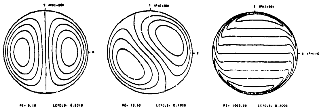
Figure 1. Contour lines of equal axial velocity, v_z/(2\pi\sigma) = \text{const.} , for Re=0.01 , 10 and 1000. The difference between levels is 0.001, 0.1 and 0.2, respectively.
