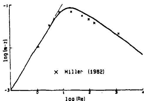
Figure 2. Comparison of the theoretical result for m , vs. Re with experimental data [1]. The straight line shows the asymptotic law m_s \approx Re/96 .
