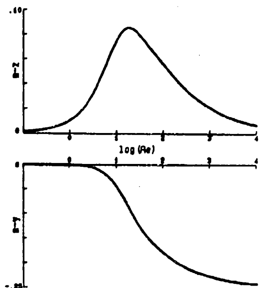
Fig. 4. The nondimensional coefficients m_z , m_y in eq. (14) versus the Reynolds number, Re .
