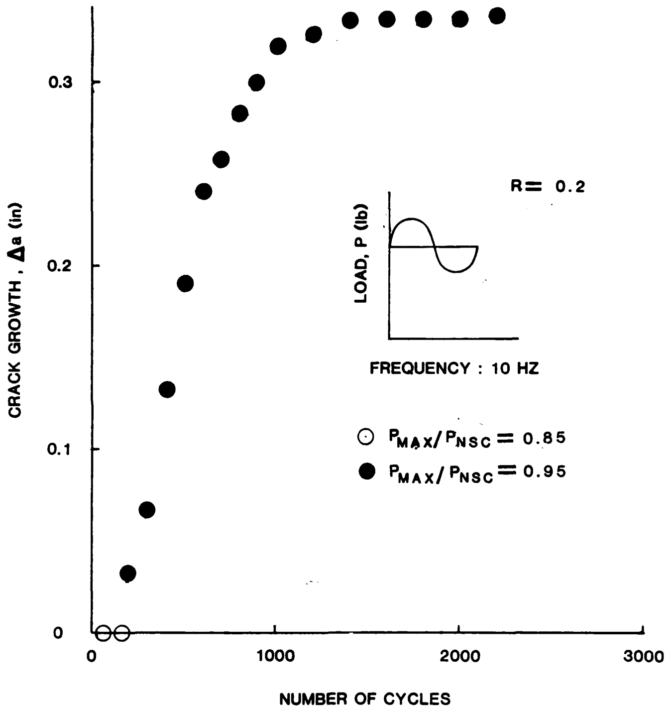
Figure 4. Tension-Tension Fatigue Crack Growth Results
